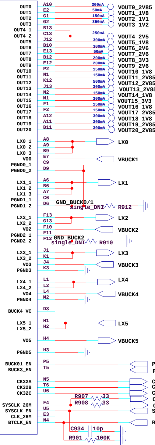
Hi6421 Power Management The type and specification of the components refer to the BOM
