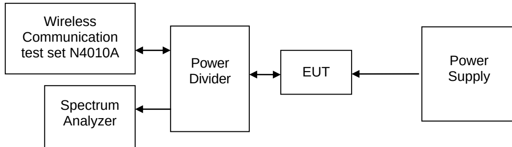
Figure 4. Test Set-up
