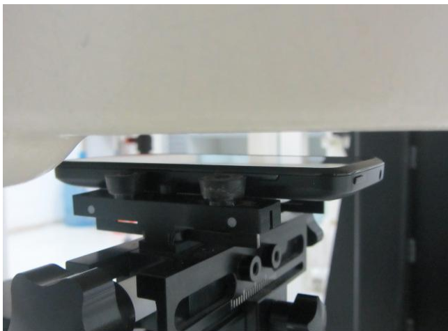
Photo 10: Left edge(10mm)
