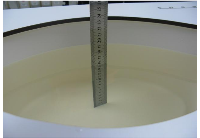
Photo 18:MSL 1800MHz depth (15.2cm)
