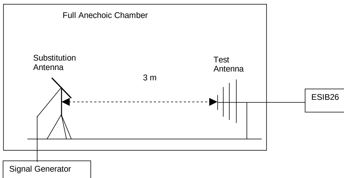
Figure 6. Test Set-up
