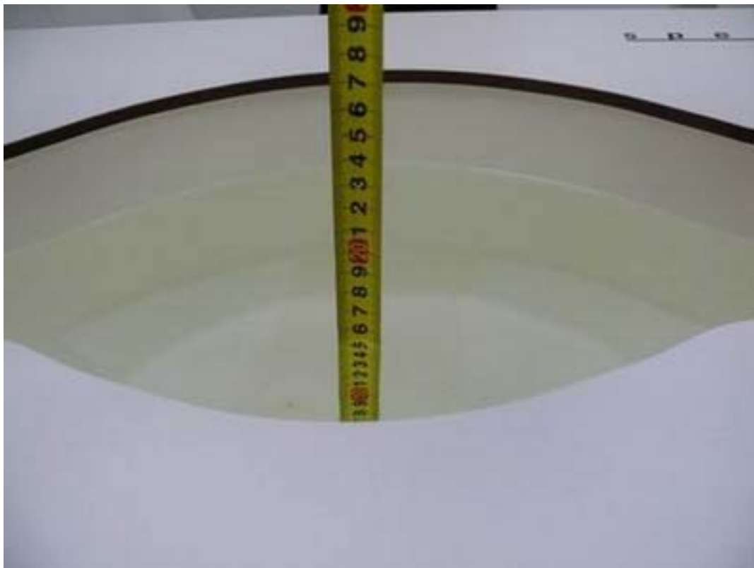
Picture 20: Liquid depth in the flat Phantom (5600 MHz, 15.3cm depth)
