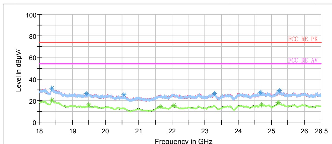
RE 18-26.5GHz PK+AV
