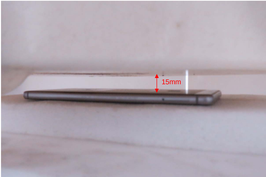
Picture 6: Back Side, the distance from handset to the bottom of the Phantom is 15mm
