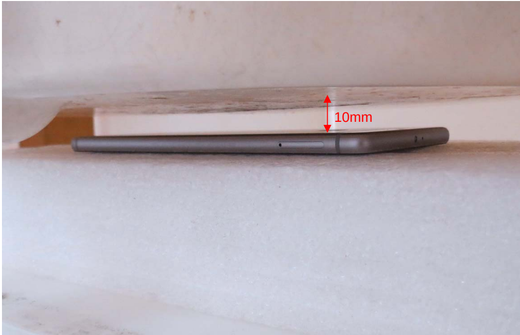
Picture 8: Back Side, the distance from handset to the bottom of the Phantom is 10mm
