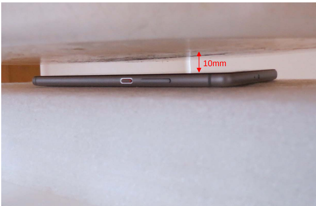
Picture 9: Front Side, the distance from handset to the bottom of the Phantom is 10mm
