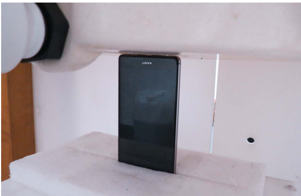
Picture 19: Bottom Side, the distance from handset to the bottom of the Phantom is 0mm
