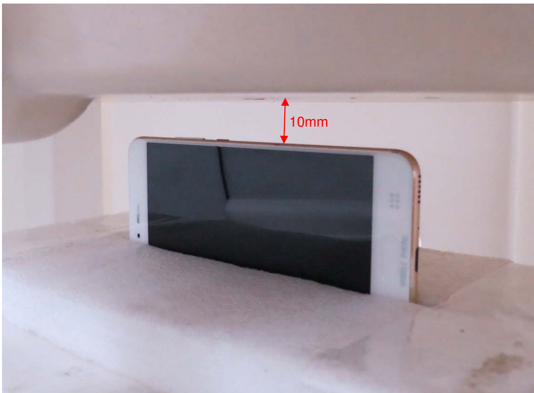
Picture 12: Right Edge, the distance from handset to the bottom of the Phantom is 10mm
