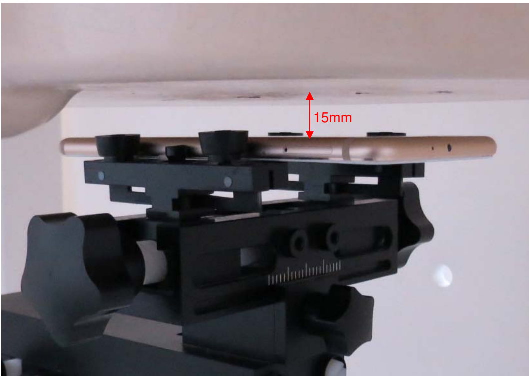
Picture 7: Back Side, the distance from handset to the bottom of the Phantom is 15mm
