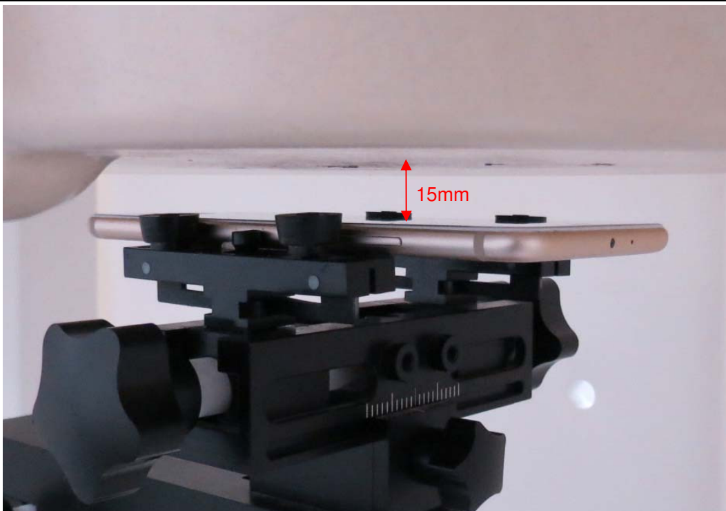
Picture 8: Front Side, the distance from handset to the bottom of the Phantom is 15mm
