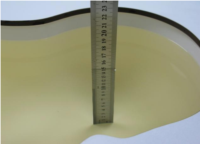
Photo 24: HSL2450MHz depth (15.0cm)
