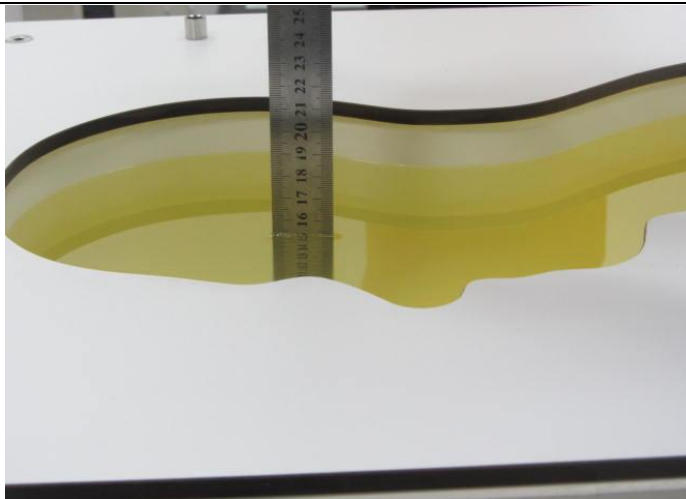
Photo 18: HSL835MHz depth (15.0cm)
