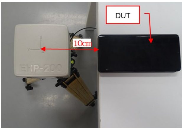
Photo 4: Bottom Side 10cm
