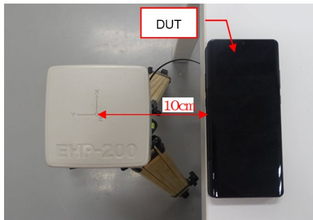
Photo 7: Front Side 10cm
