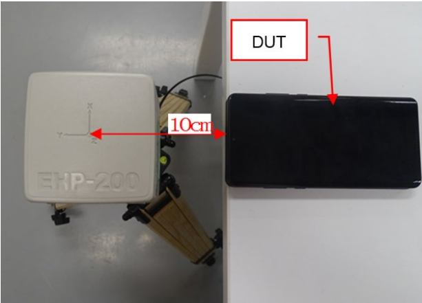
Photo 3: Top Side 10cm
