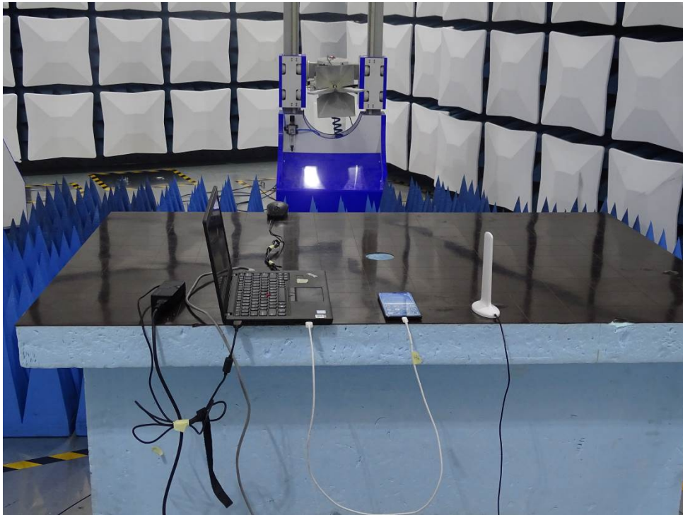
Radiated Disturbance Emissions (1GHz to 18GHz)
