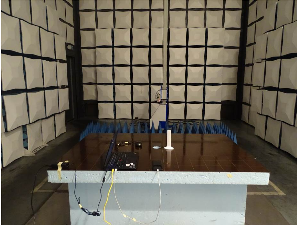
Radiated Disturbance Emissions (26.5GHz to 40GHz)
