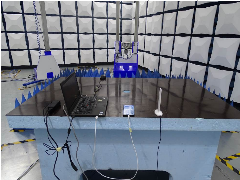
Radiated Disturbance Emissions (18GHz to 26.5GHz)
