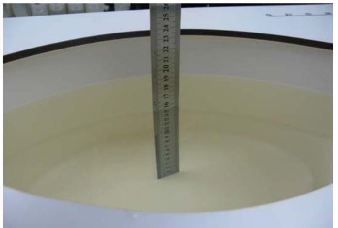
Photo 24: MSL1750MHz depth (15.1cm)
