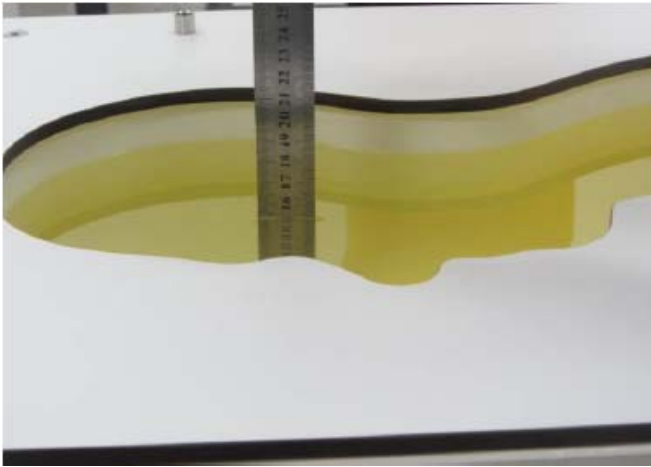
Photo 21: HSL835MHz depth (15.1cm)
