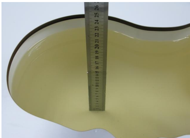
Photo 21: HSL1900MHz depth (15.0cm)
