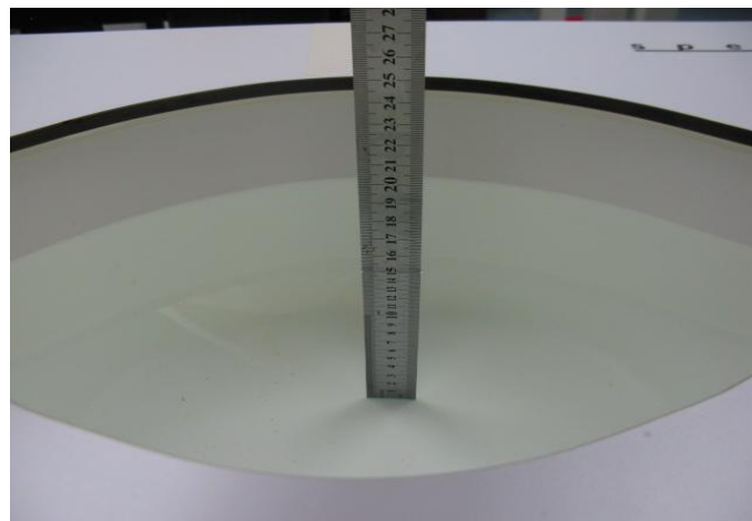
Photo 21: MSL1900MHz depth (15.1cm)
