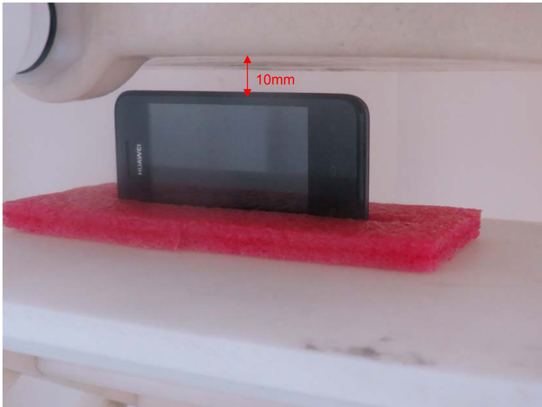
Picture 16: Right Edge, the distance from handset to the bottom of the Phantom is 10mm (Original)
