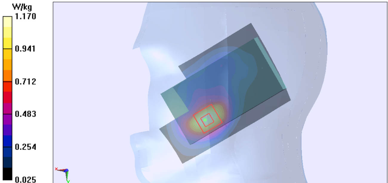
Figure Right Hand Touch Cheek UMTS Band II Channel 9538
