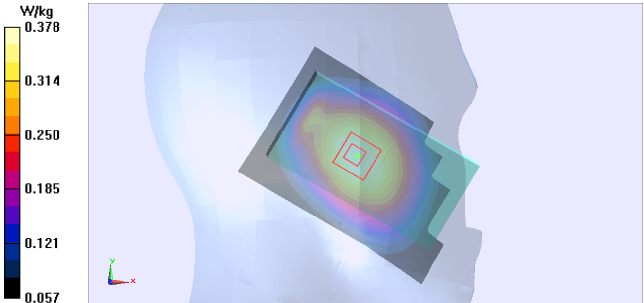
Figure Left Hand Tilt 15° UMTS Band V Channel 4183
