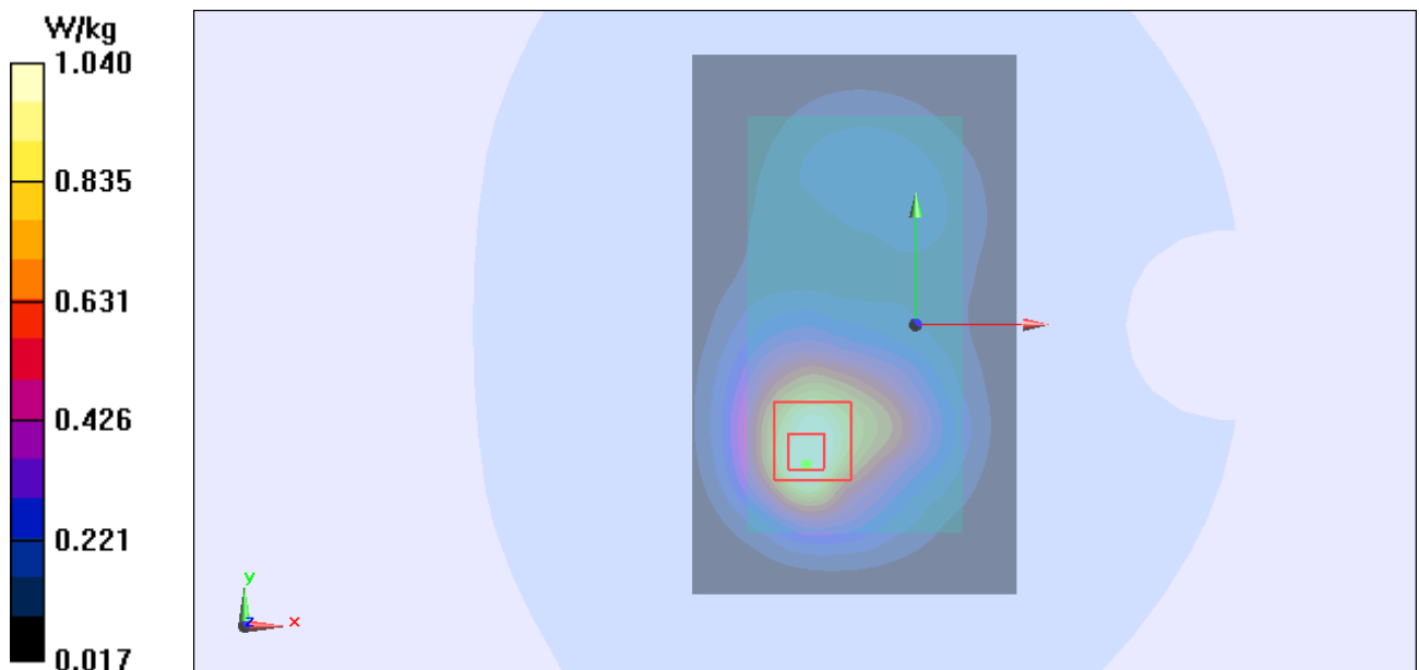
Figure Body, Back Side, GSM 1900 GPRS (4Txslots) Channel 661
