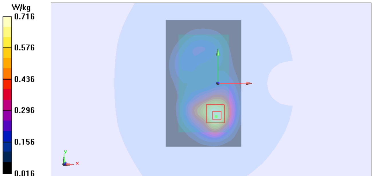
Figure Body, Front Side, GSM 1900 GPRS (4Txslots) Channel 512
