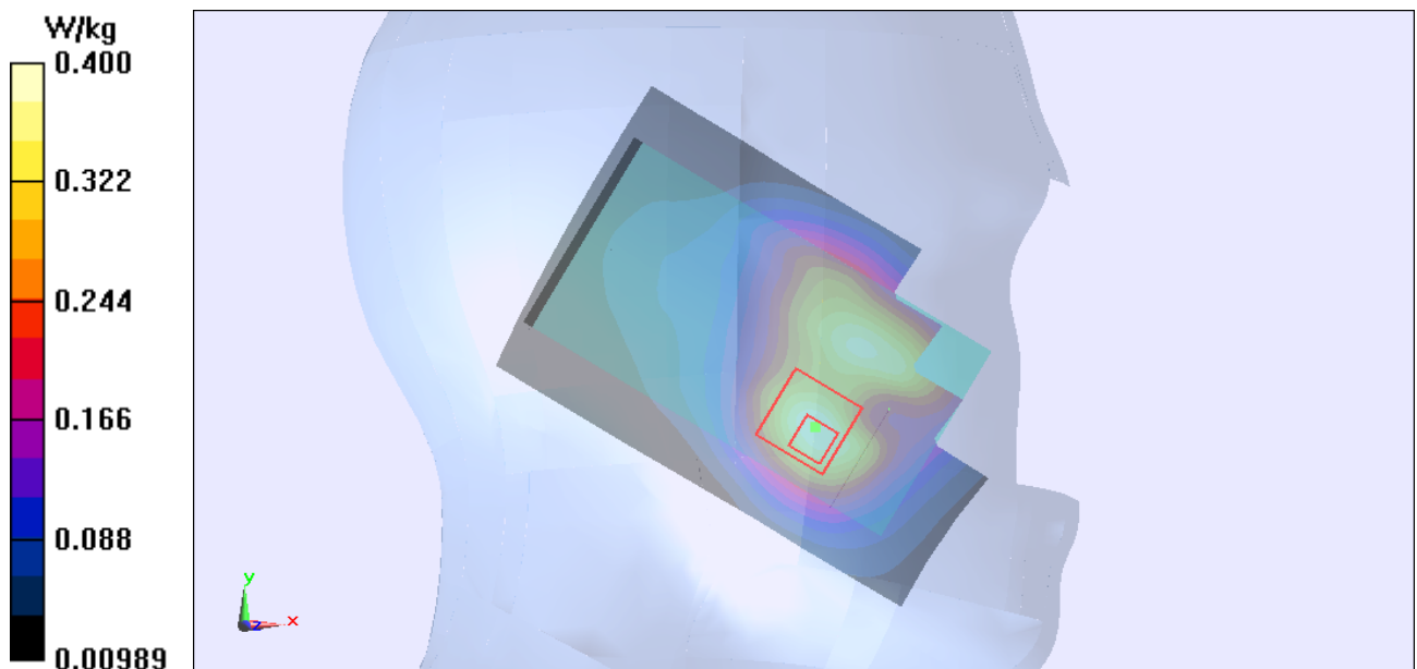
Figure Left Hand Touch Cheek GSM 1900 Channel 661
