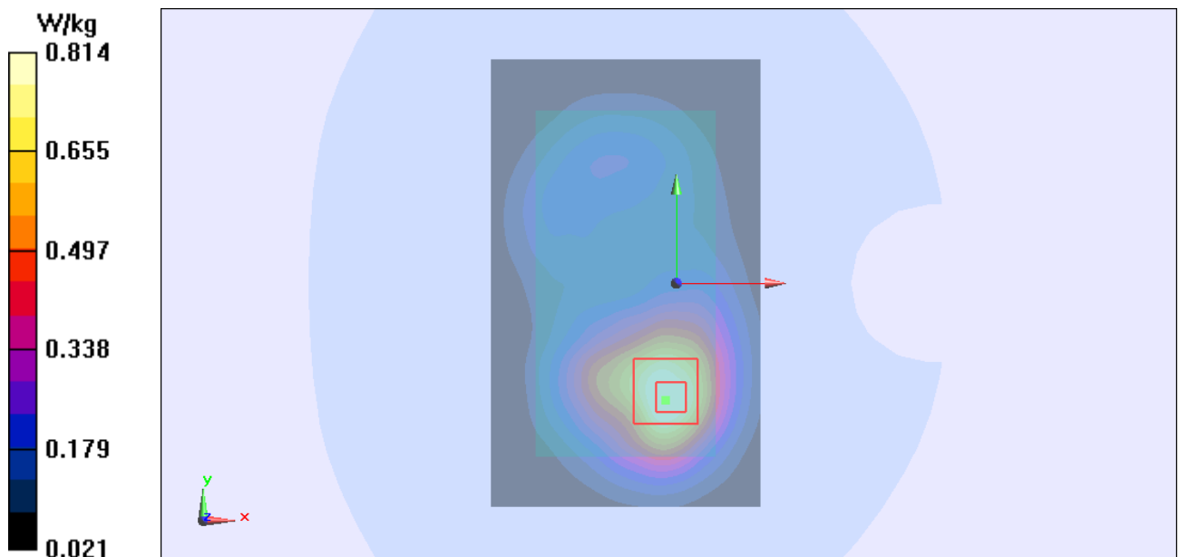
Figure Body, Front Side, GSM 1900 GPRS (4Txslots) Channel 661
