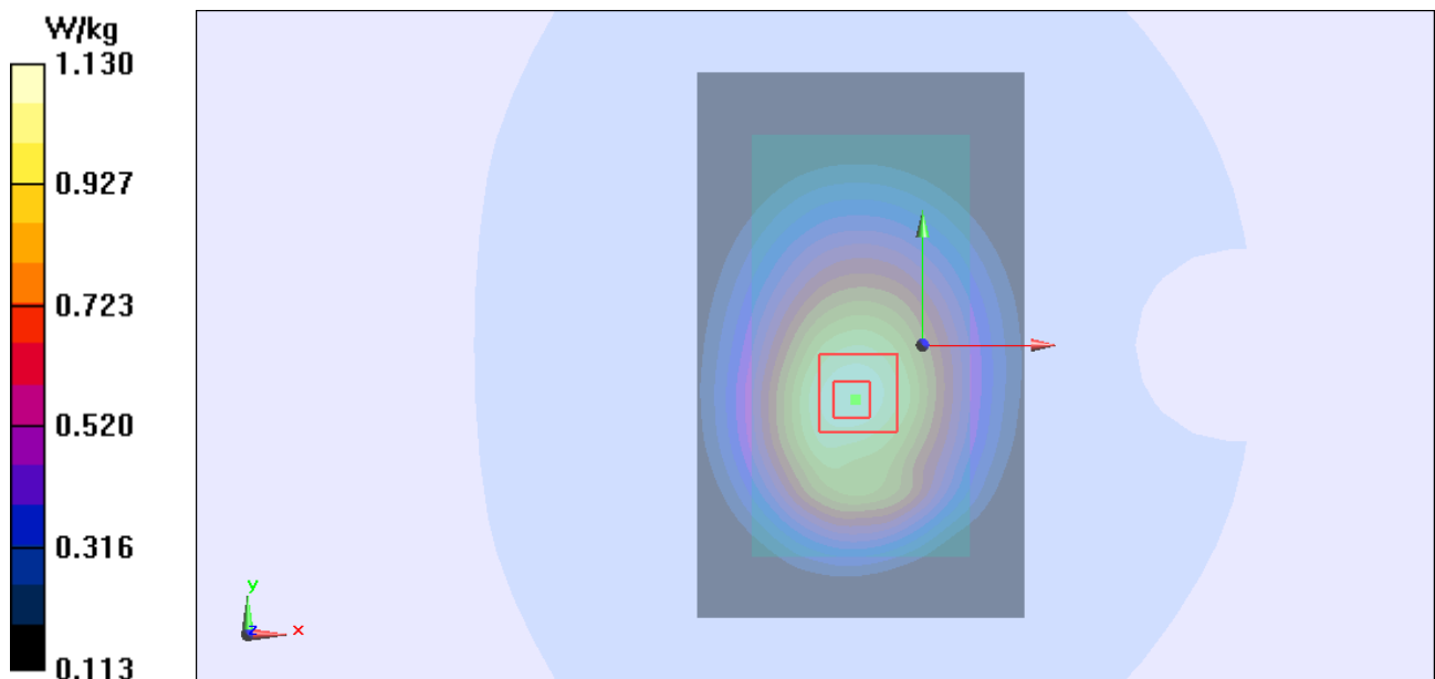
Figure Body, Back Side, GSM 850 GPRS (4Txslots) Channel 128
