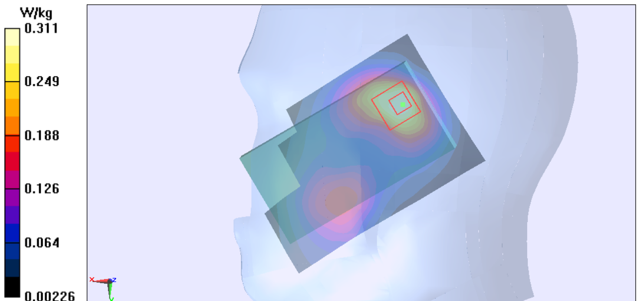
Figure Right Hand Tilt 15° UMTS Band II Channel 9400
