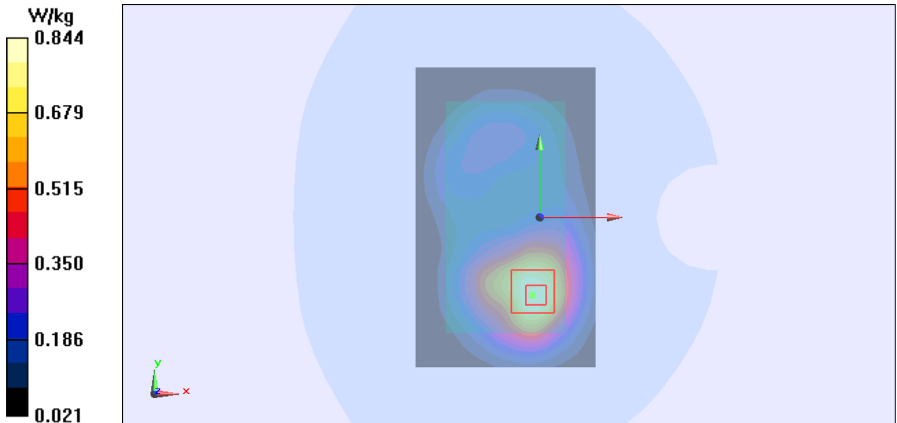
Figure Body, Front Side, UMTS Band II Channel 9538
