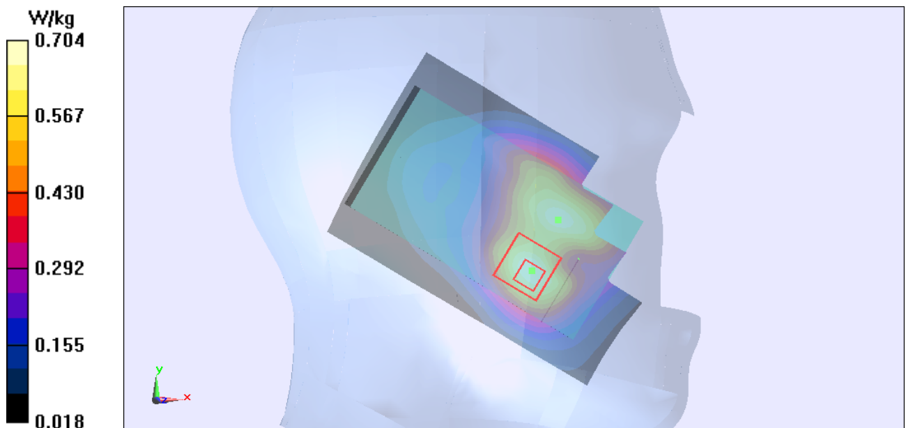
Figure Left Hand Touch Cheek UMTS Band II Channel 9538
