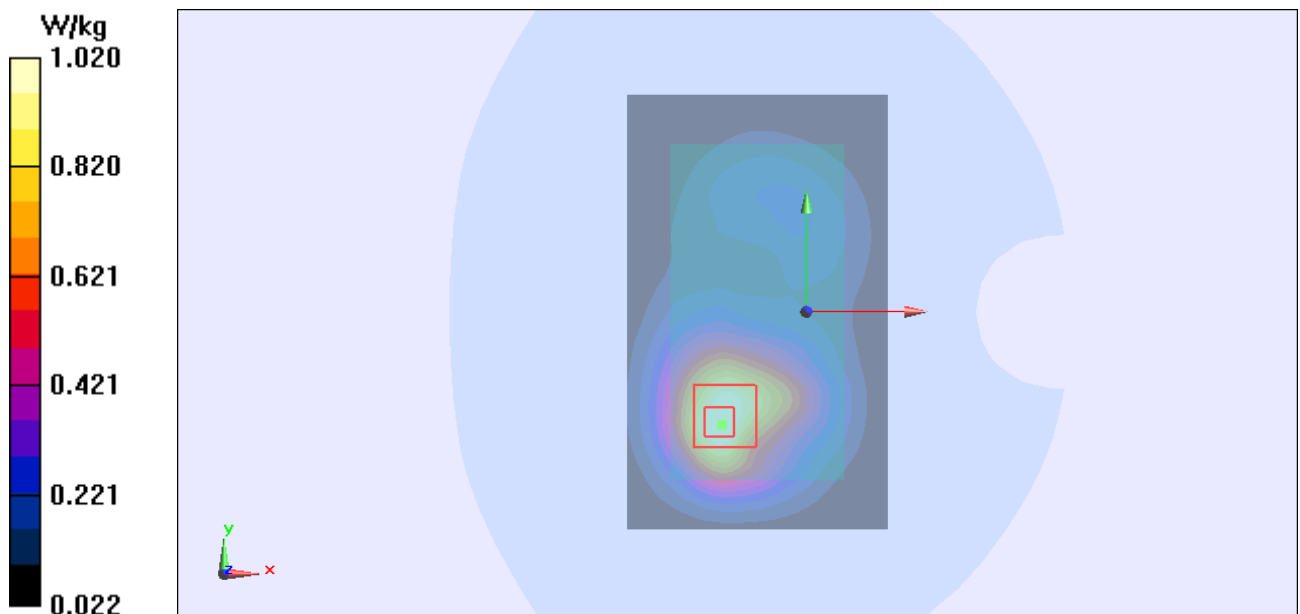
Figure Body, Back Side, UMTS Band II Channel 9538
