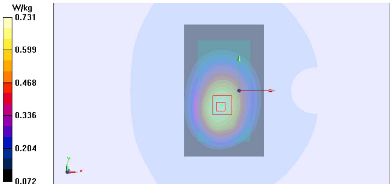
Figure Body, Back Side, GSM 850 Channel 190
