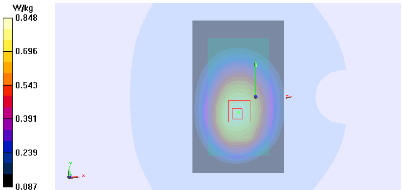
Figure Body, Back Side, GSM 850 GPRS (4Txslots) Channel 251
