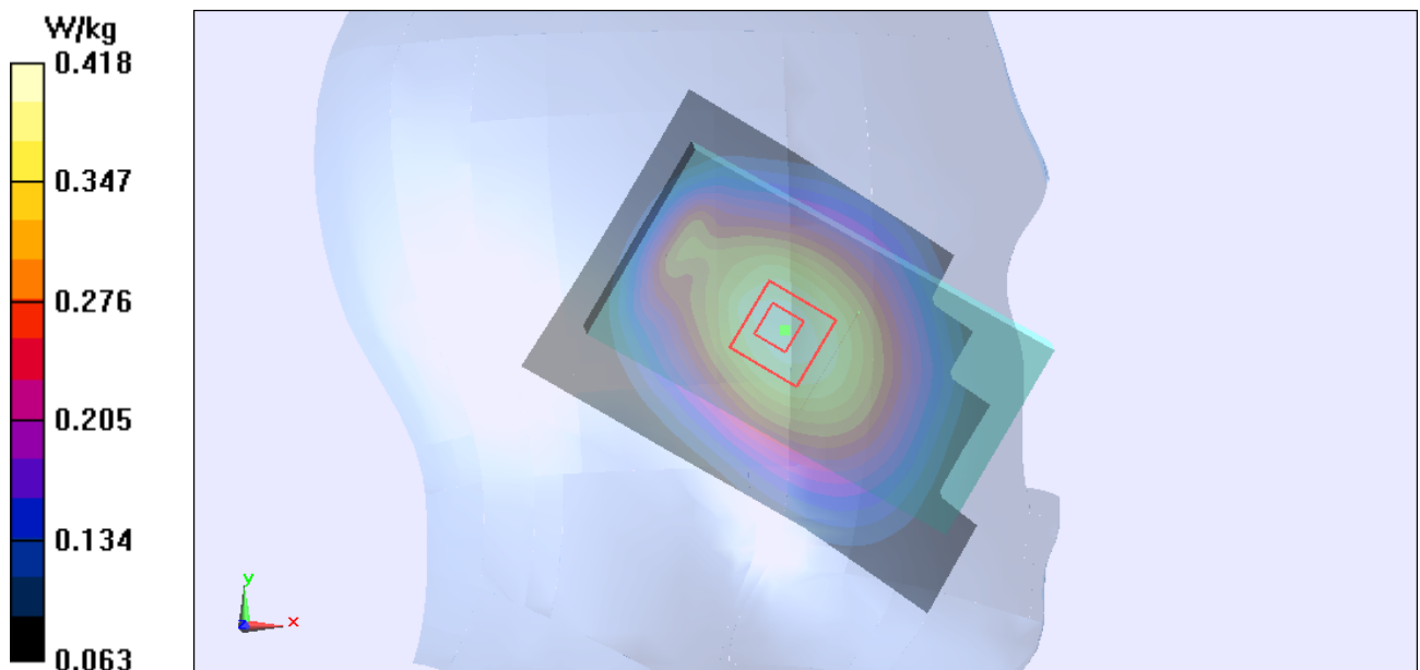
Figure Left Hand Tilt 15° GSM 850 Channel 190
