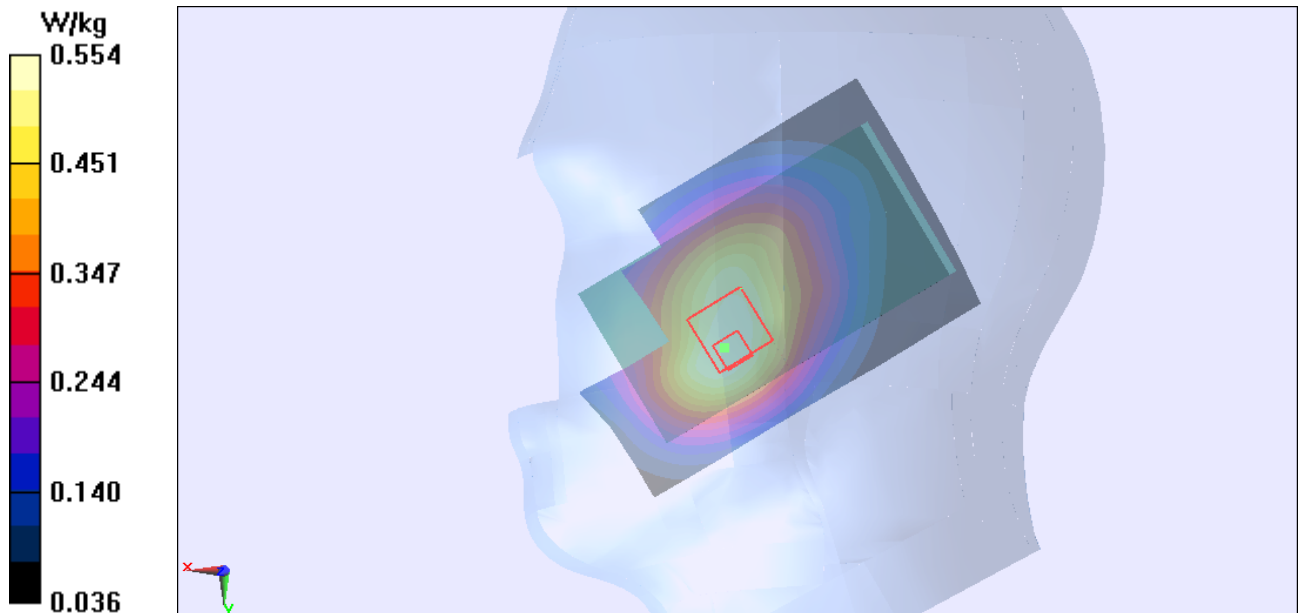
Figure Right Hand Touch Cheek UMTS Band V Channel 4183
