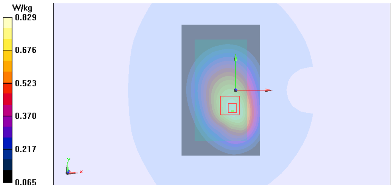
Figure Body, Front Side, GSM 850 GPRS (4Txslots)Channel 190
