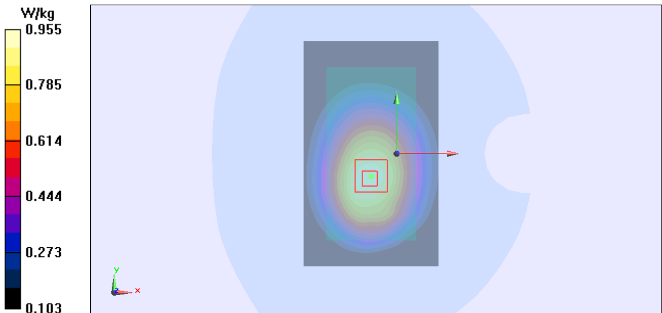
Figure Body, Back Side, GSM 850 GPRS (4Txslots) Channel 190
