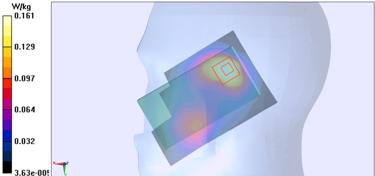
Figure Right Hand Tilt 15° GSM 1900 Channel 661
