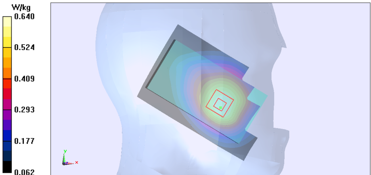
Figure Left Hand Touch Cheek GSM 850 Channel 190
