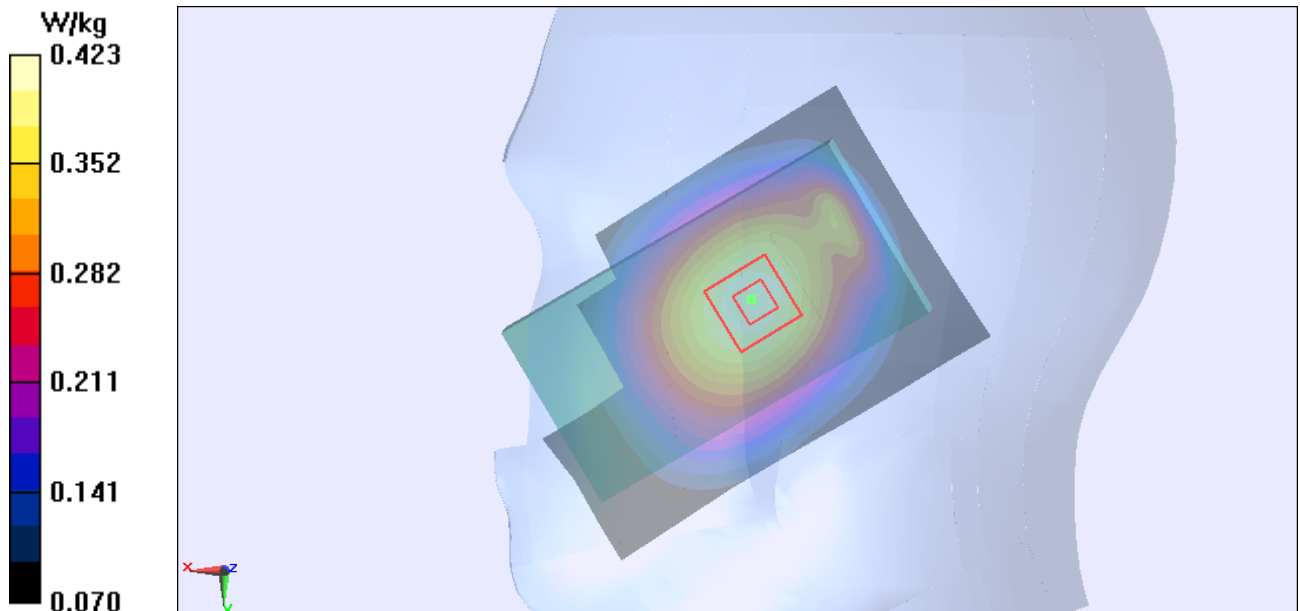
Figure Right Hand Tilt 15° GSM 850 Channel 190
