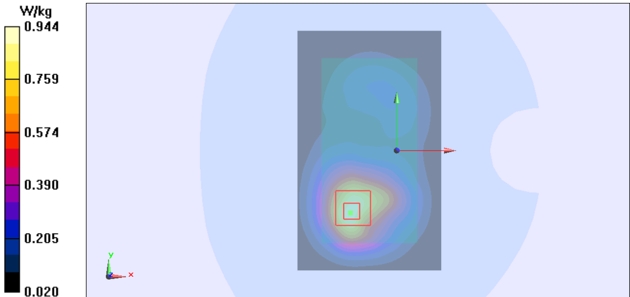
Figure Body, Back Side, GSM 1900 EGPRS (4Txslots) Channel 661
