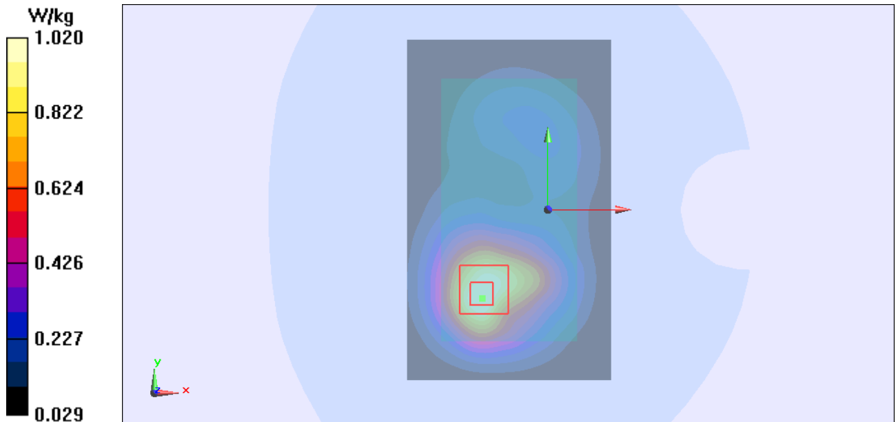
Figure Body, Back Side, UMTS Band II Channel 9400
