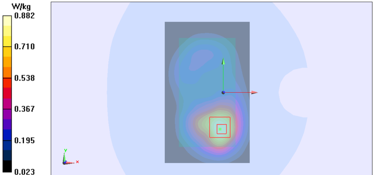
Figure Body, Front Side, UMTS Band II Channel 9400
