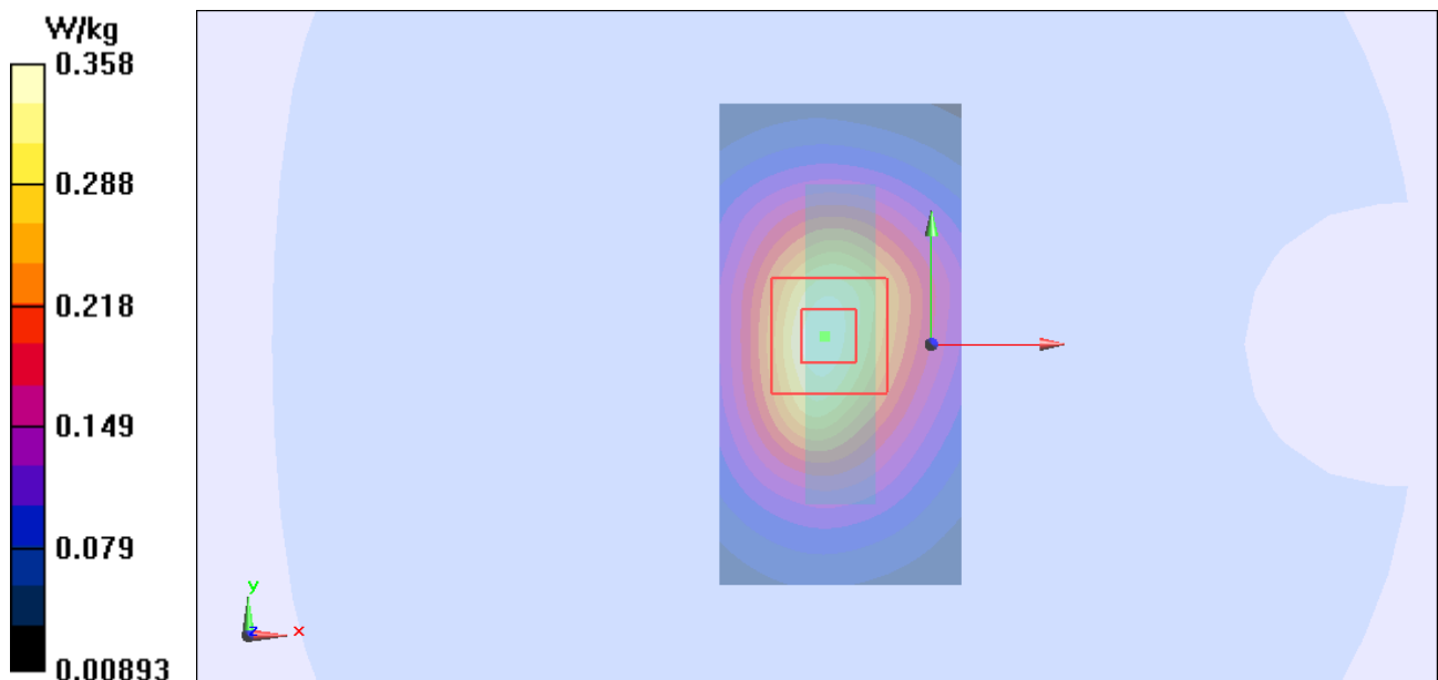
Figure Body, Bottom Edge, GSM 1900 GPRS (4Txslots) Channel 661
