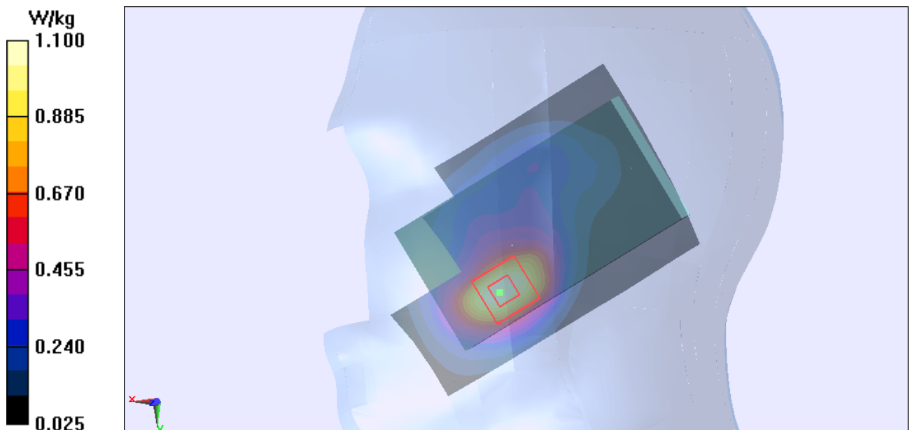
Figure Right Hand Touch Cheek UMTS Band II Channel 9262
