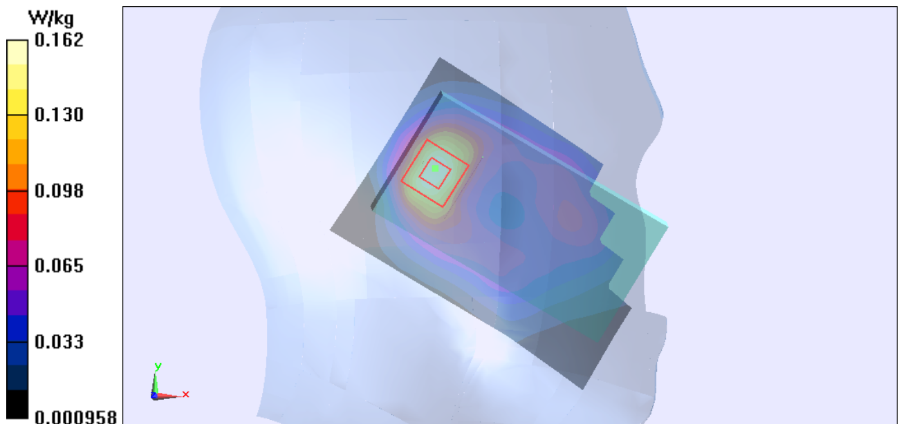
Figure Left Hand Tilt 15° GSM 1900 Channel 661
