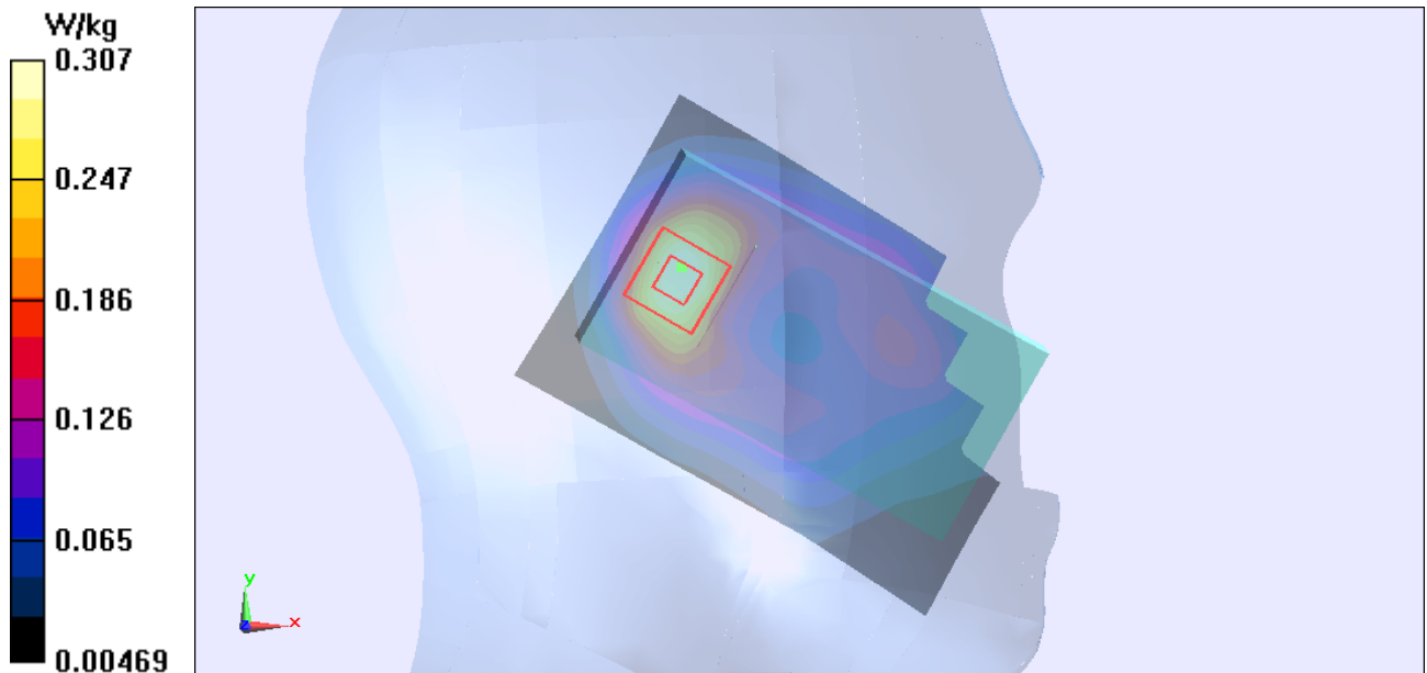
Figure Left Hand Tilt 15° UMTS Band II Channel 9400
