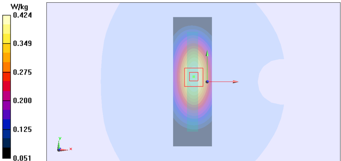
Figure Body, Right Edge, GSM 850 GPRS (4Txslots)Channel 190
