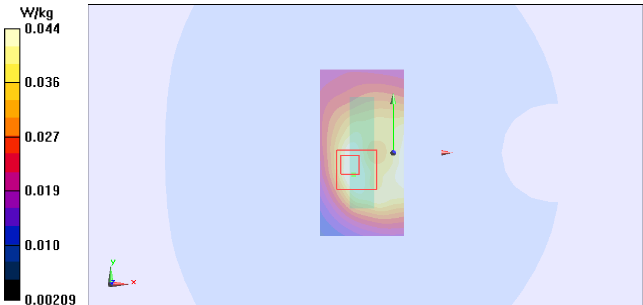
Figure Body, Bottom Edge, GSM 850 GPRS (4Txslots)annel 190
