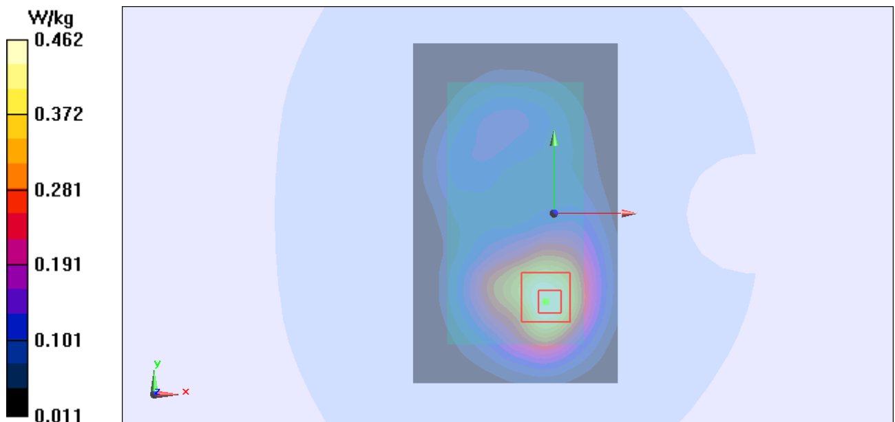
Figure Body, Front Side, GSM 1900 Channel 661
