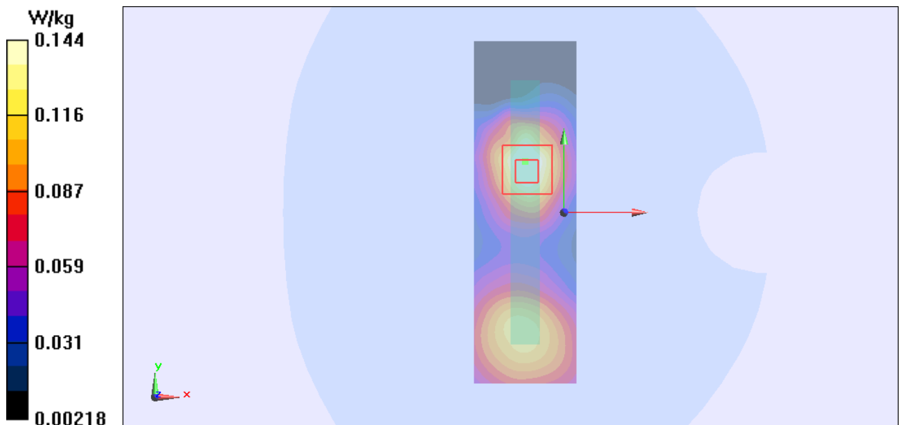
Figure Body, Left Edge, GSM 1900 GPRS (4Txslots) Channel 661
