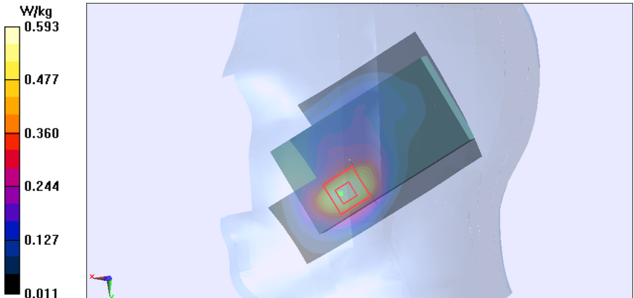
Figure Right Hand Touch Cheek GSM 1900 Channel 661
