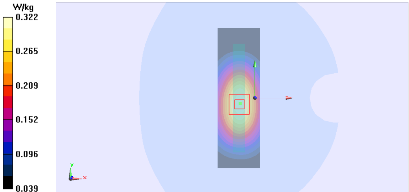
Figure Body, Left Edge, GSM 850 GPRS (4Txslots)Channel 190
