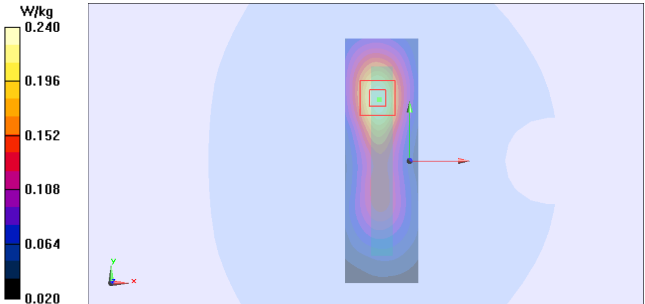
Figure Body, Right Edge, GSM 1900 GPRS (4Txslots) Channel 661
