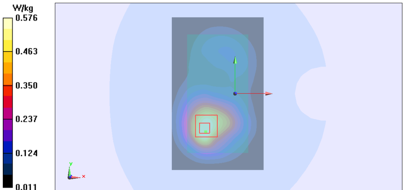
Figure Body, Back Side, GSM 1900 Channel 661
