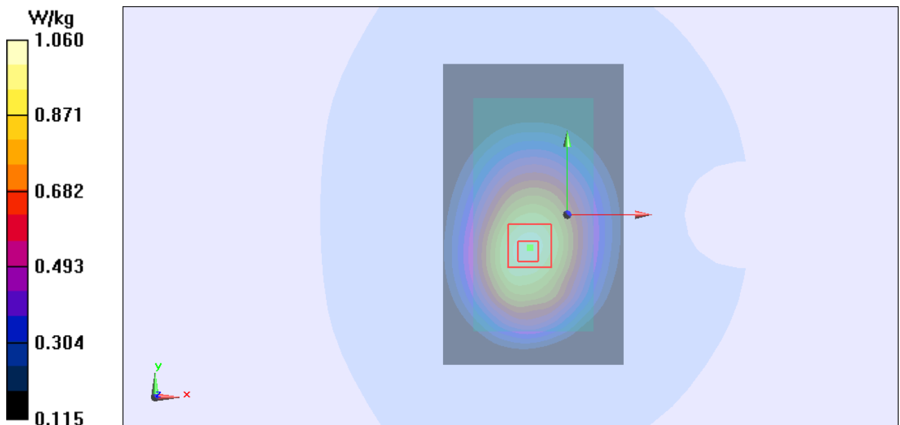
Figure Body, Back Side, GSM 850 EGPRS (4Txslots) Channel 128
