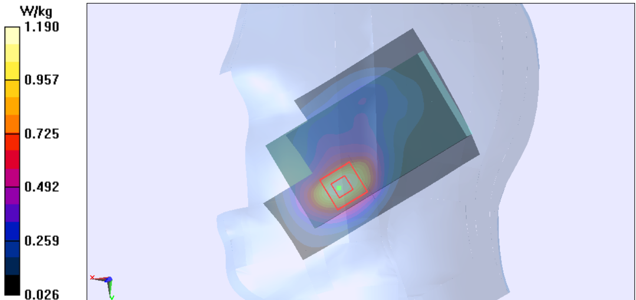
Figure Right Hand Touch Cheek UMTS Band II Channel 9400
