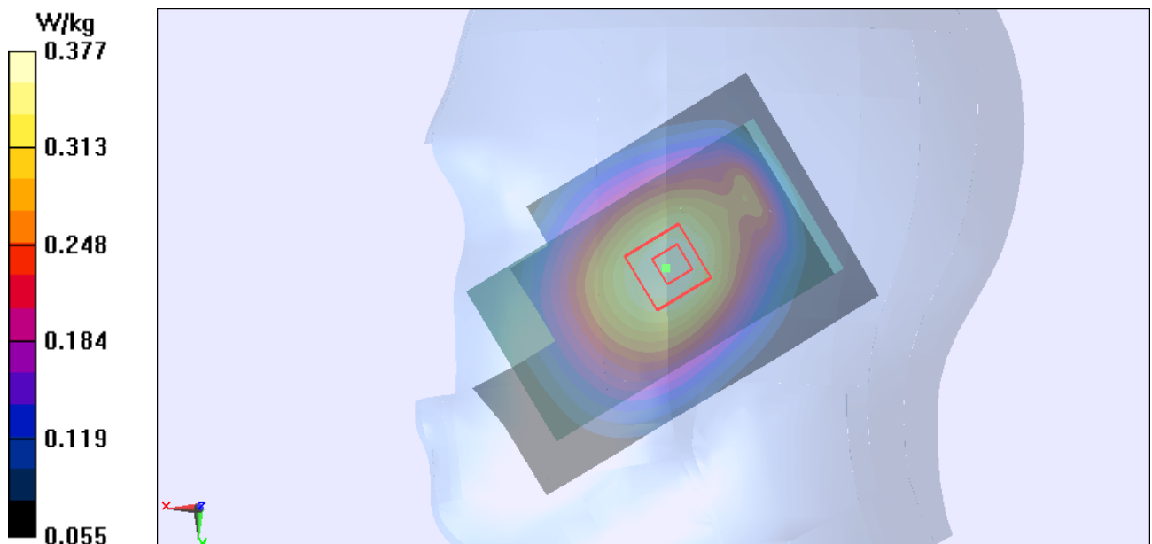
Figure Right Hand Tilt 15° UMTS Band V Channel 4183
