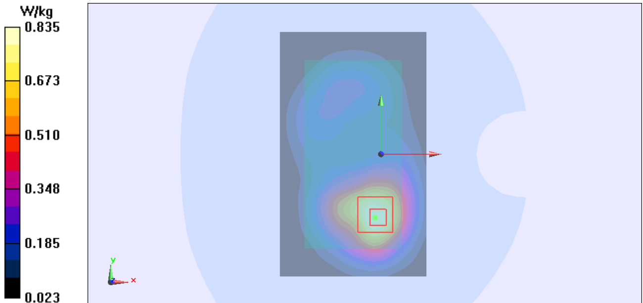
Figure Body, Front Side, UMTS Band II Channel 9262
