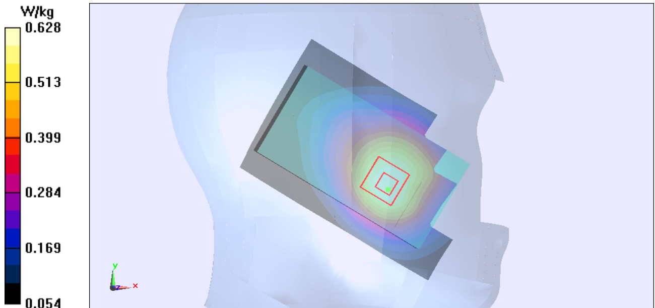
Figure Left Hand Touch Cheek UMTS Band V Channel 4183
