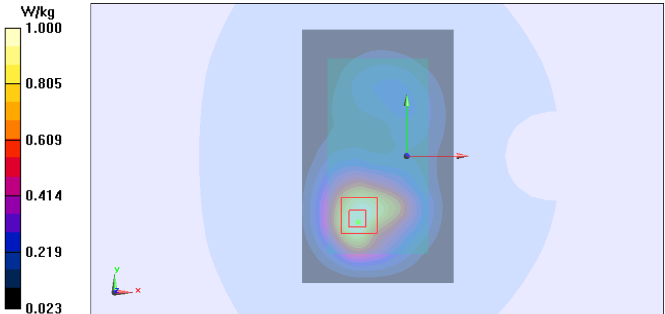
Figure Body, Back Side, UMTS Band II Channel 9262
