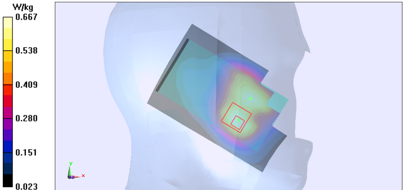
Figure Left Hand Touch Cheek UMTS Band II Channel 9262
