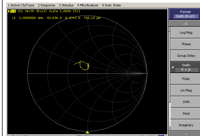
Impedance Test-Body
