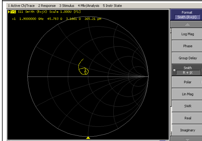
Impedance Test-Body
