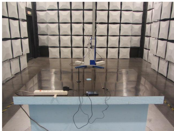
Radiated Spurious Emission (30MHz-1GHz)
