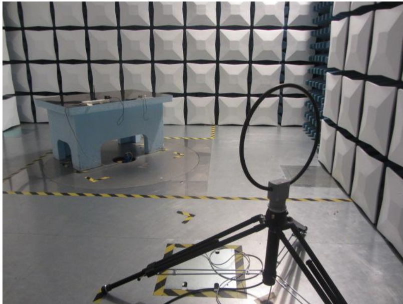
Radiated Spurious Emission (9 KHz-30 MHz)
