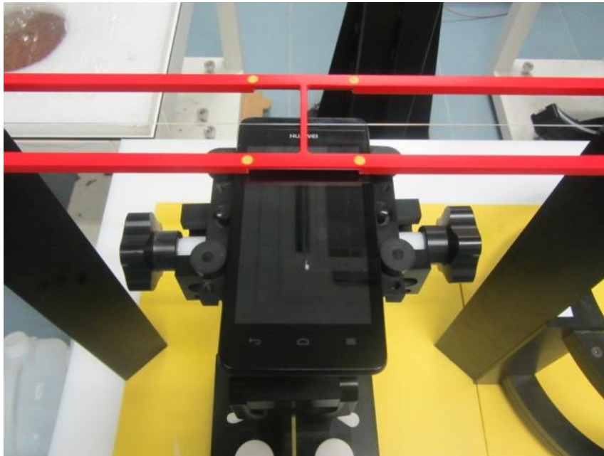
HAC RF test photo
