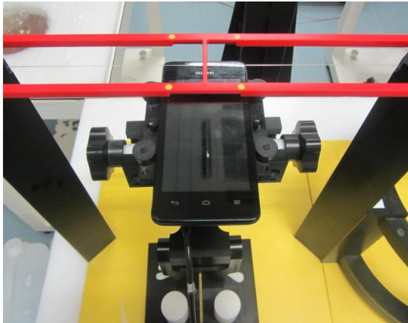
HAC T-coil test photo
