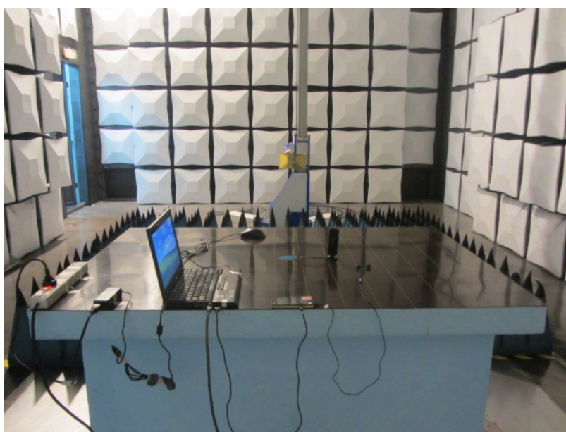
Radiated Disturbance Emissions (1GHz to 18GHz)
