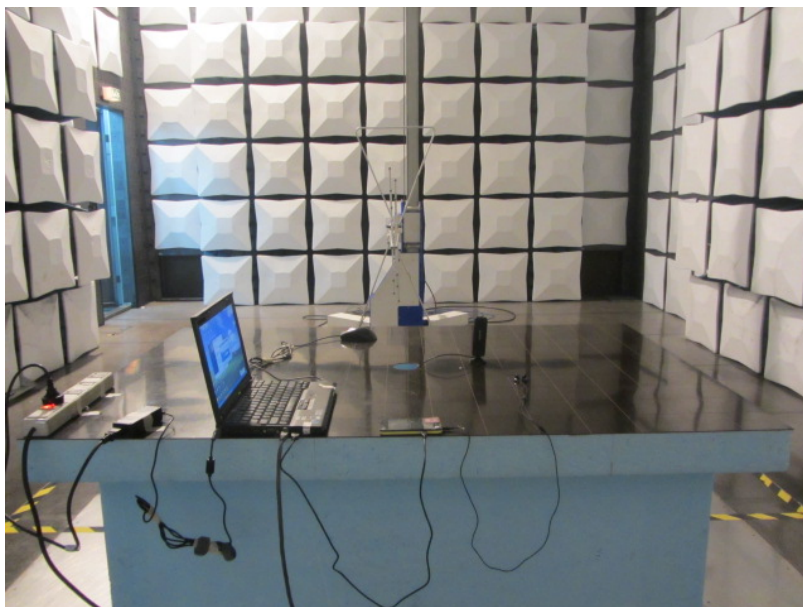
Radiated Disturbance Emissions (below 1GHz)
