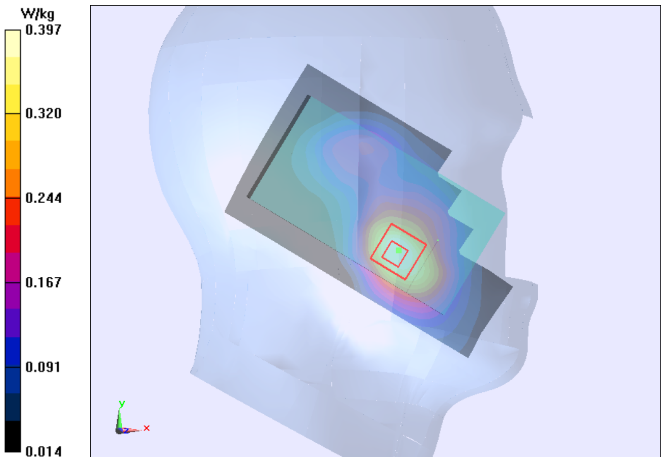
Figure 132 Left Hand Touch Cheek GSM 1900 Channel 661
