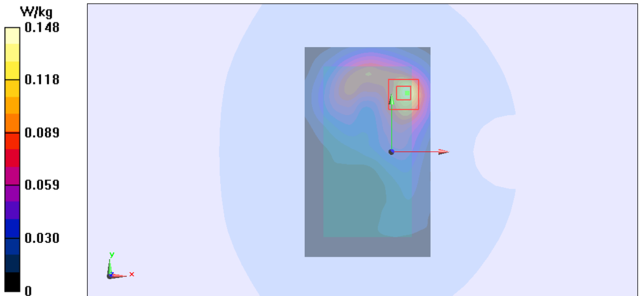
Figure 118 Body, Back Side, 802.11b Channel 1
