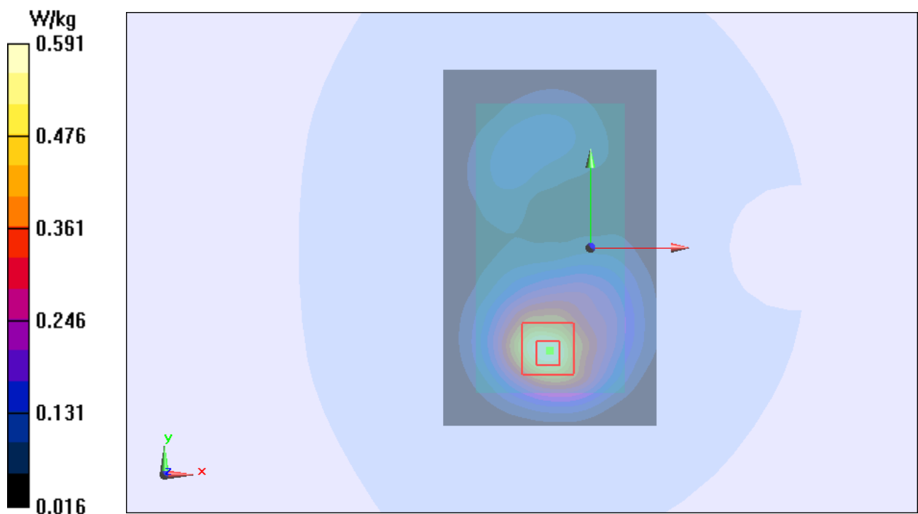
Figure 134 Body, Back Side, GSM 1900 Channel 661
