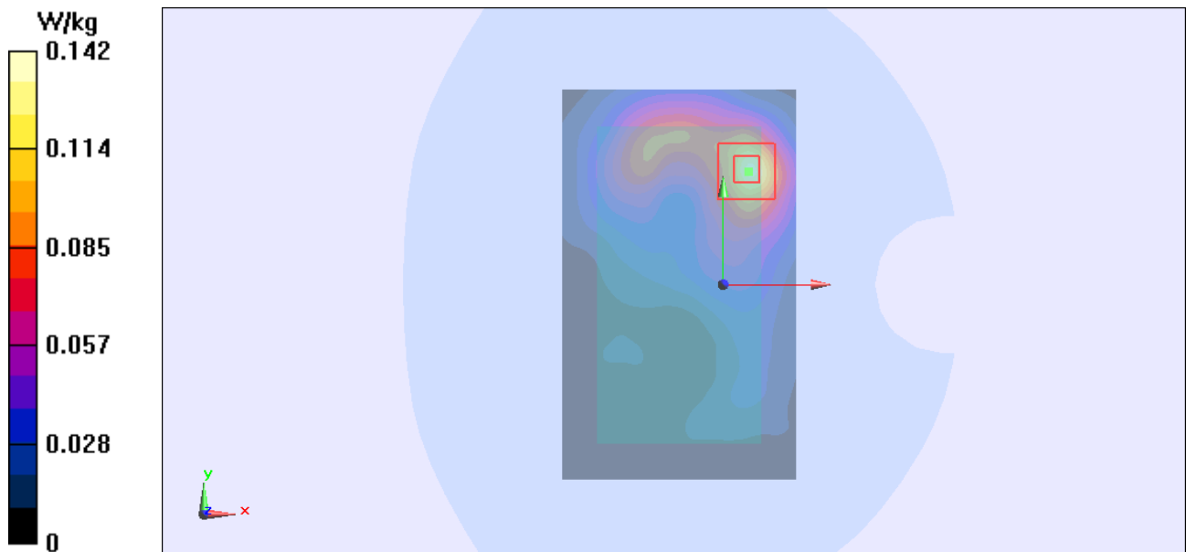
Figure 120 Body, Back Side, 802.11b Channel 1
