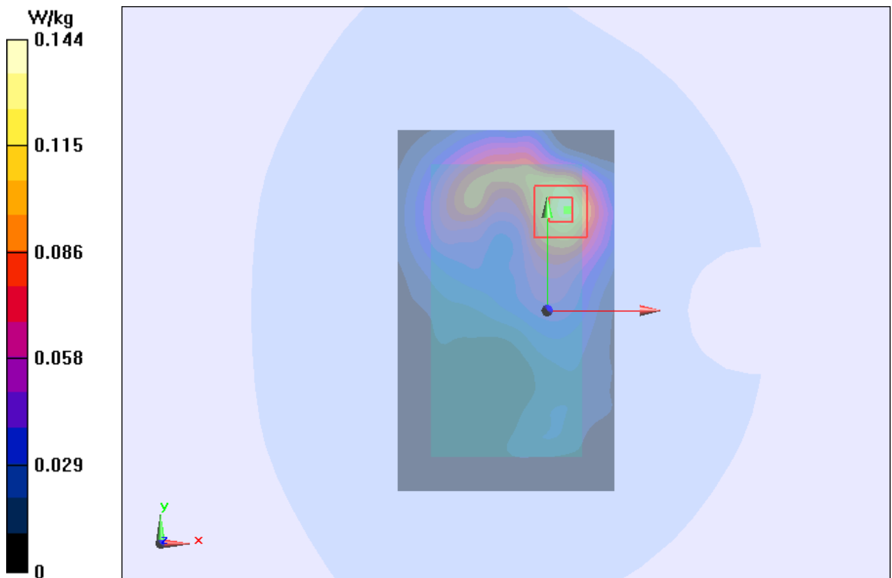
Figure 141 Body, Back Side, 802.11b Channel 1
