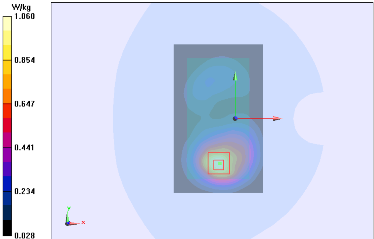
Figure 137 Body, Back Side, UMTS Band II Channel 9262
