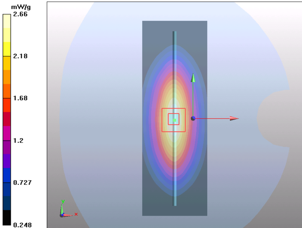
Figure 122 System Performance Check 835MHz 250mW
