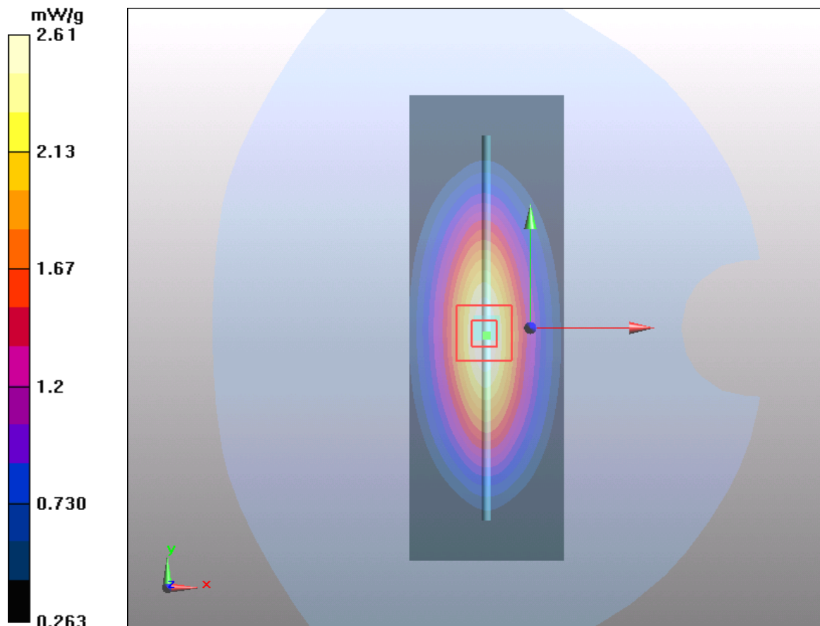
Figure 123 System Performance Check 835MHz 250mW
