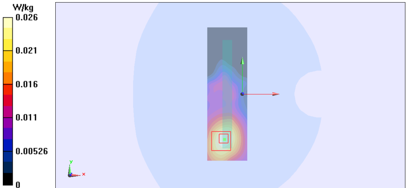
Figure 115 Body, Right Edge, 802.11b Channel 1
