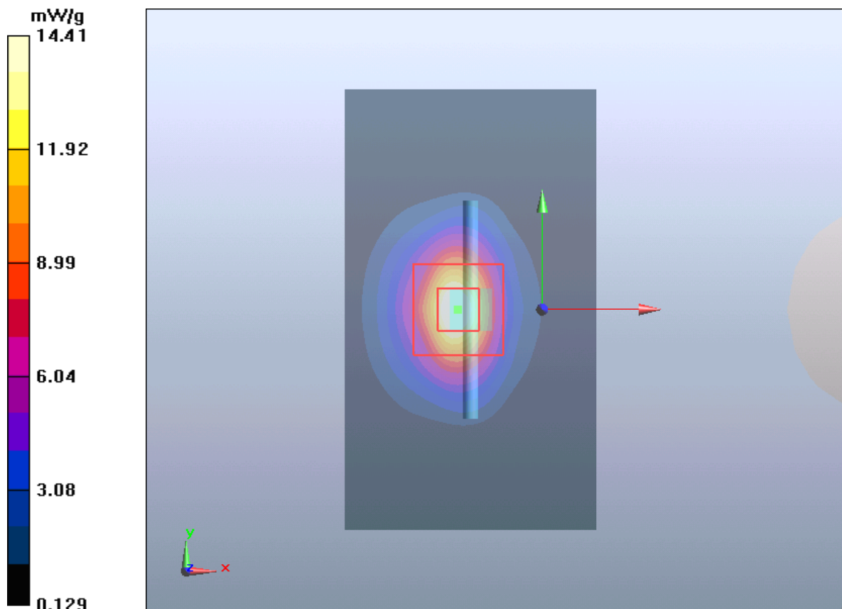
Figure 127 System Performance Check 2450MHz 250mW
