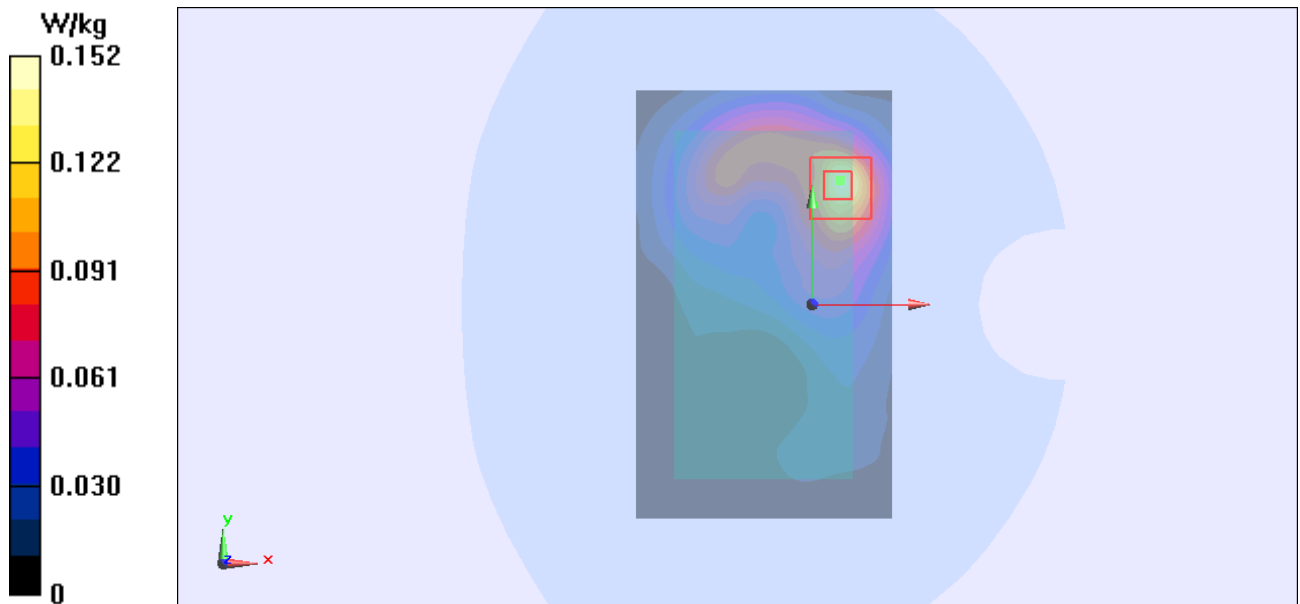
Figure 121 Body, Back Side, 802.11b Channel 1
