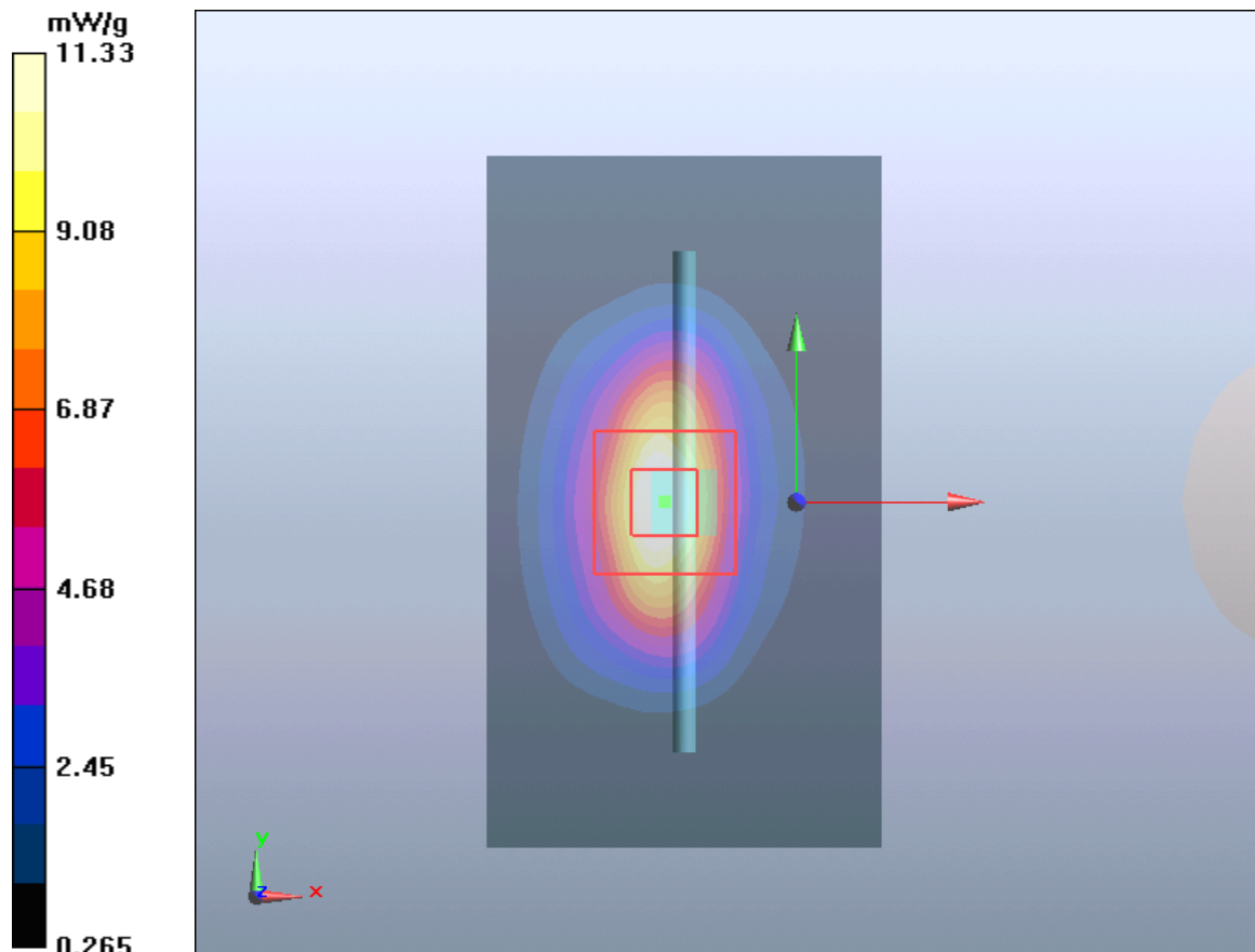
Figure 125 System Performance Check 1900MHz 250mW
