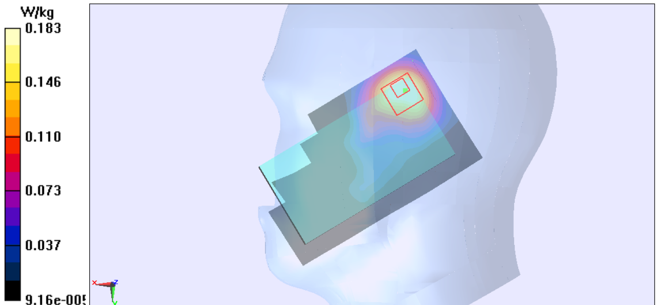
Figure 109 Right Hand Touch Cheek 802.11b Channel 1
