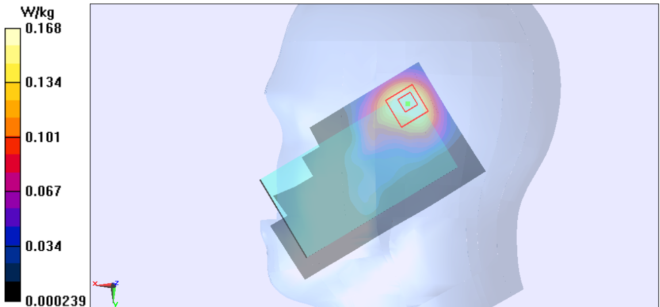
Figure 110 Right Hand Touch Cheek 802.11b Channel 1
