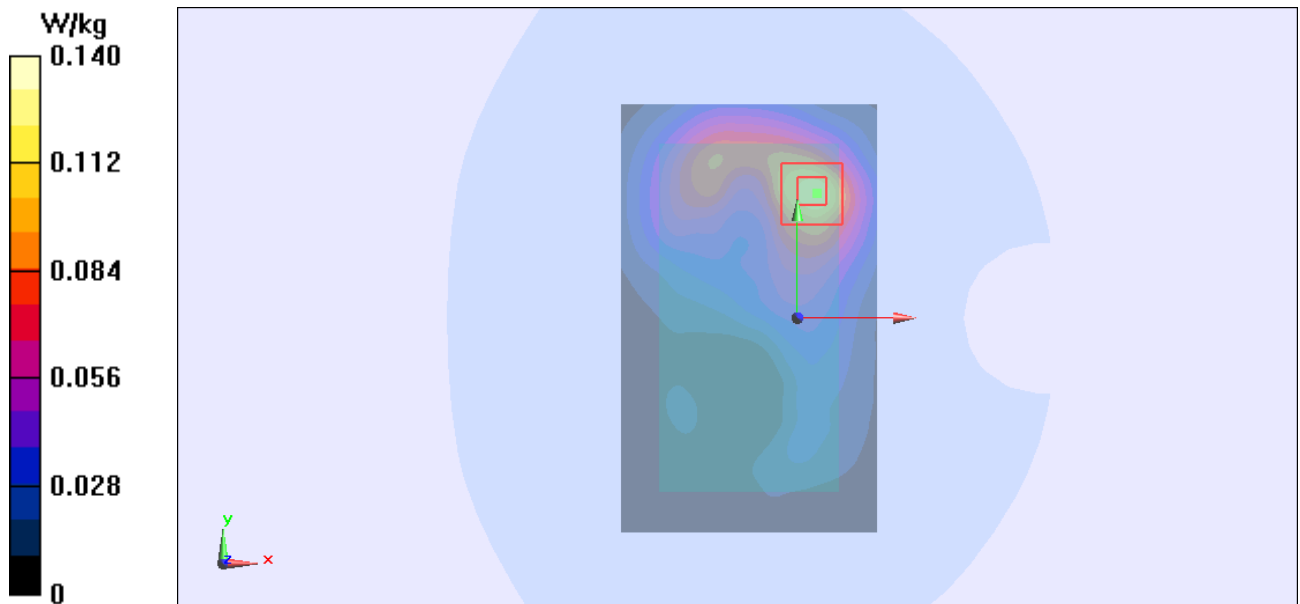
Figure 117 Body, Back Side, 802.11b Channel 1
