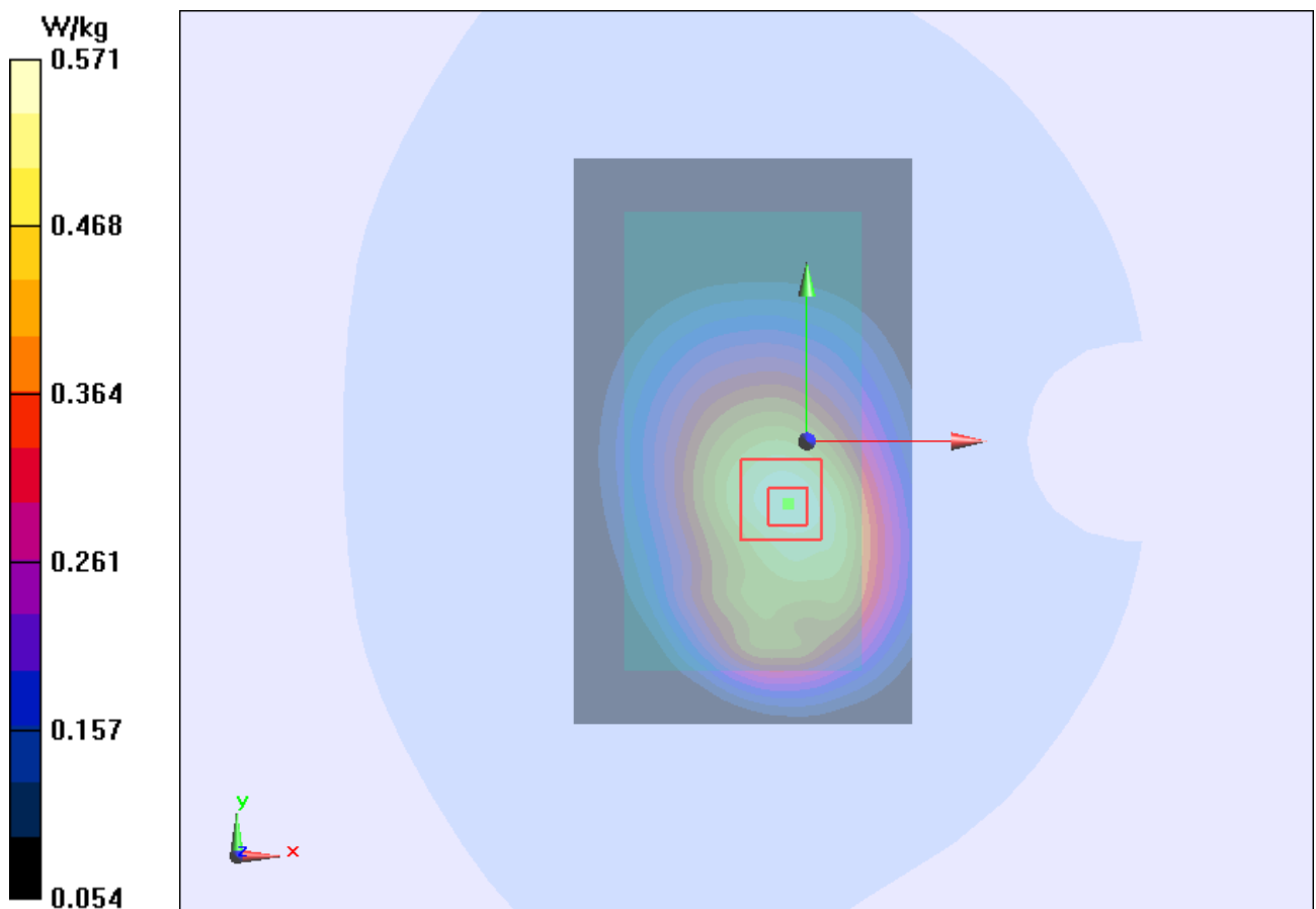
Figure 129 Body, Back Side, GSM 850 GPRS (2Txslots) Channel 190
