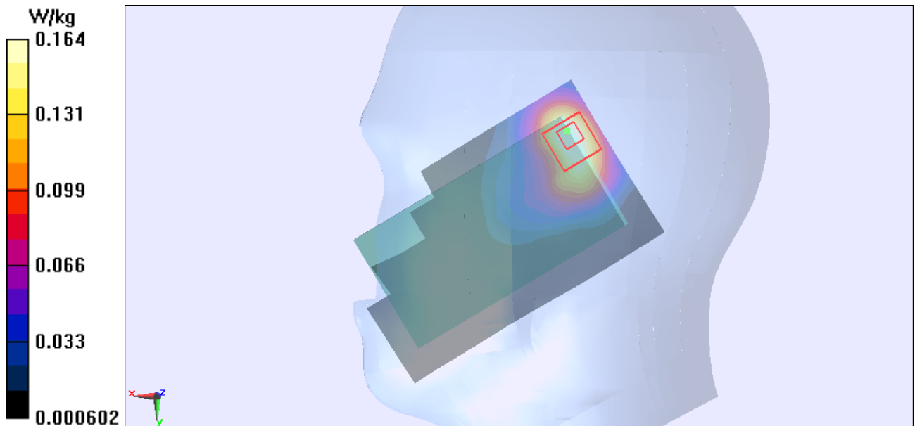
Figure 106 Right Hand Tilt 15° 802.11b Channel 1
