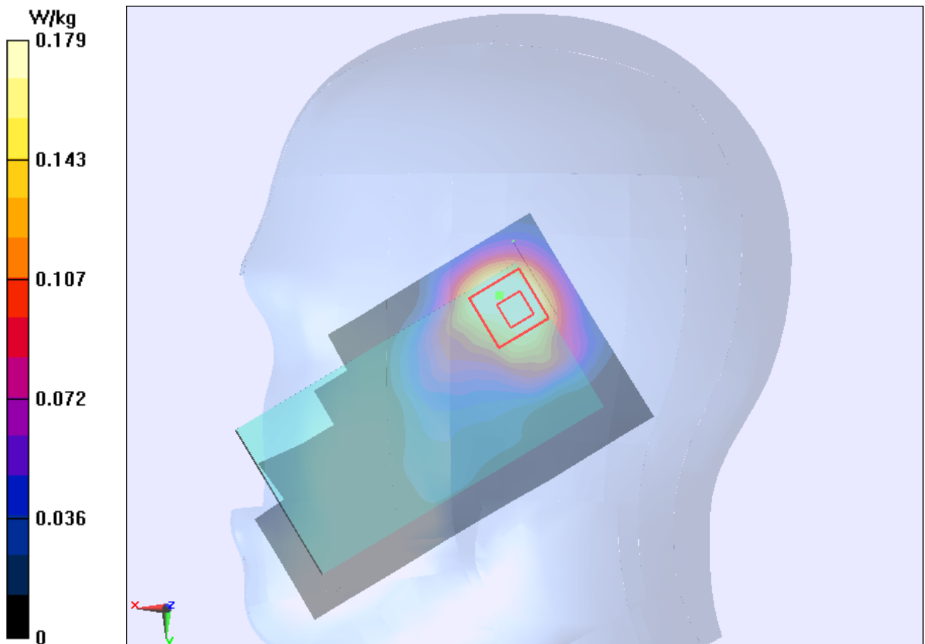
Figure 140 Right Hand Touch Cheek 802.11b Channel 1
