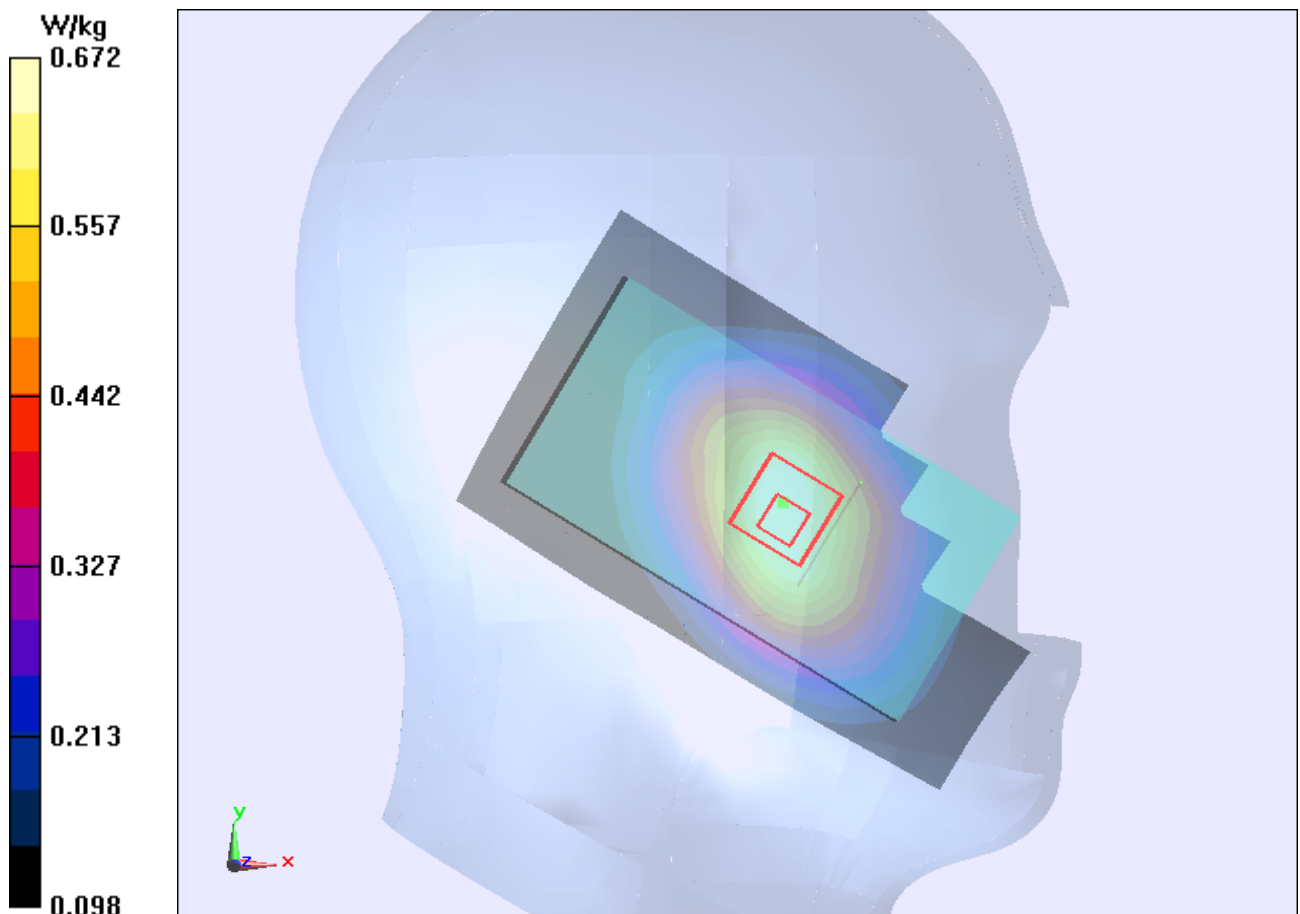
Figure 138 Left Touch Cheek UMTS Band V Channel 4183
