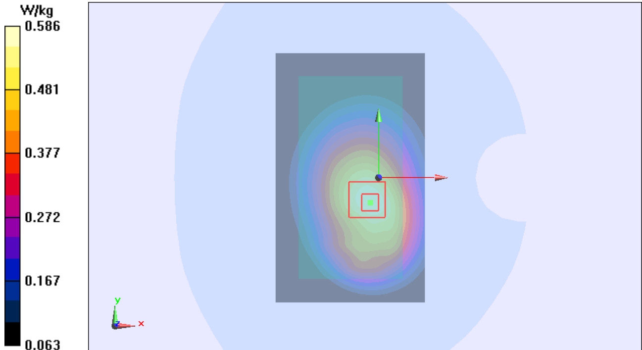
Figure 130 Body, Back Side, GSM 850 Channel 190
