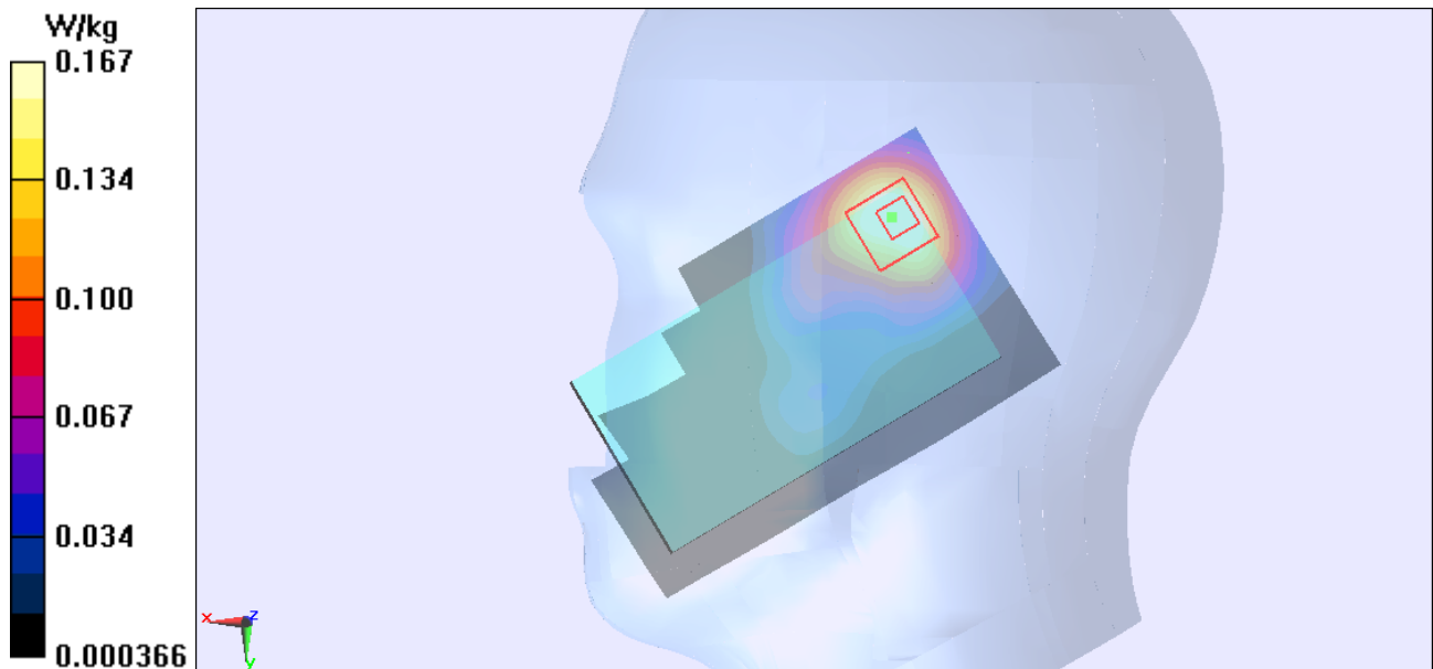
Figure 108 Right Hand Touch Cheek 802.11b Channel 1
