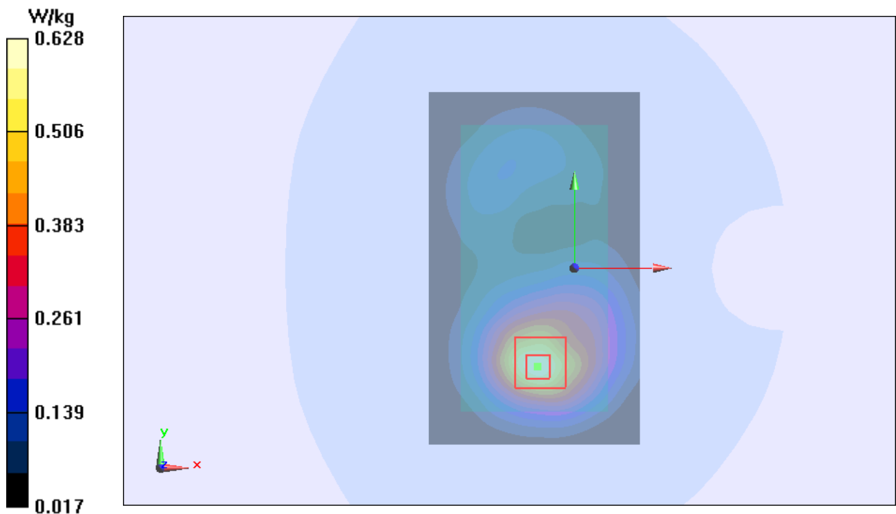
Figure 133 Body, Back Side, GSM 1900 GPRS (2Txslots) Channel 661
