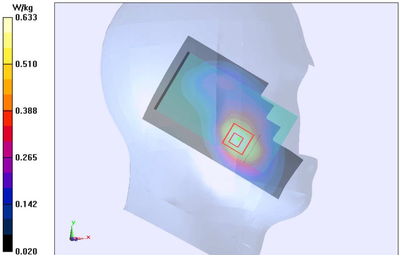
Figure 136 Left Hand Touch Cheek UMTS Band II Channel 9400
