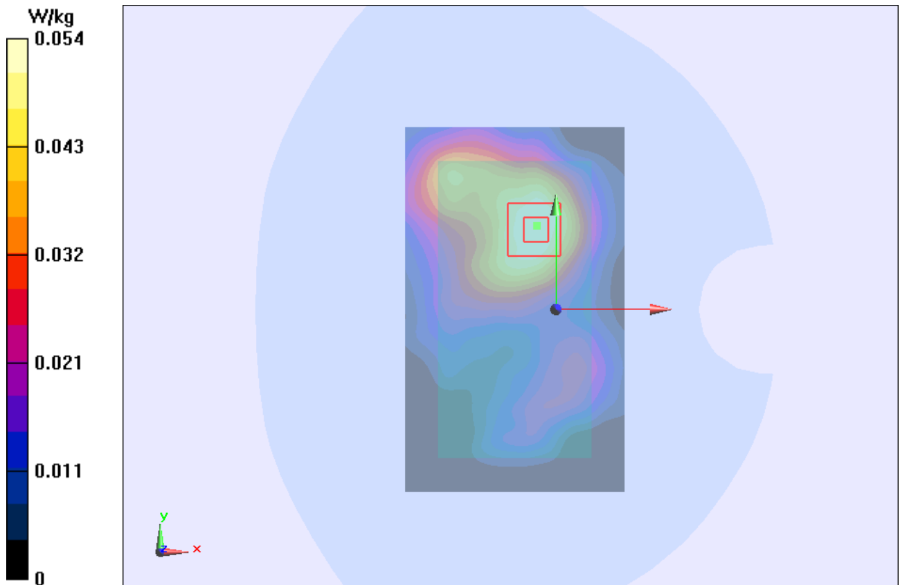
Figure 113 Body, Front Side, 802.11b Channel 1
