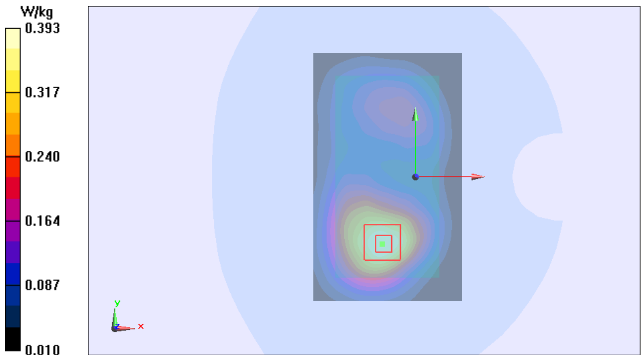
Figure 135 Body, Front Side, GSM 1900 Channel 661
