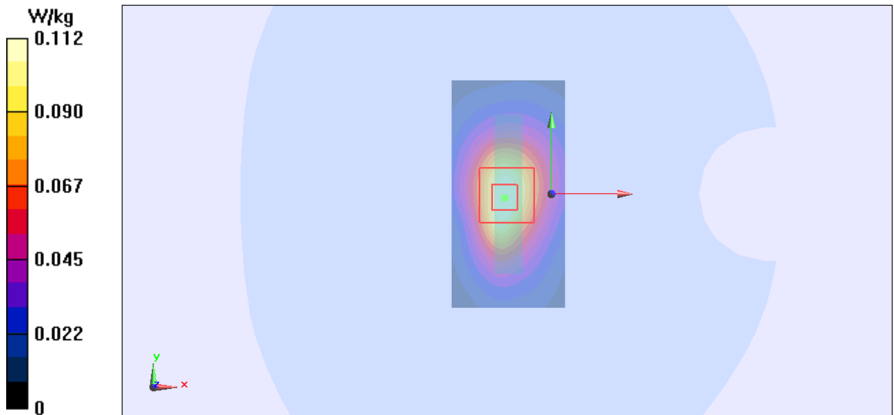
Figure 116 Body, Top Edge, 802.11b Channel 1
