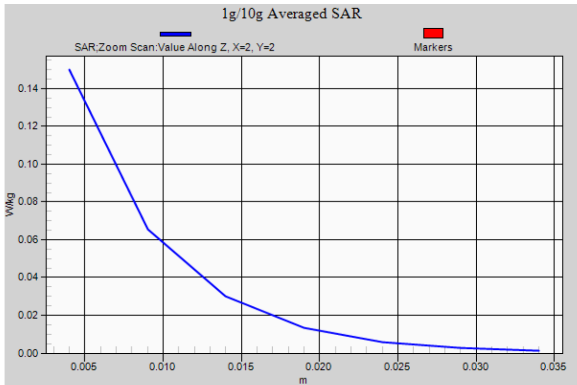
Figure 112 Body, Back Side, 802.11b Channel 1
