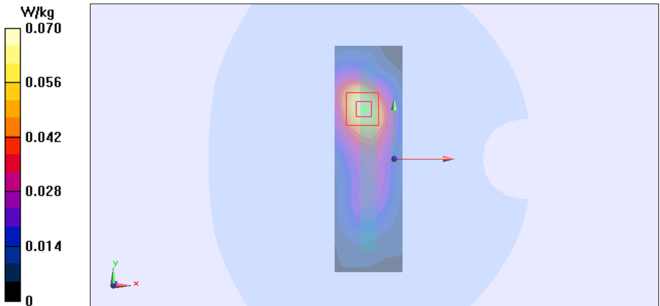
Figure 114 Body, Left Edge, 802.11b Channel 1
