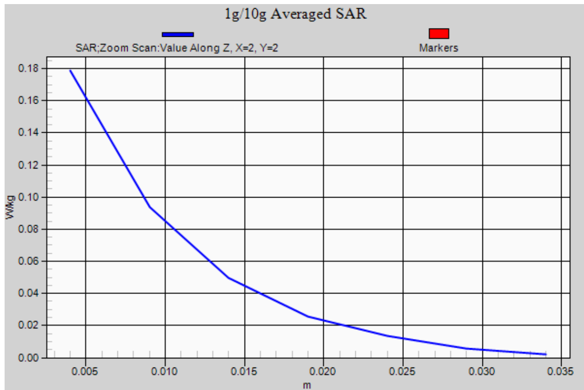
Figure 105 Right Hand Touch Cheek 802.11b Channel 1
