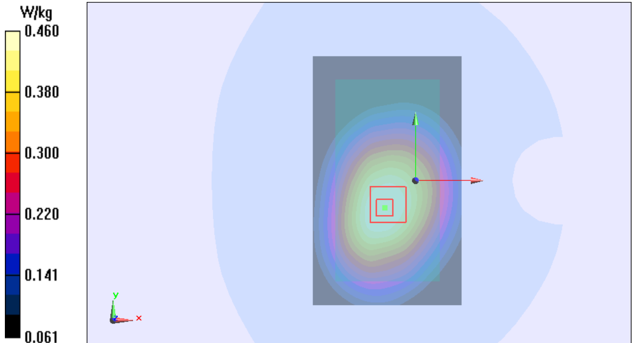
Figure 131 Body, Front Side, GSM 850 Channel 190
