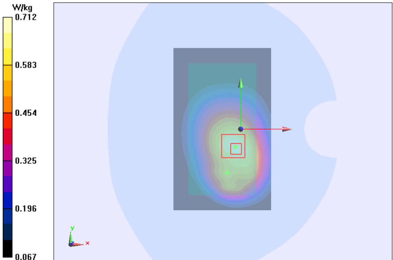
Figure 139 Body, Back Side, UMTS Band V Channel 4183
