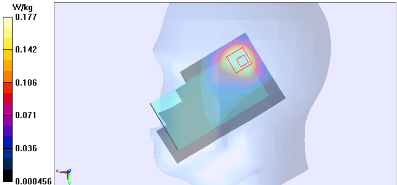
Figure 111 Right Hand Touch Cheek 802.11b Channel 1
