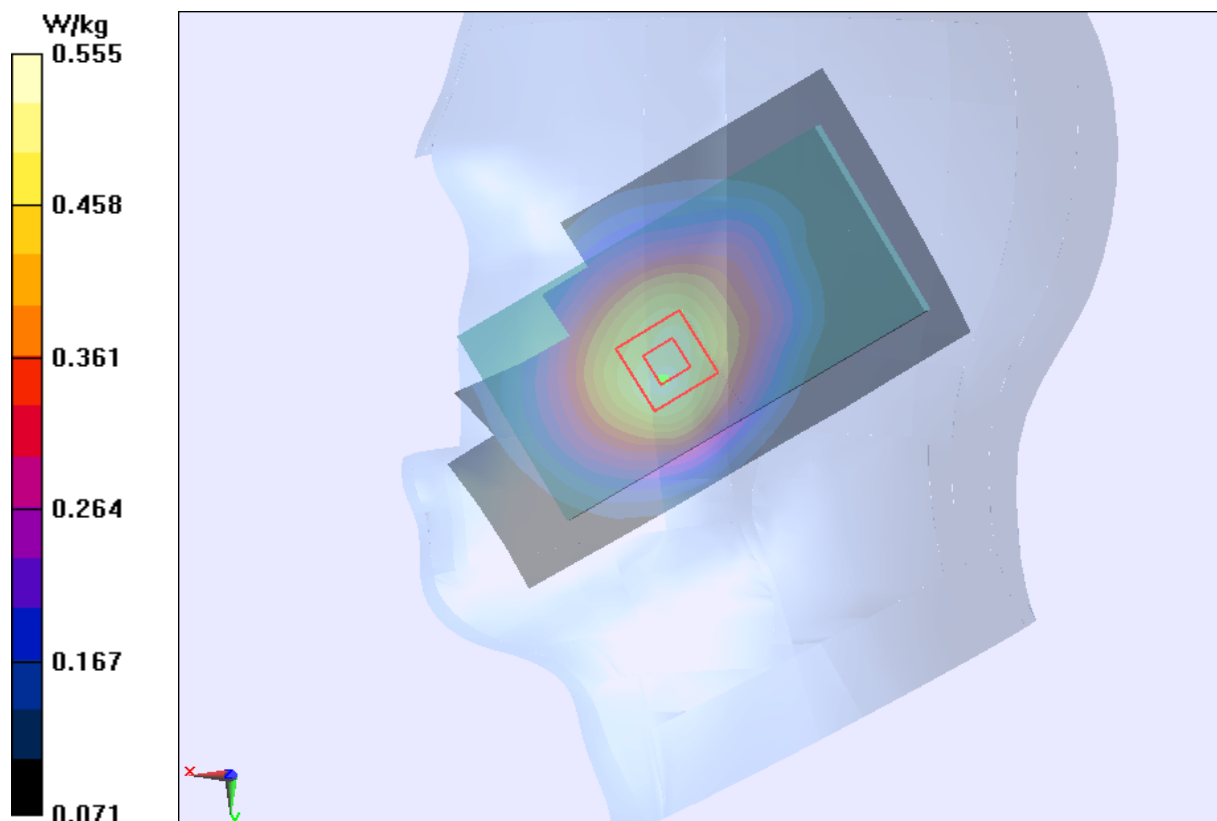
Figure 128 Right Touch Cheek GSM 850 Channel 190
