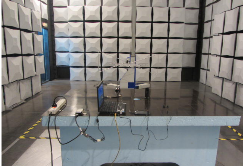
Radiated Spurious Emission (below 1GHz)
