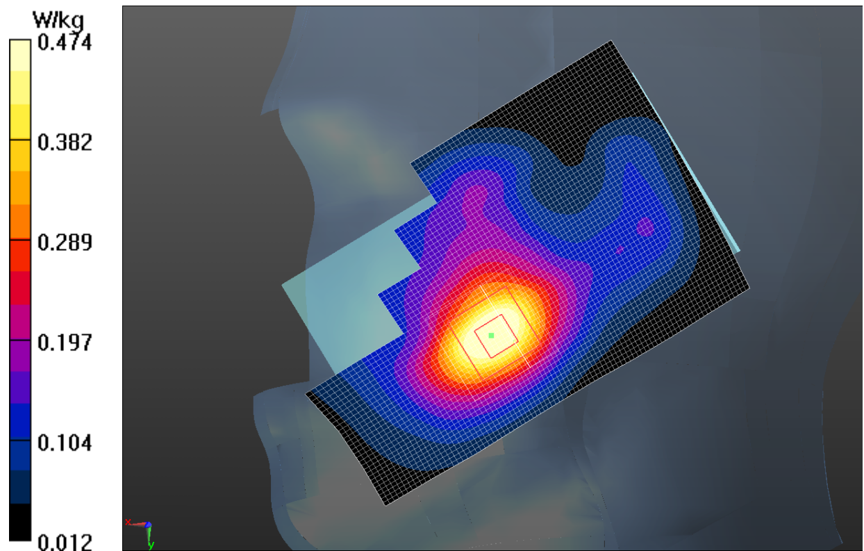
Fig.3 1900 MHz CH810
