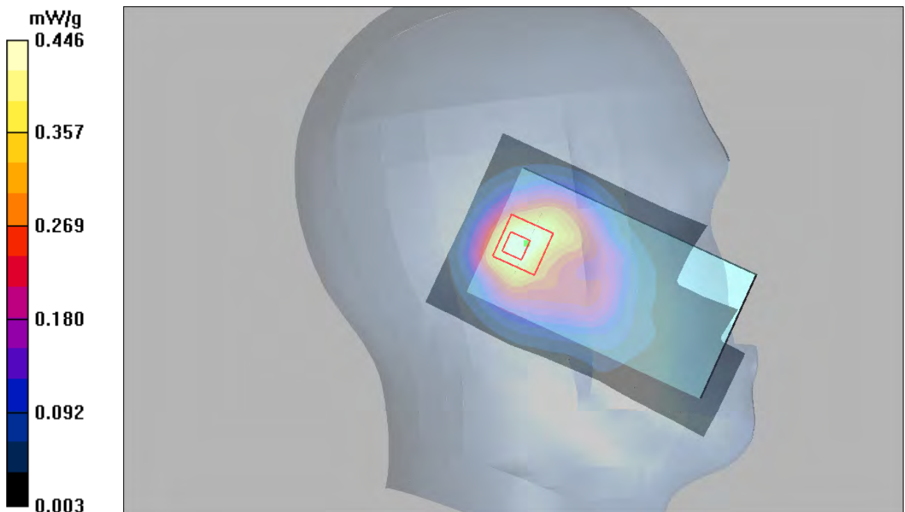
Figure 86 Left Hand Touch Cheek 802.11b Channel 11
