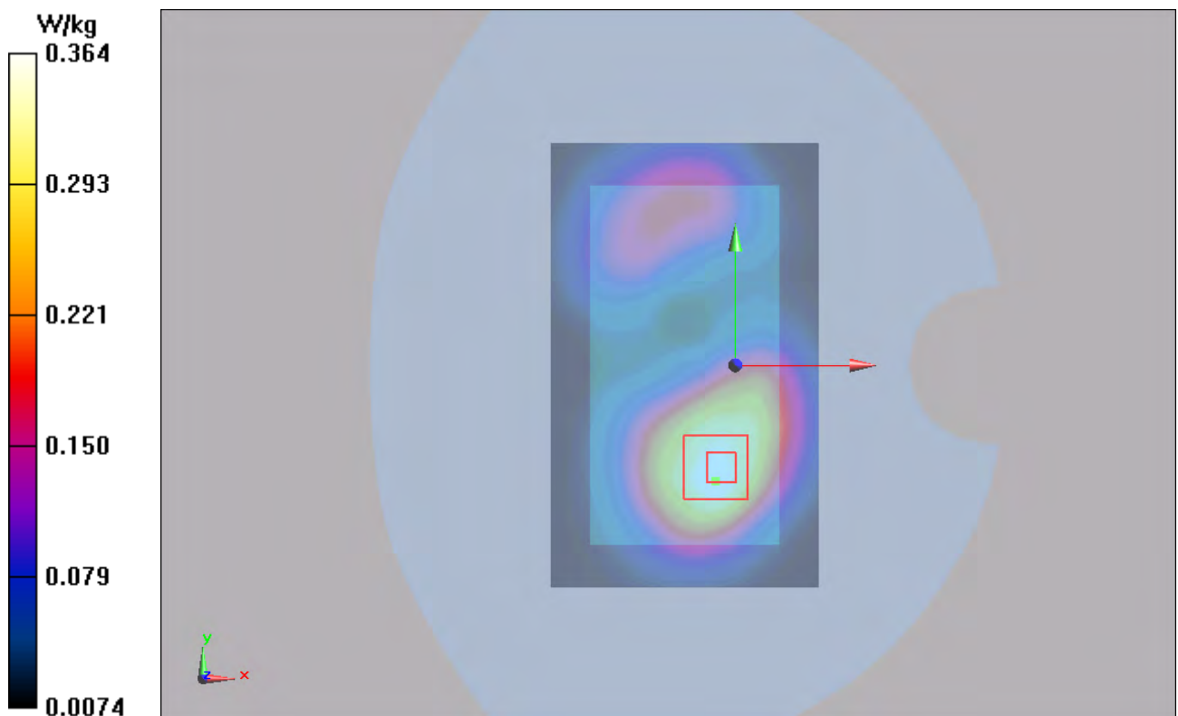
Figure 38 Body, Back Side, GSM 1900 Channel 661
