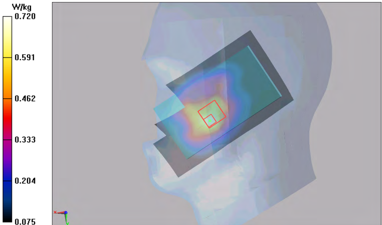
Figure 71 Right Hand Touch Cheek UMTS Band V Channel 4183
