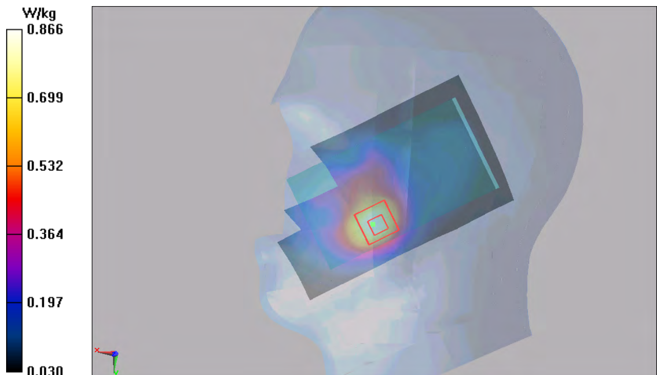
Figure 54 Right Hand Touch Cheek UMTS Band II Channel 9400
