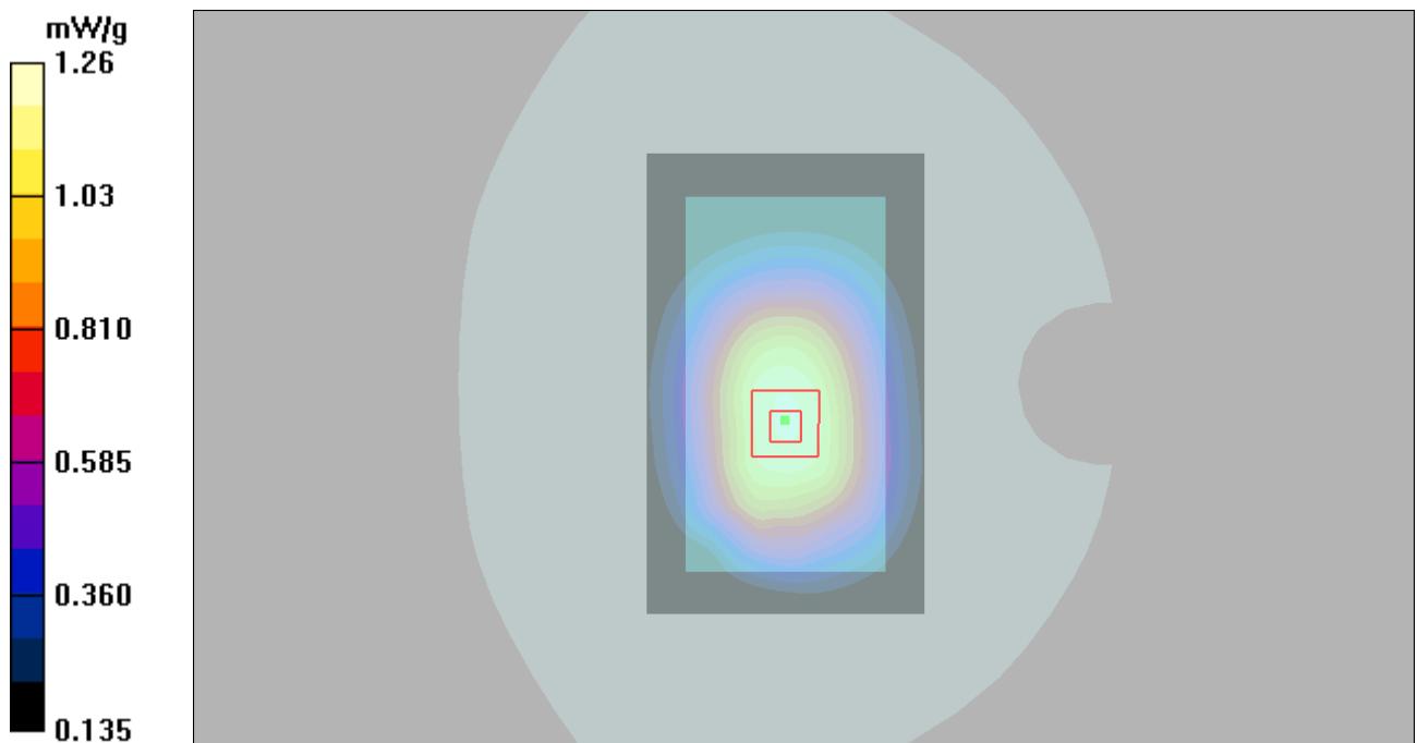
Figure 22 Body, Back Side, GSM 850 GPRS (4Txslots) Channel 251
