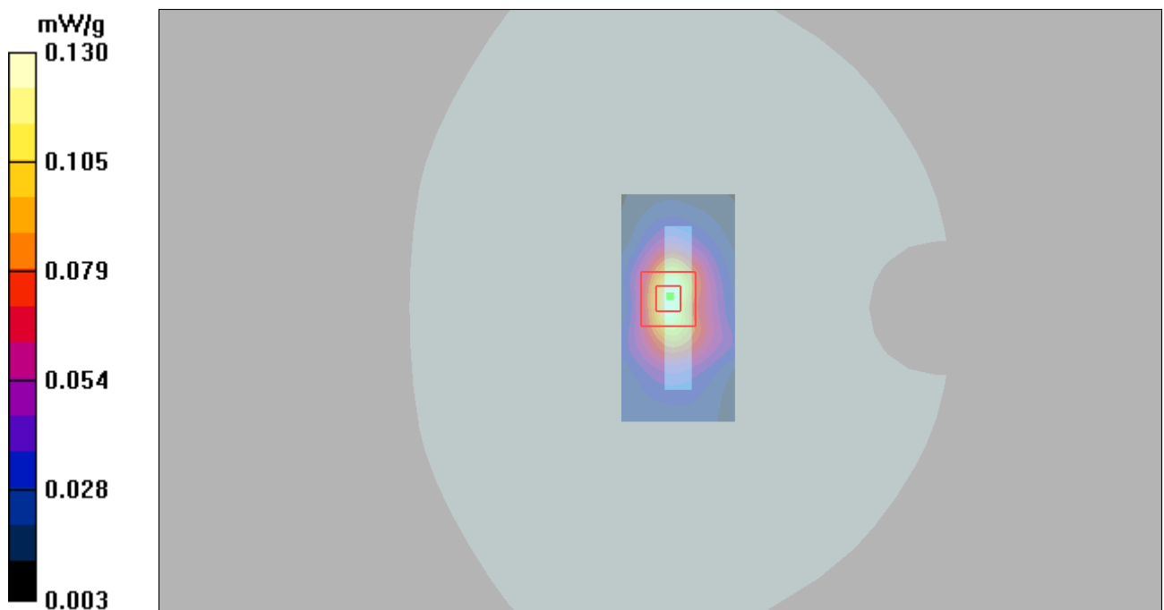
Figure 84 Body, Bottom Edge, UMTS Band V Channel 4183
