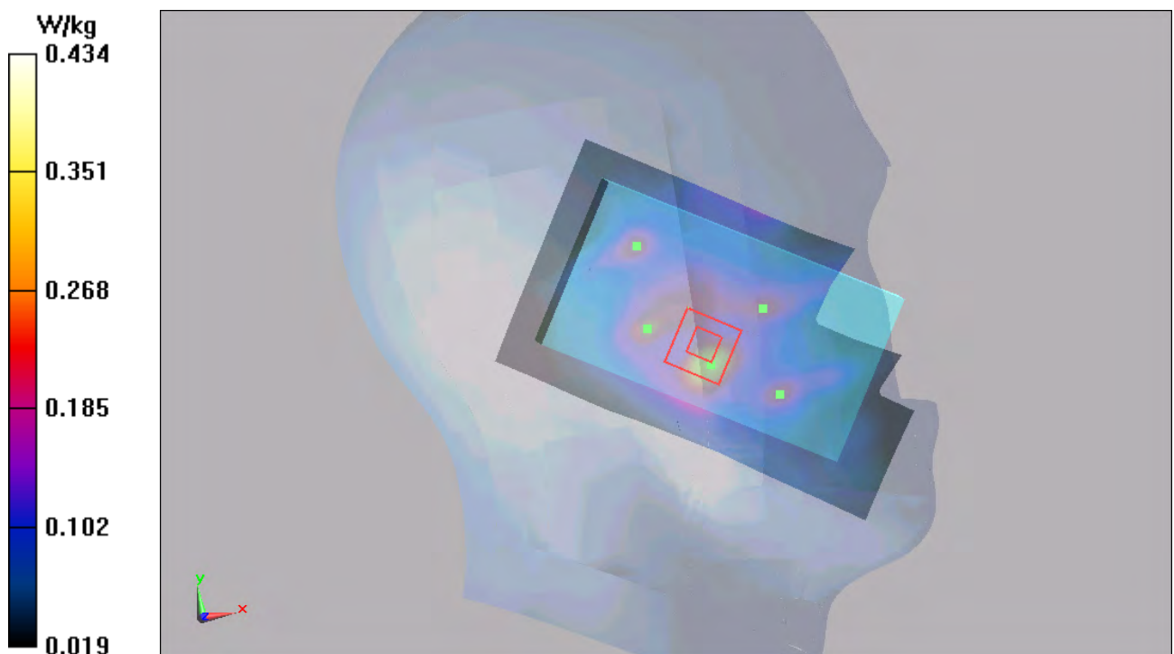
Figure 69 Left Hand Tilt 15° UMTS Band V Channel 4183
