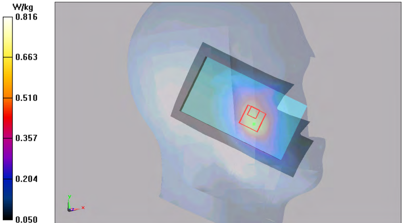
Figure 68 Left Hand Touch Cheek UMTS Band V Channel 4132
