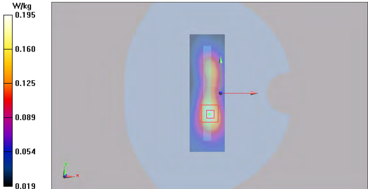
Figure 60 Body, Left Edge, UMTS Band II Channel 9400
