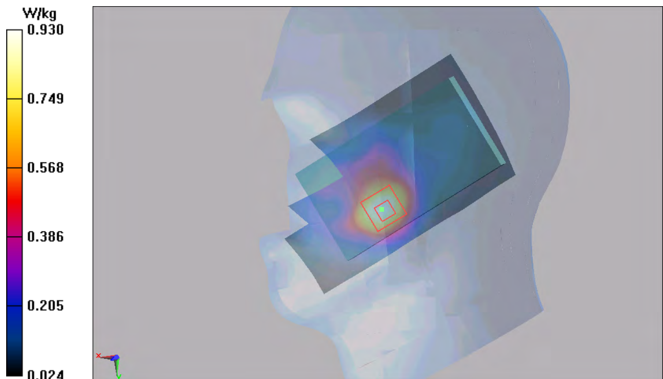
Figure 51 Right Hand Touch Cheek UMTS Band II Channel 9400
