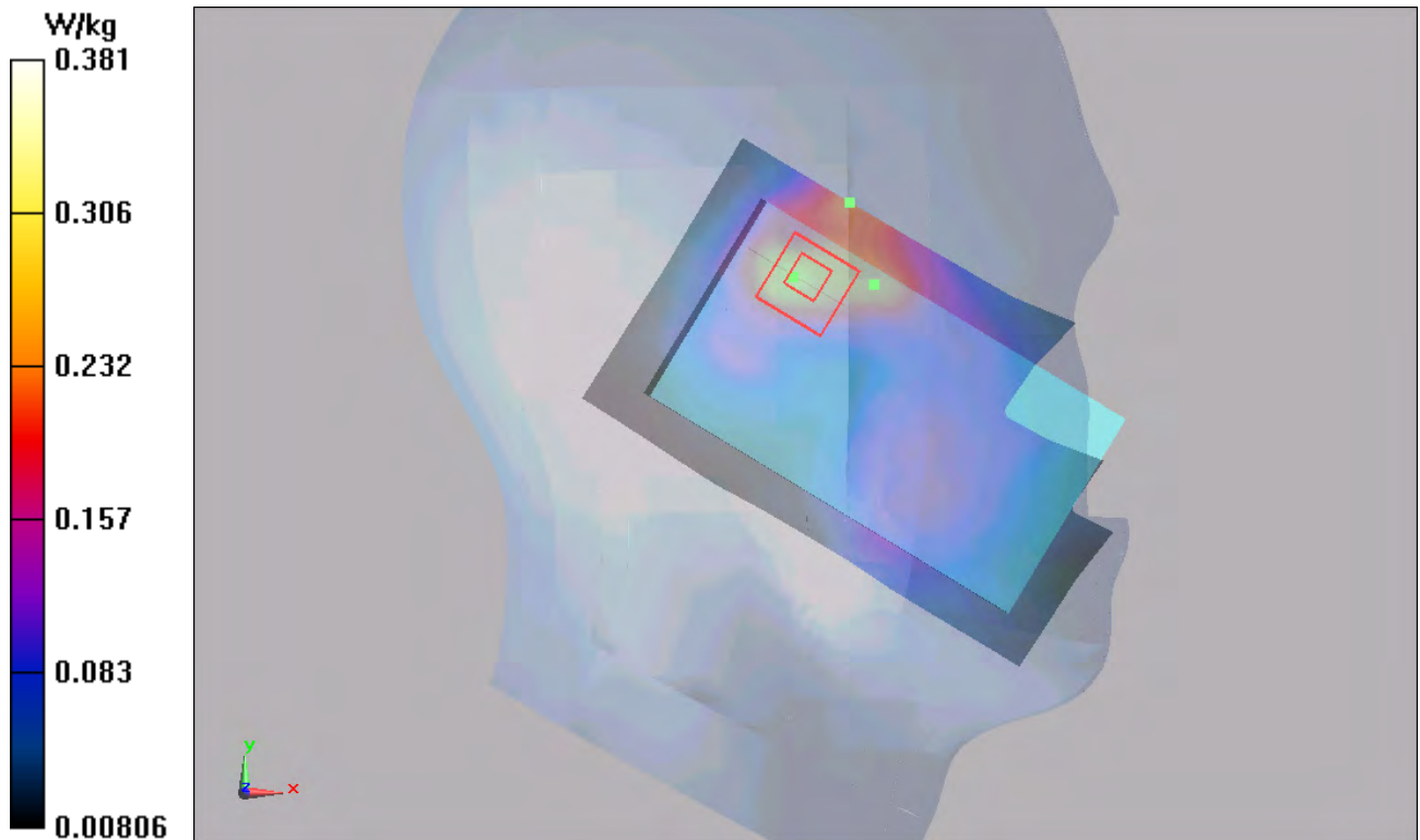
Figure 34 Left Hand Tilt 15° GSM 1900 Channel 661
