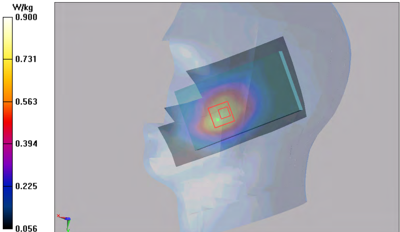
Figure 72 Left Hand Touch Cheek UMTS Band V Channel 4132
