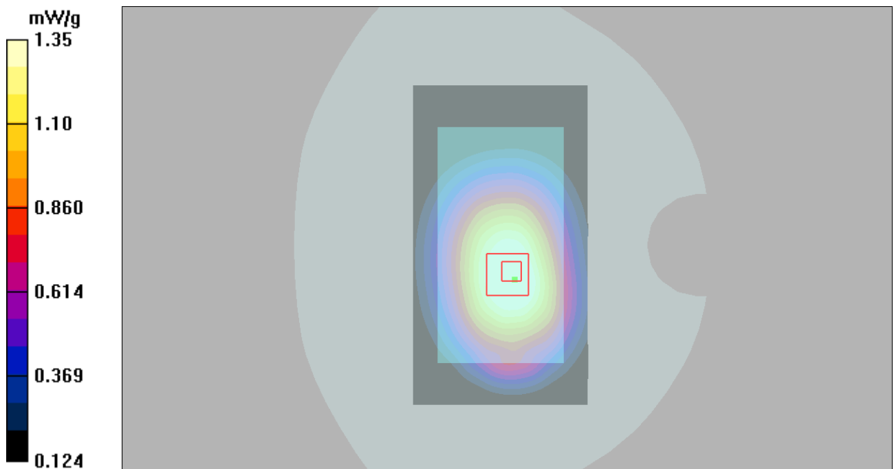
Figure 23 Body, Back Side, GSM 850 GPRS (4Txslots) Channel 190
