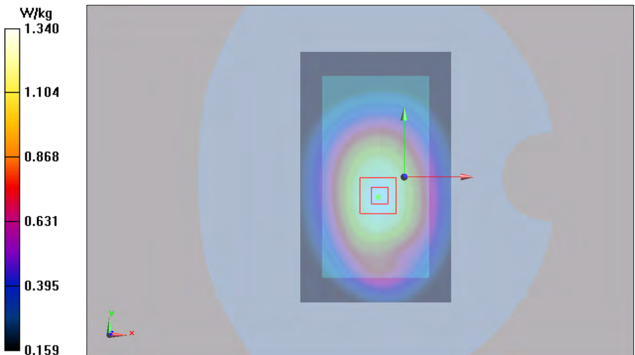
Figure 32 Body, Back Side, GSM 850 GPRS (4Txslots) Channel 190
