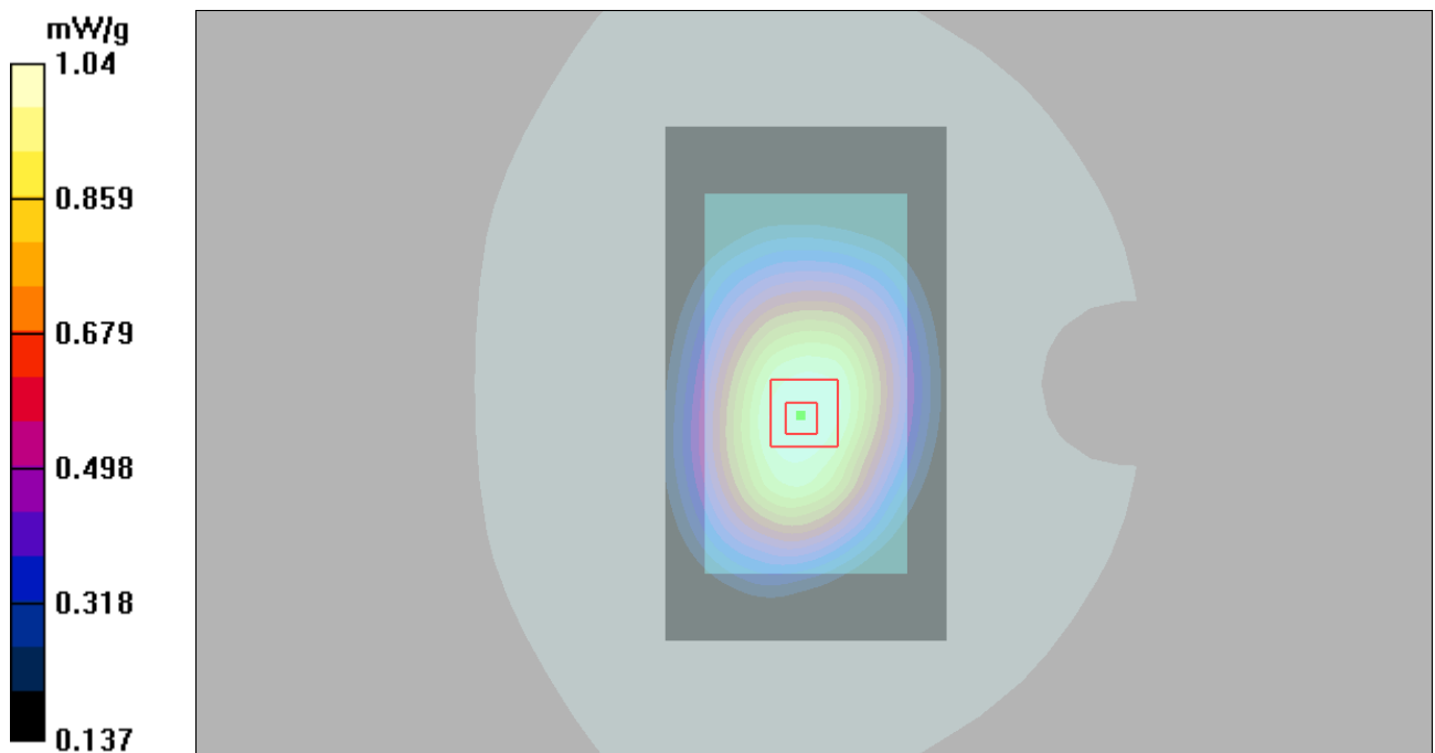
Figure 27 Body, Front Side, GSM 850 GPRS (4Txslots)Channel 128
