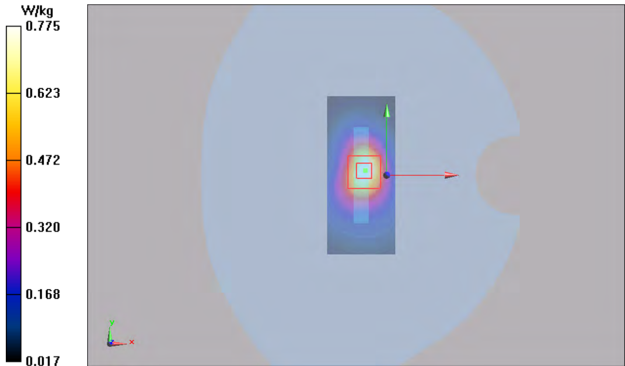
Figure 65 Body, Bottom Edge, UMTS Band II Channel 9400
