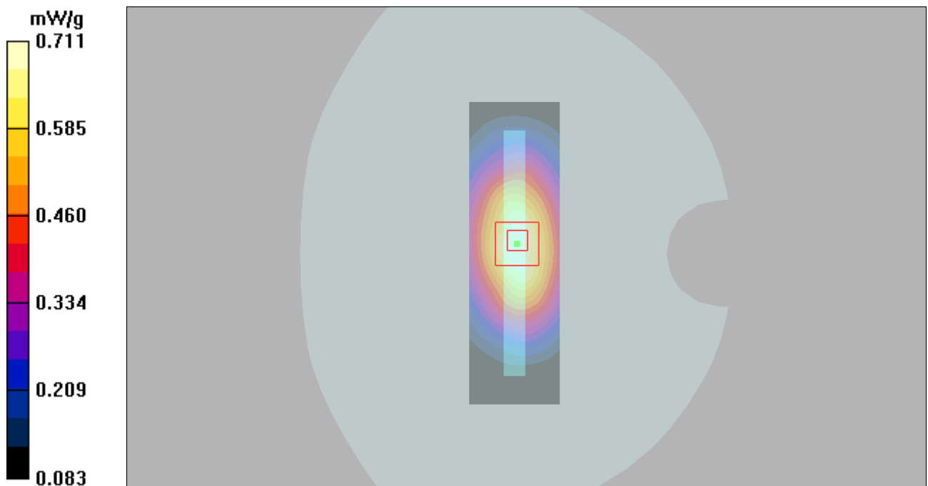
Figure 29 Body, Right Edge, GSM 850 GPRS (4Txslots)Channel 190
