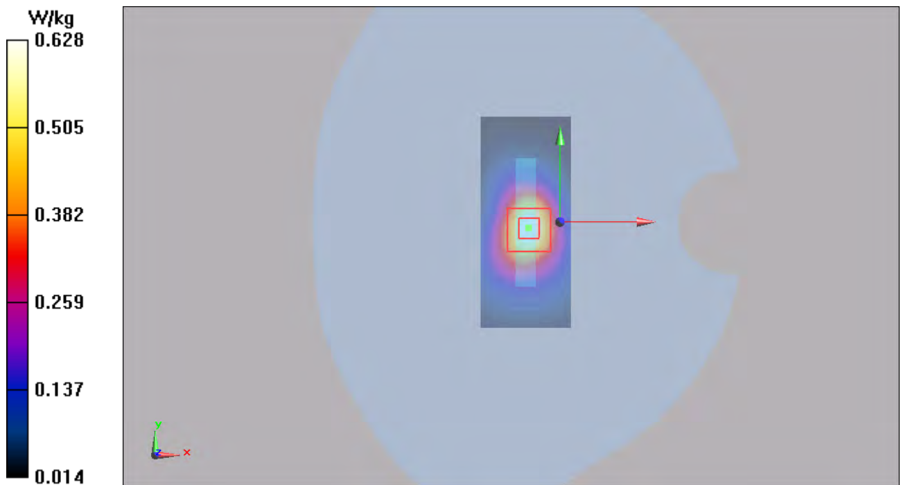
Figure 46 Body, Bottom Edge, GSM 1900 GPRS (4Txslots) Channel 512
