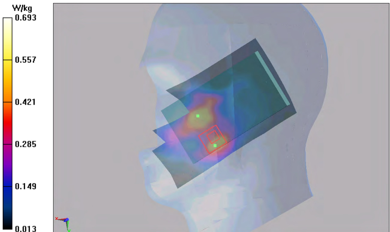
Figure 35 Right Hand Touch Cheek GSM 1900 Channel 661
