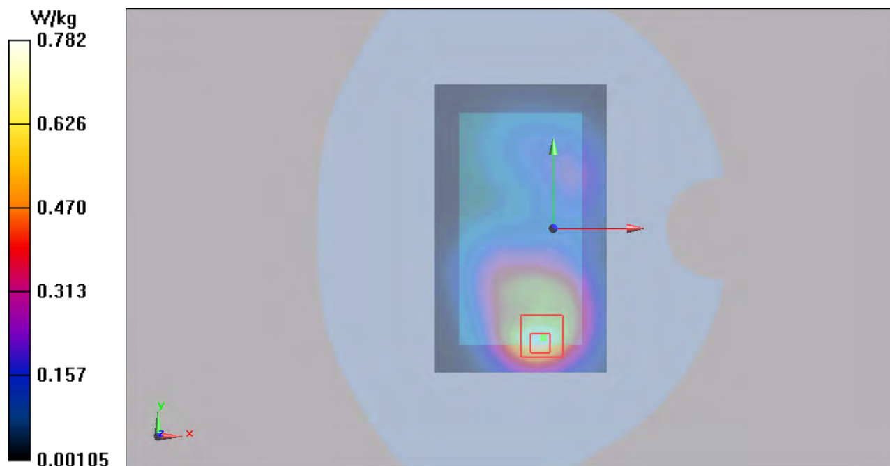
Figure 57 Body, Front Side, UMTS Band II Channel 9538
