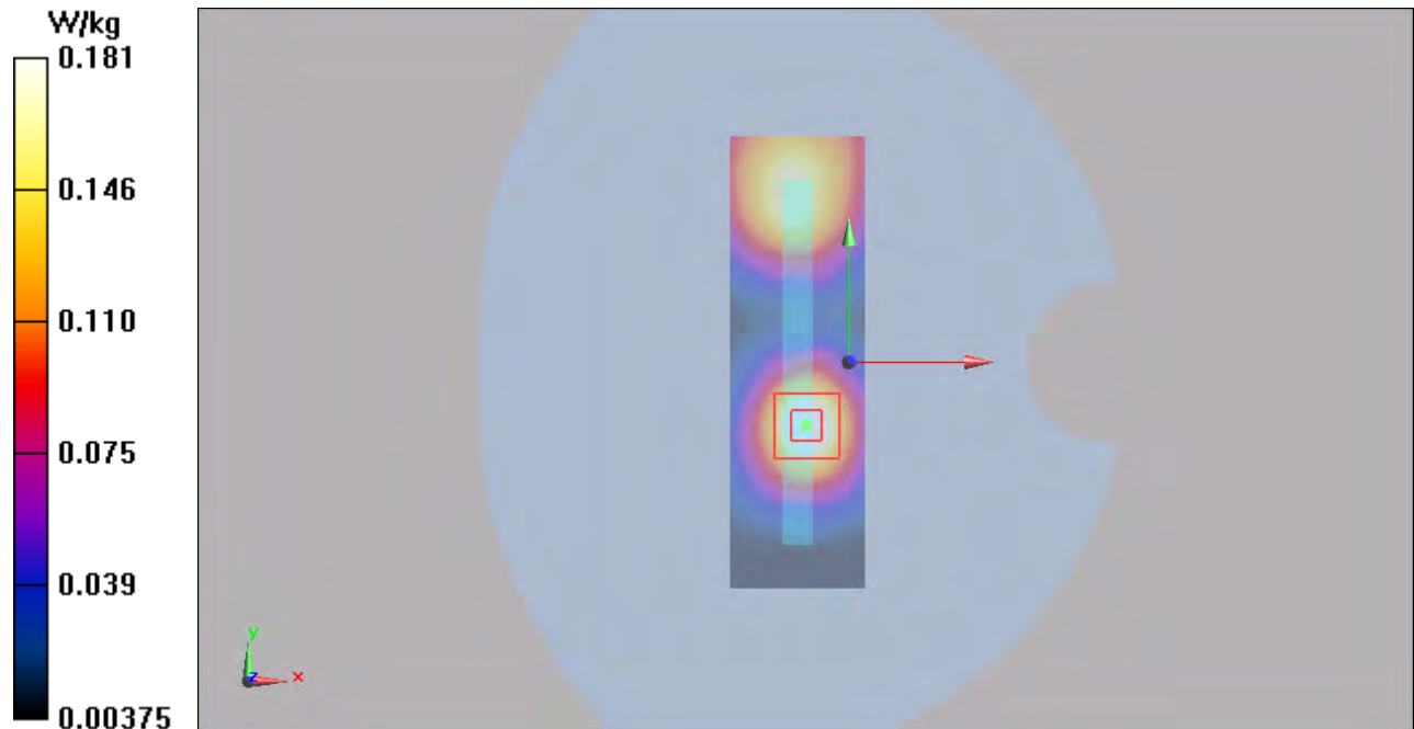
Figure 61 Body, Right Edge, UMTS Band II Channel 9400
