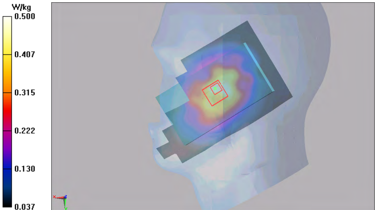
Figure 18 Right Hand Tilt 15° GSM 850 Channel 190
