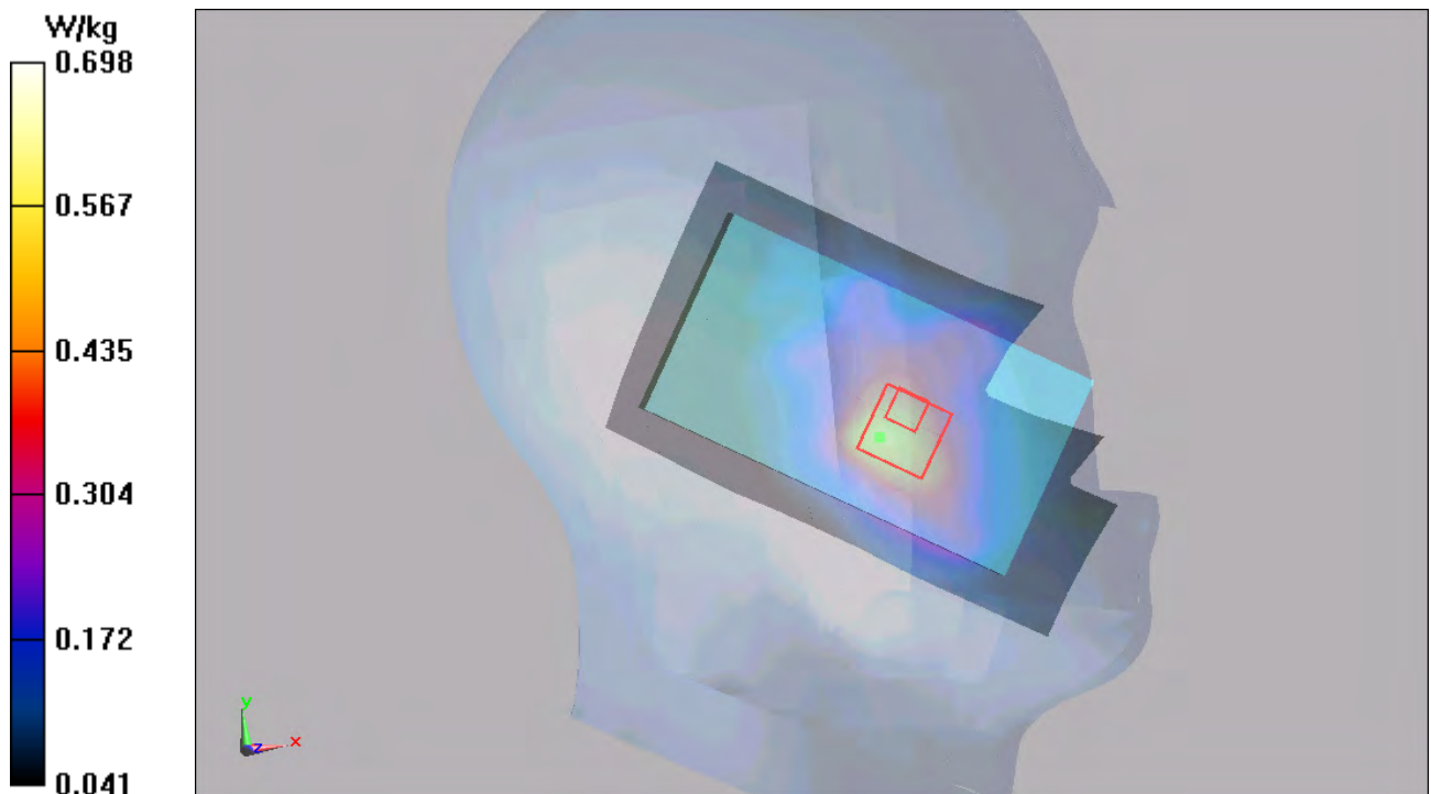
Figure 66 Left Hand Touch Cheek UMTS Band V Channel 4233
