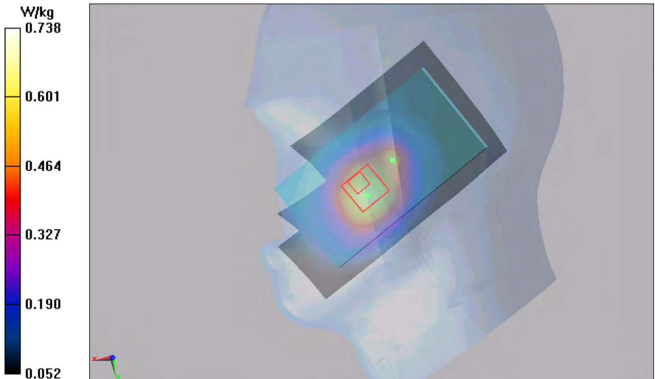
Figure 70 Right Hand Touch Cheek UMTS Band V Channel 4233
