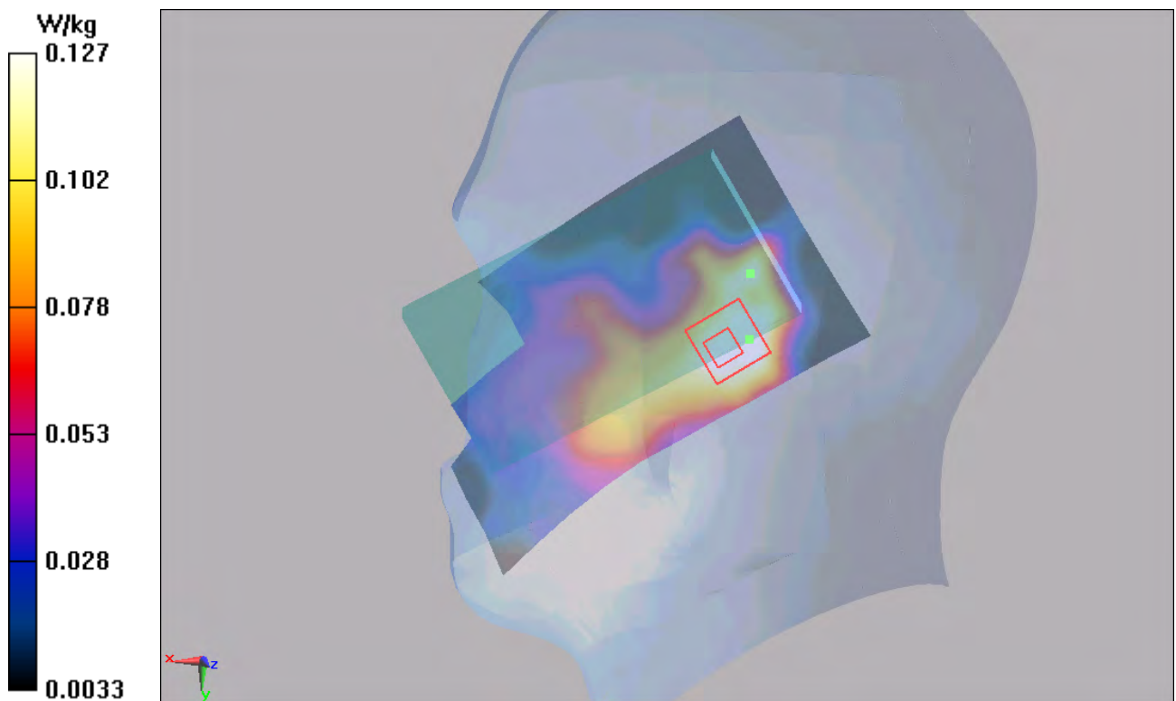
Figure 36 Right Hand Tilt 15° GSM 1900 Channel 661
