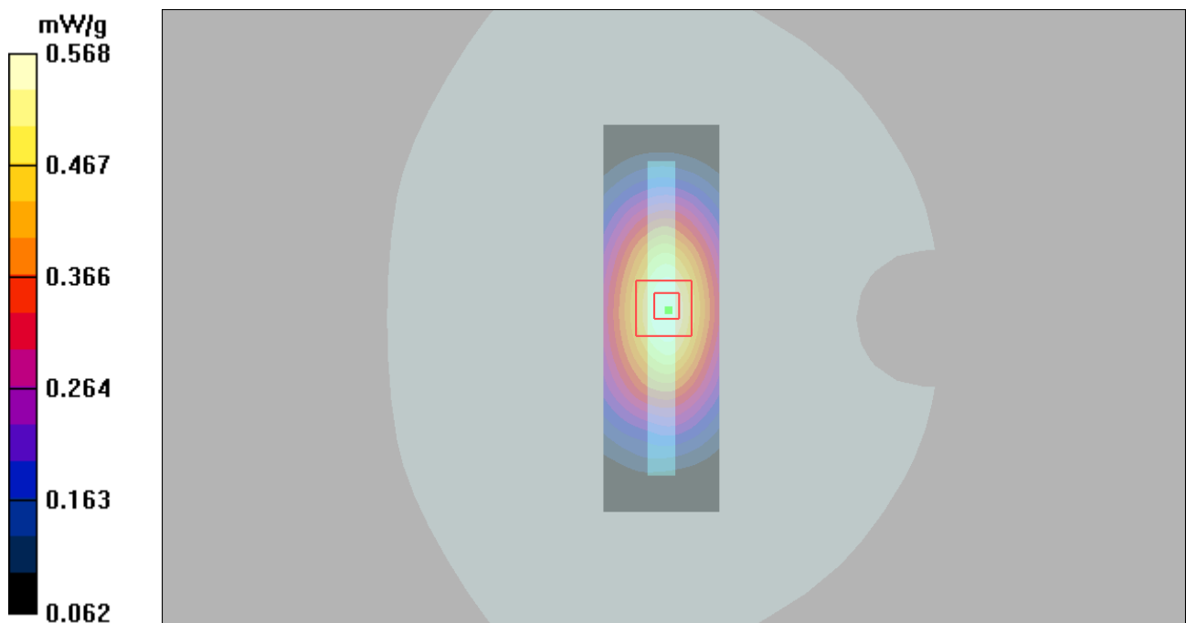
Figure 28 Body, Left Edge, GSM 850 GPRS (4Txslots)Channel 190
