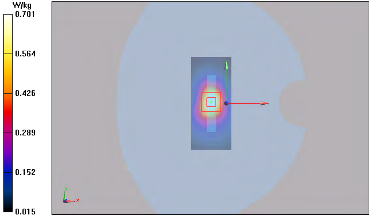
Figure 62 Body, Bottom Edge, UMTS Band II Channel 9538
