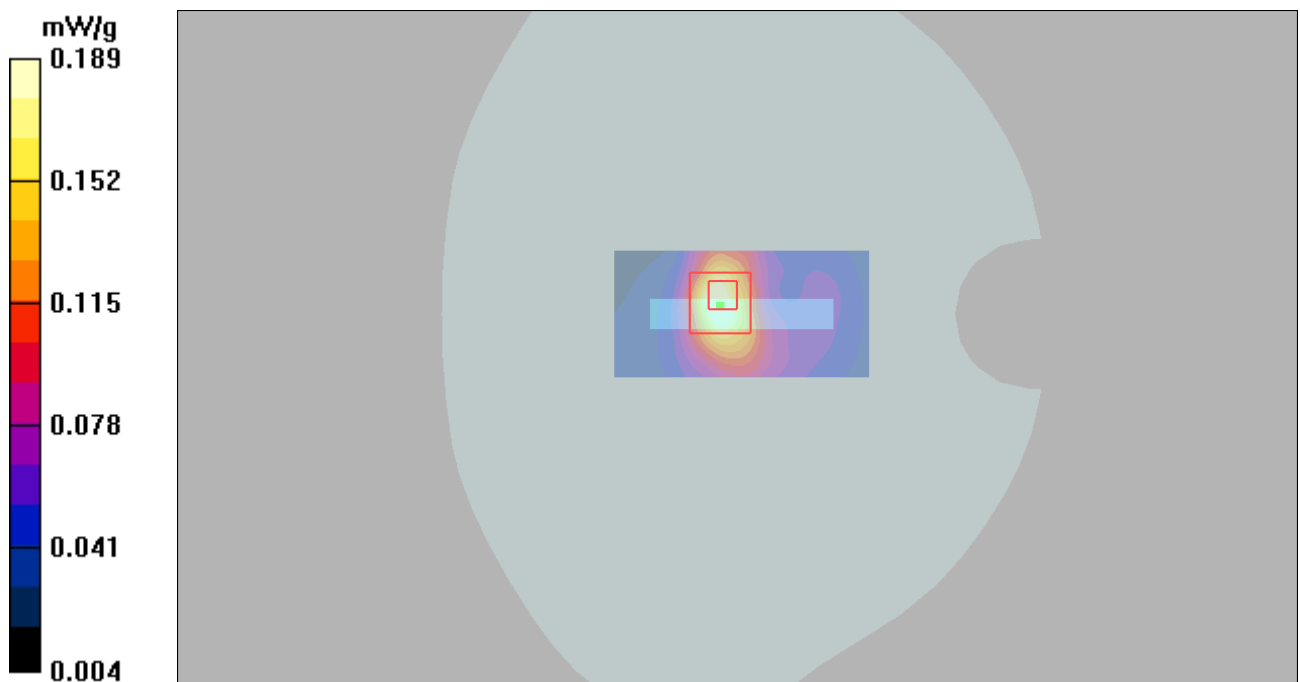
Figure 30 Body, Bottom Edge, GSM 850 GPRS (4Txslots)annel 190
