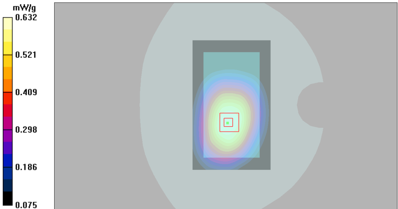
Figure 80 Body, Front Side, UMTS Band V Channel 4183
