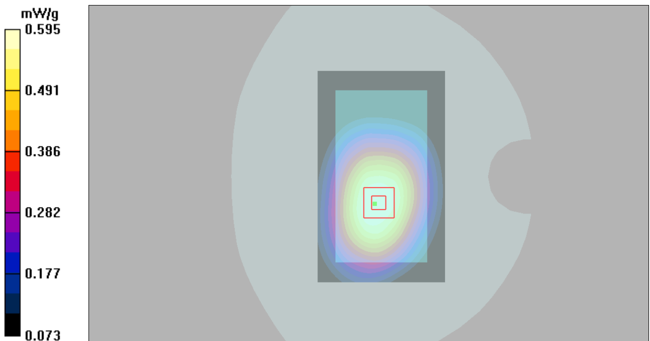
Figure 79 Body, Front Side, UMTS Band V Channel 4233
