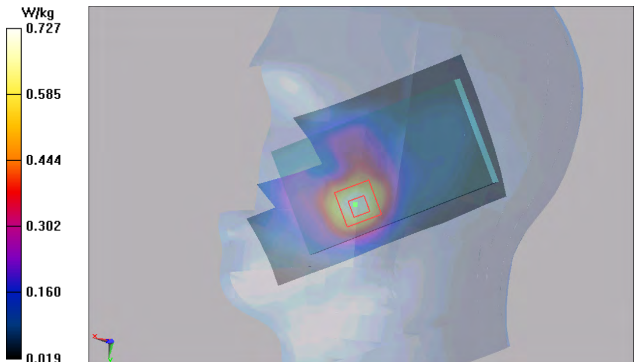
Figure 52 Right Hand Touch Cheek UMTS Band II Channel 9262
