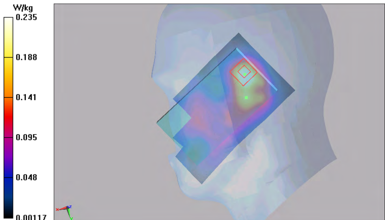
Figure 53 Right Hand Tilt 15° UMTS Band II Channel 9400
