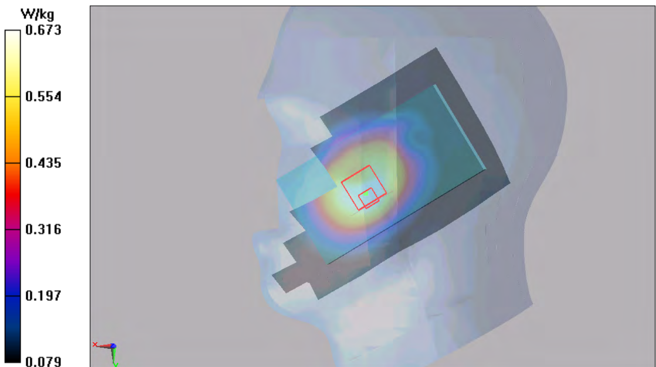
Figure 17 Right Hand Touch Cheek GSM 850 Channel 190
