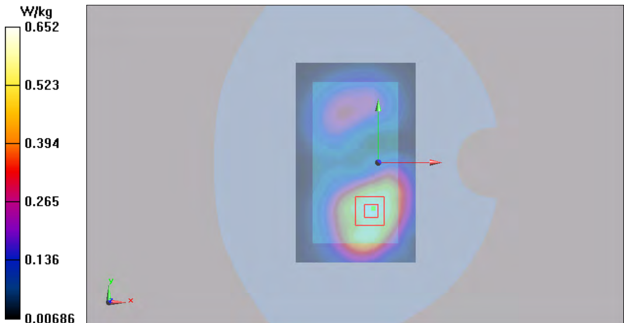
Figure 56 Body, Back Side, UMTS Band II Channel 9400
