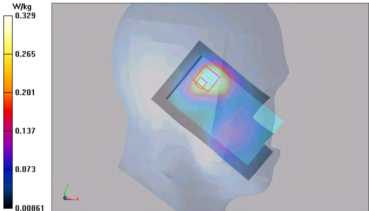
Figure 49 Left Hand Tilt 15° UMTS Band II Channel 9400
