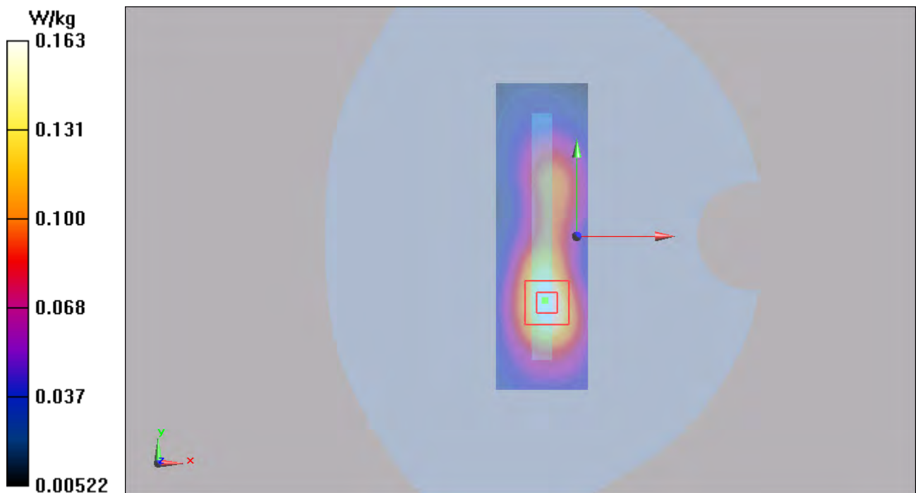
Figure 42 Body, Left Edge, GSM 1900 GPRS (4Txslots) Channel 661
