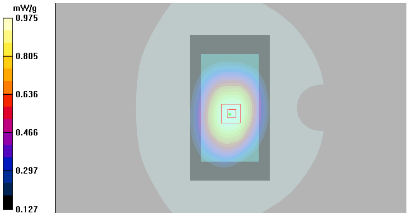
Figure 25 Body, Front Side, GSM 850 GPRS (4Txslots)Channel 251
