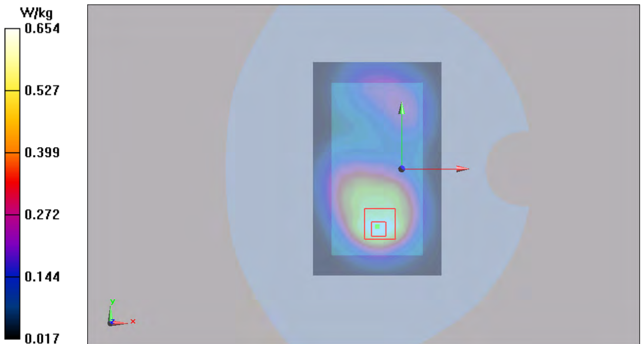
Figure 41 Body, Front Side, GSM 1900 GPRS (4Txslots) Channel 661
