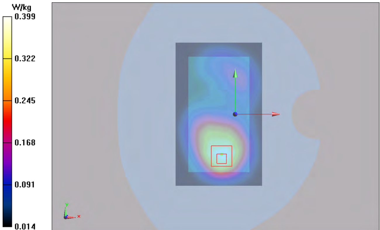
Figure 39 Body, Front Side, GSM 1900 Channel 661
