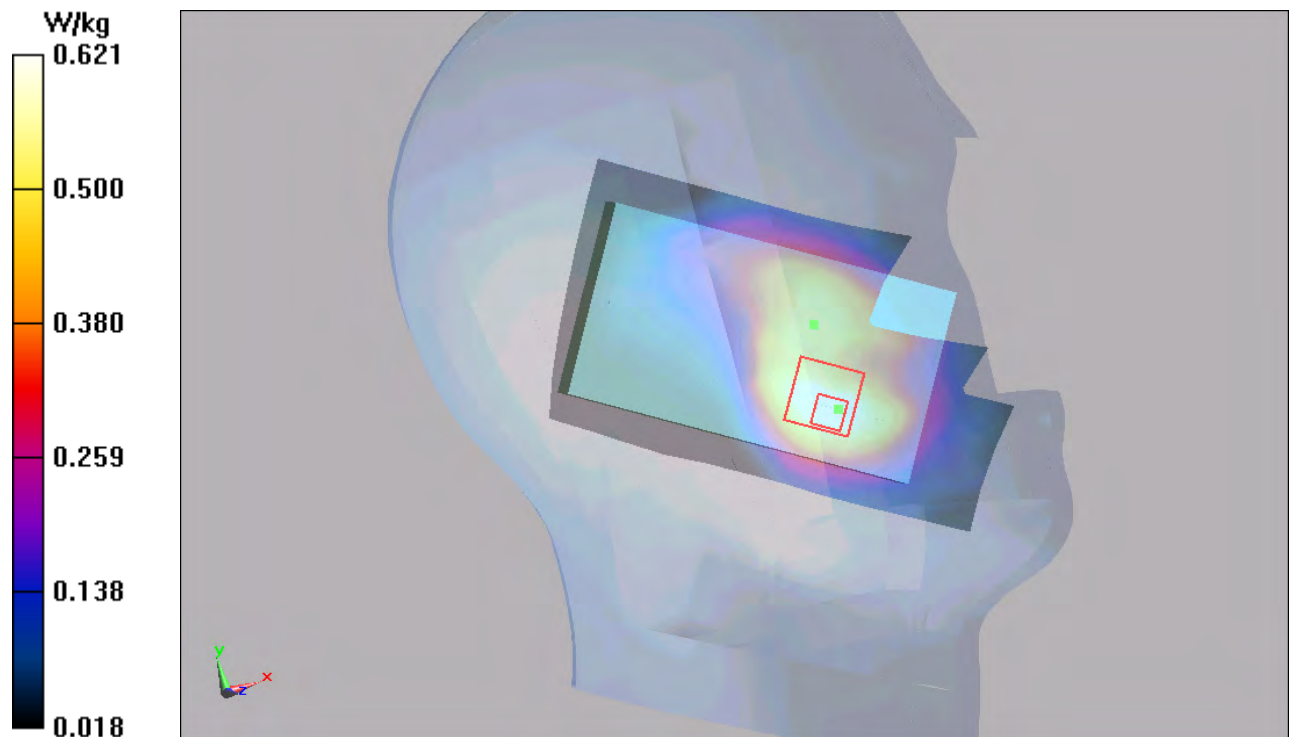
Figure 48 Left Hand Touch Cheek UMTS Band II Channel 9400
