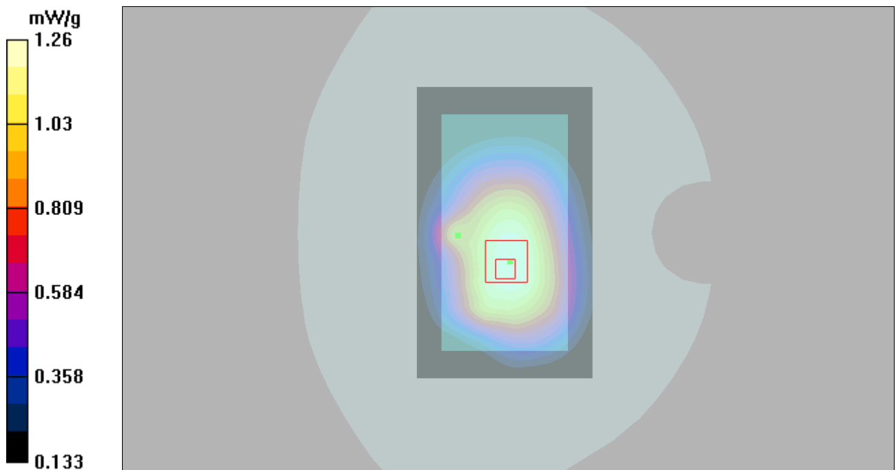
Figure 24 Body, Back Side, GSM 850 GPRS (4Txslots) Channel 128
