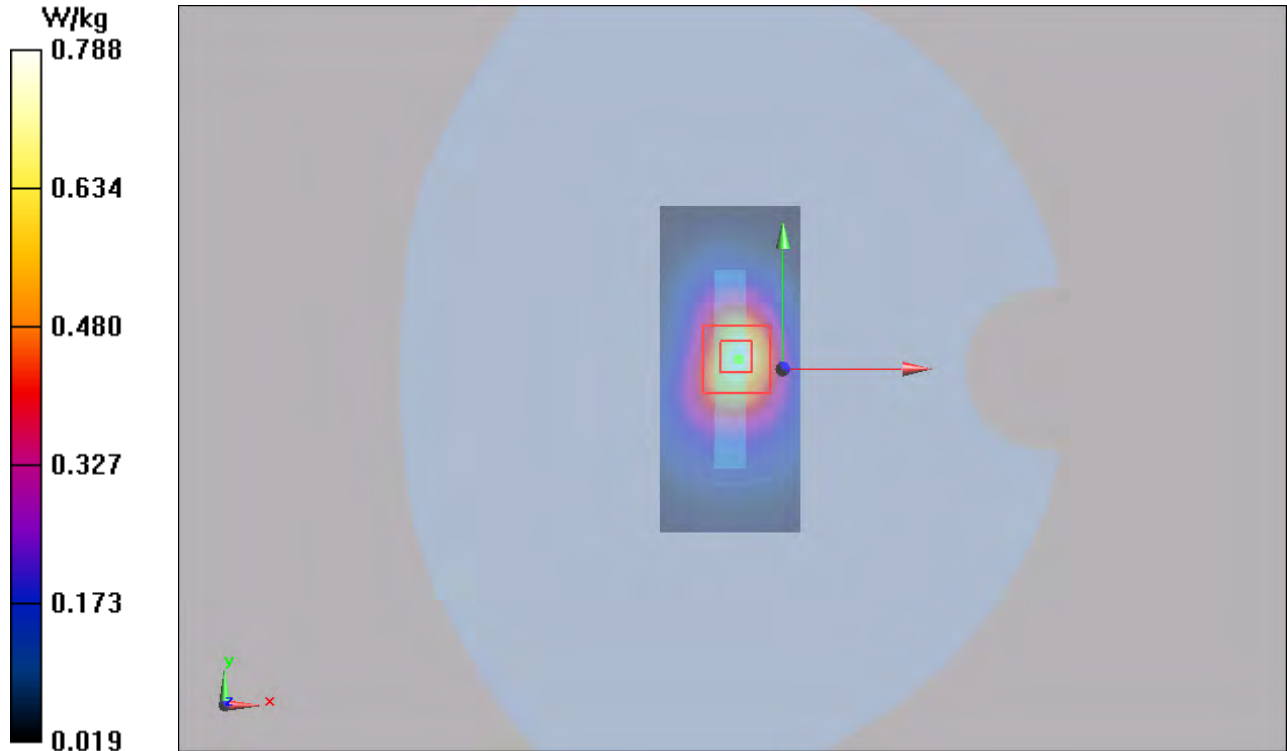
Figure 64 Body, Bottom Edge, UMTS Band II Channel 9262
