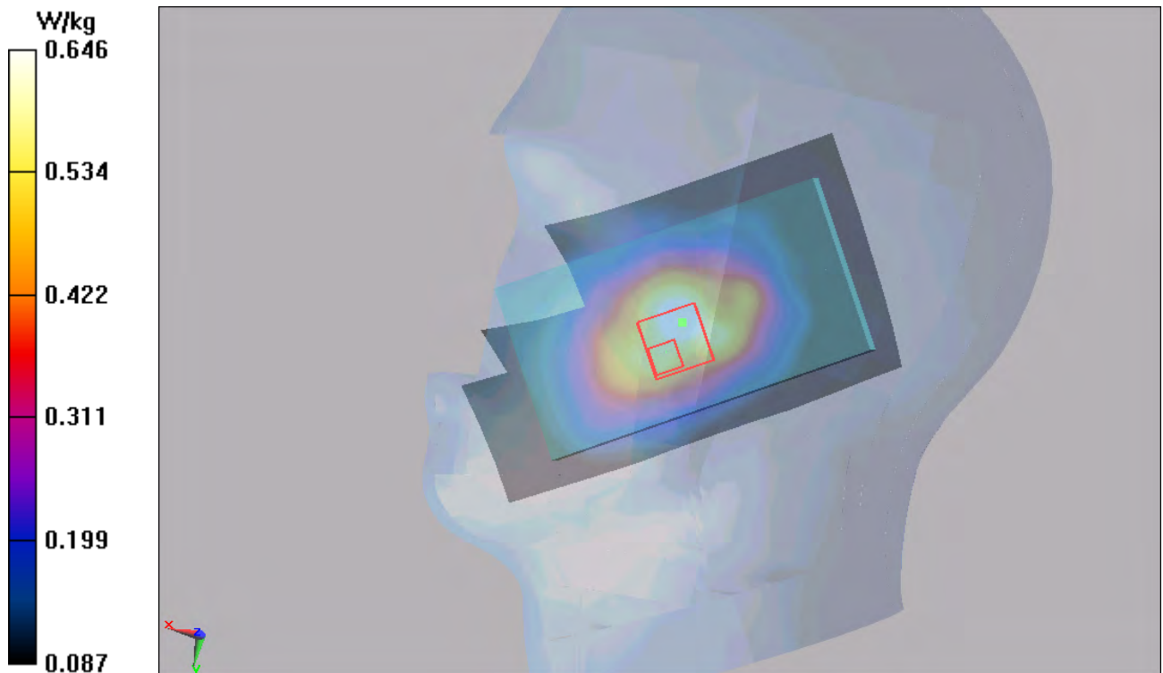
Figure 74 Left Touch Cheek UMTS Band V Channel 4132
