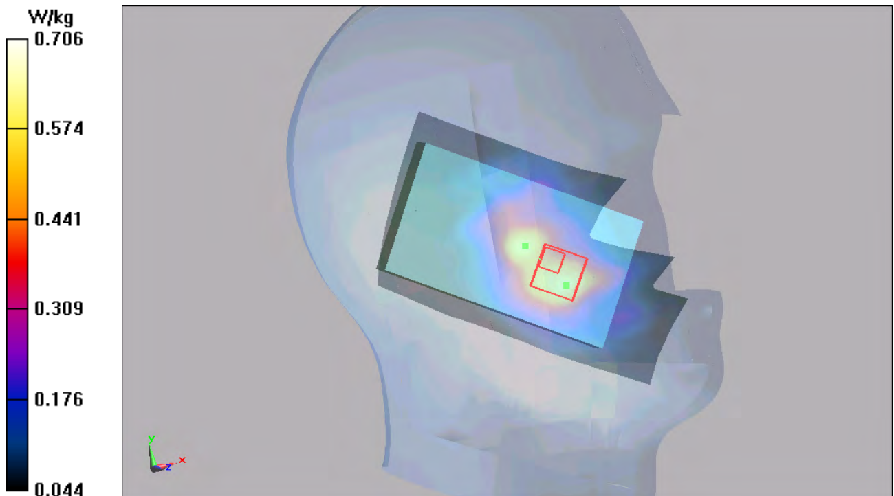
Figure 67 Left Hand Touch Cheek UMTS Band V Channel 4183
