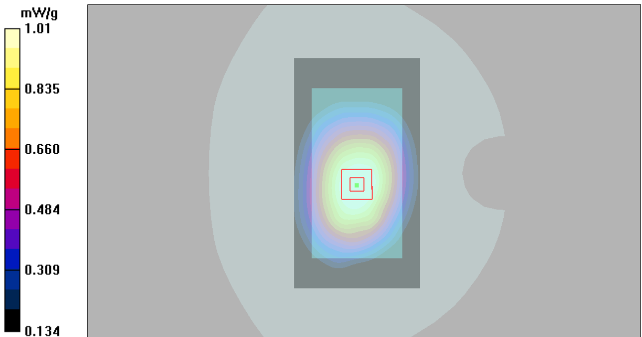
Figure 26 Body, Front Side, GSM 850 GPRS (4Txslots)Channel 190
