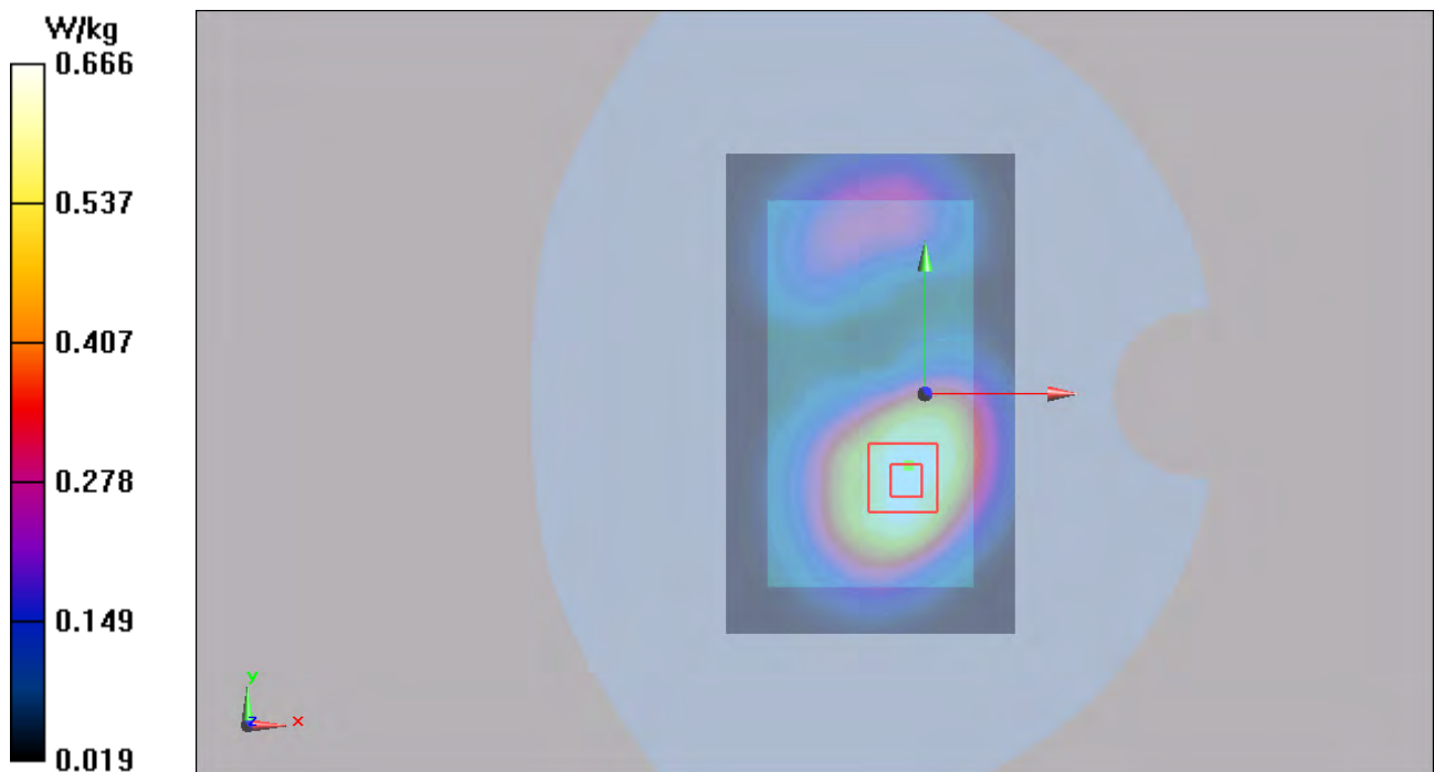
Figure 40 Body, Back Side, GSM 1900 GPRS (4Txslots) Channel 661
