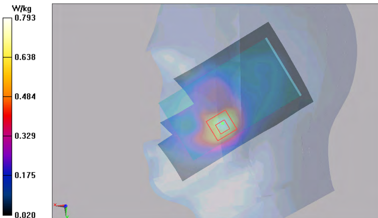
Figure 55 Body, Right Cheek, UMTS Band II Channel 9400
