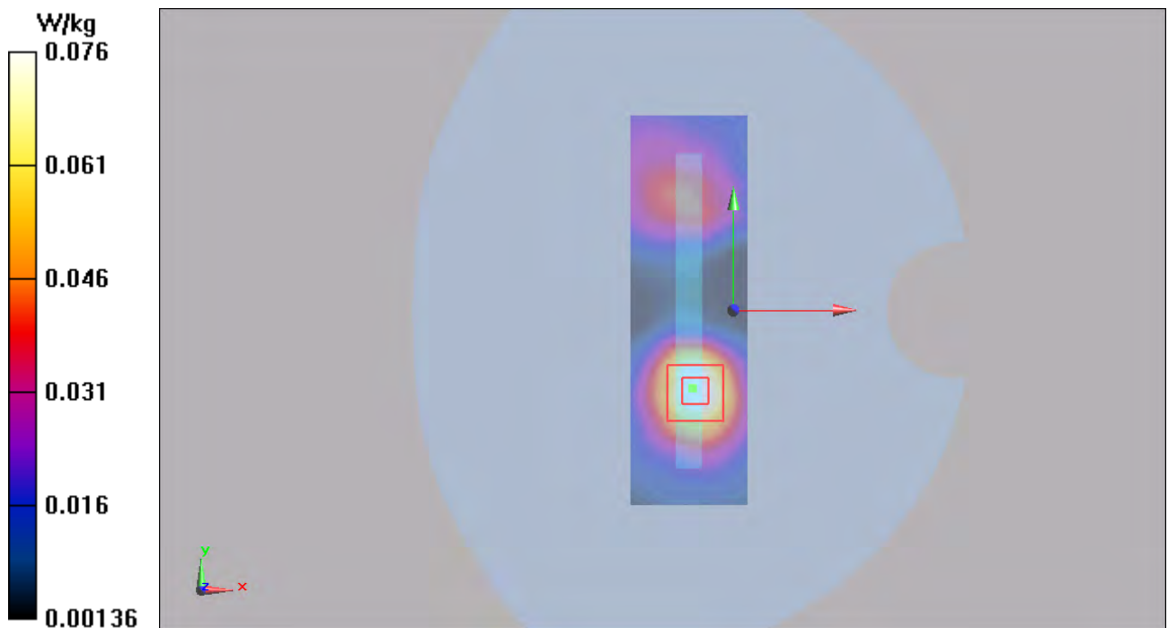
Figure 43 Body, Right Edge, GSM 1900 GPRS (4Txslots) Channel 661
