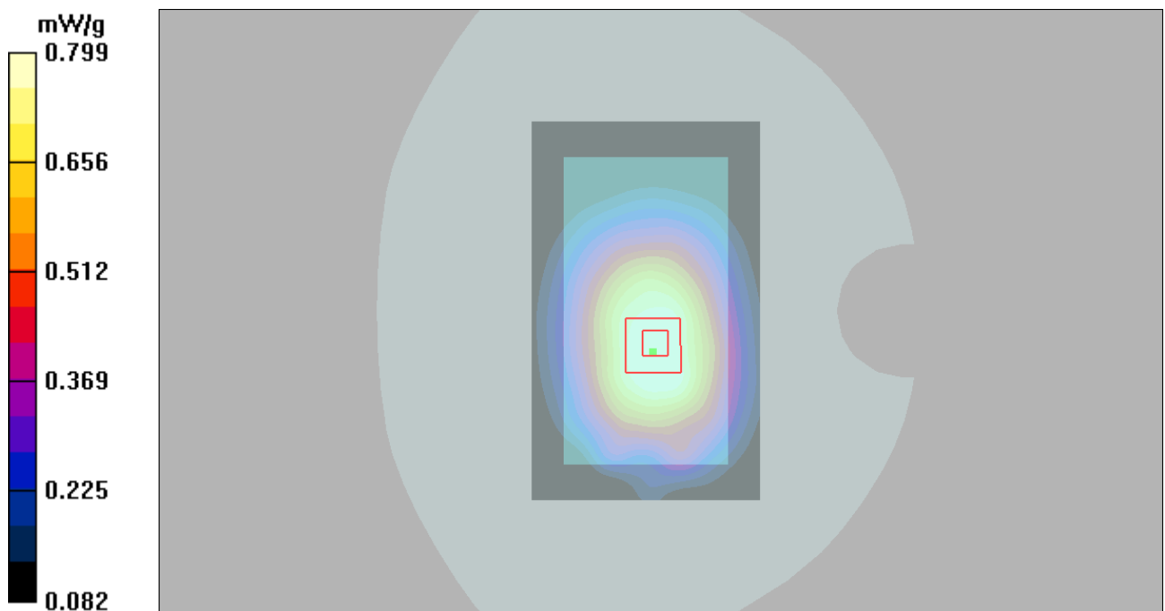
Figure 76 Body, Back Side, UMTS Band V Channel 4233
