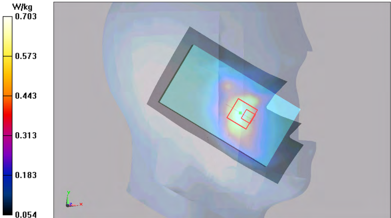
Figure 19 Left Hand Touch Cheek GSM 850 Channel 190
