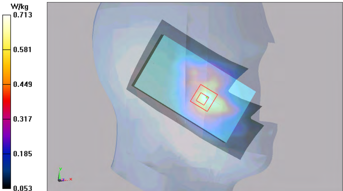
Figure 15 Left Hand Touch Cheek GSM 850 Channel 190
