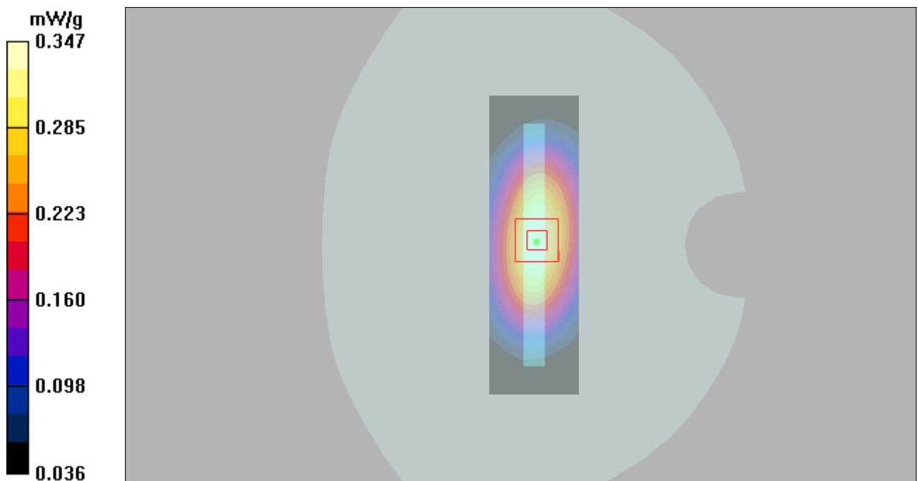
Figure 82 Body, Left Edge, UMTS Band V Channel 4183
