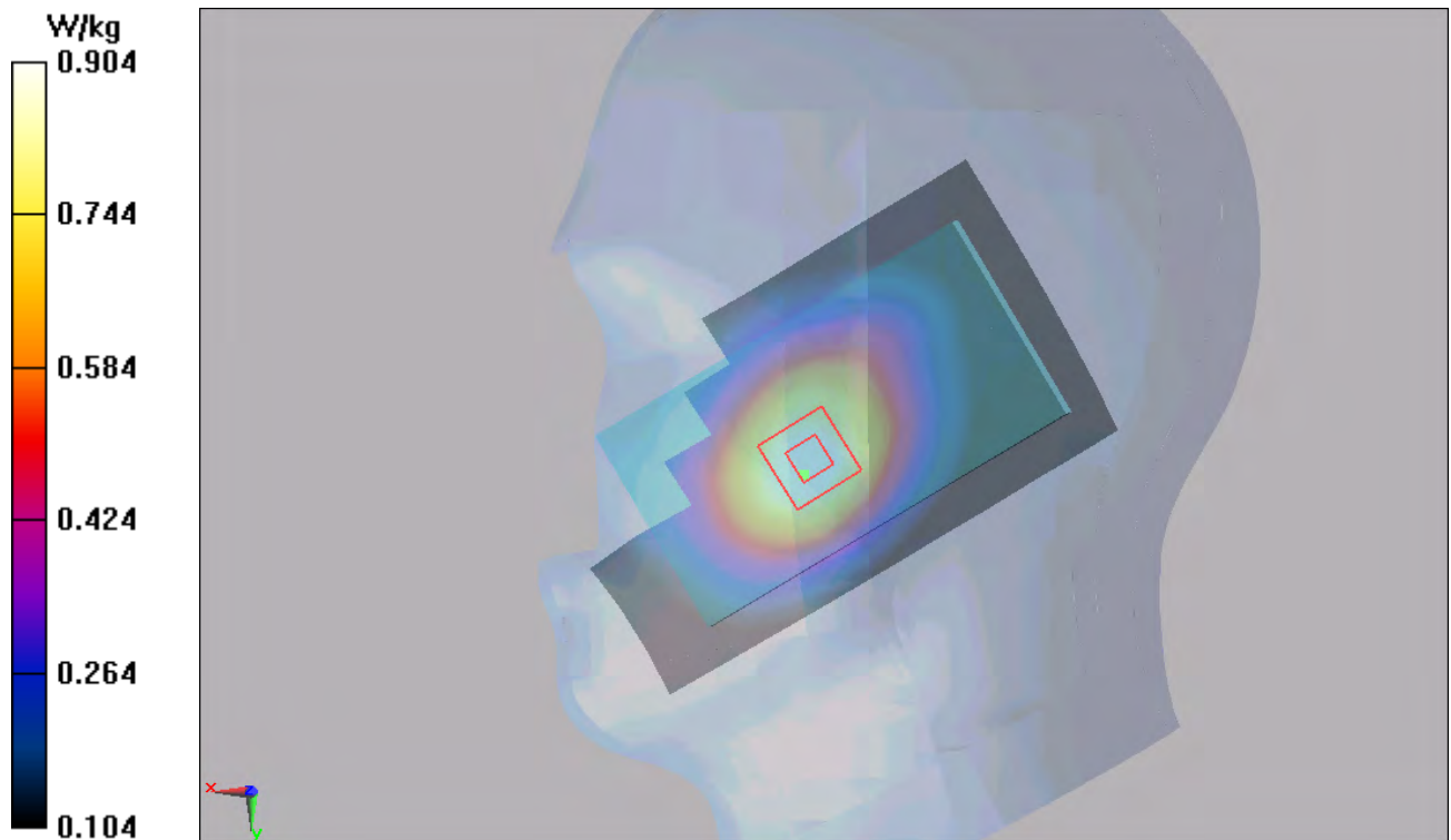
Figure 75 Body, Right Cheek, UMTS Band V Channel 4132
