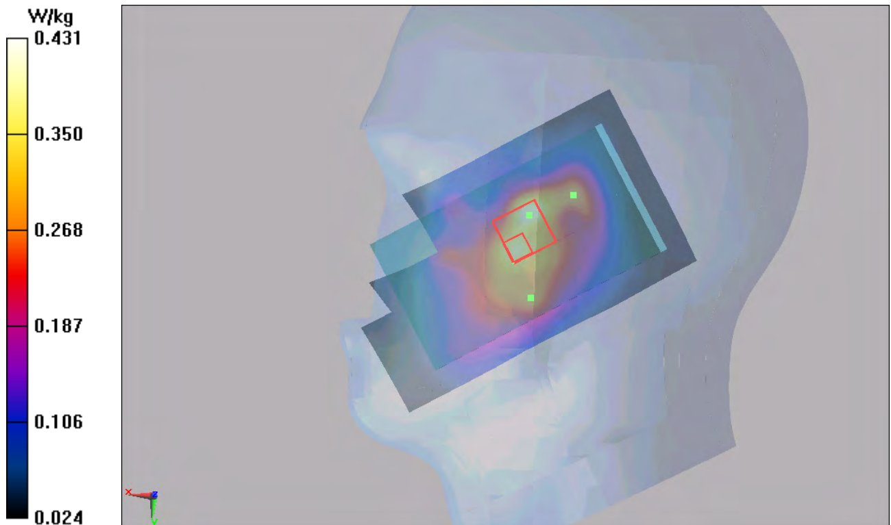
Figure 73 Right Hand Tilt 15° UMTS Band V Channel 4183
