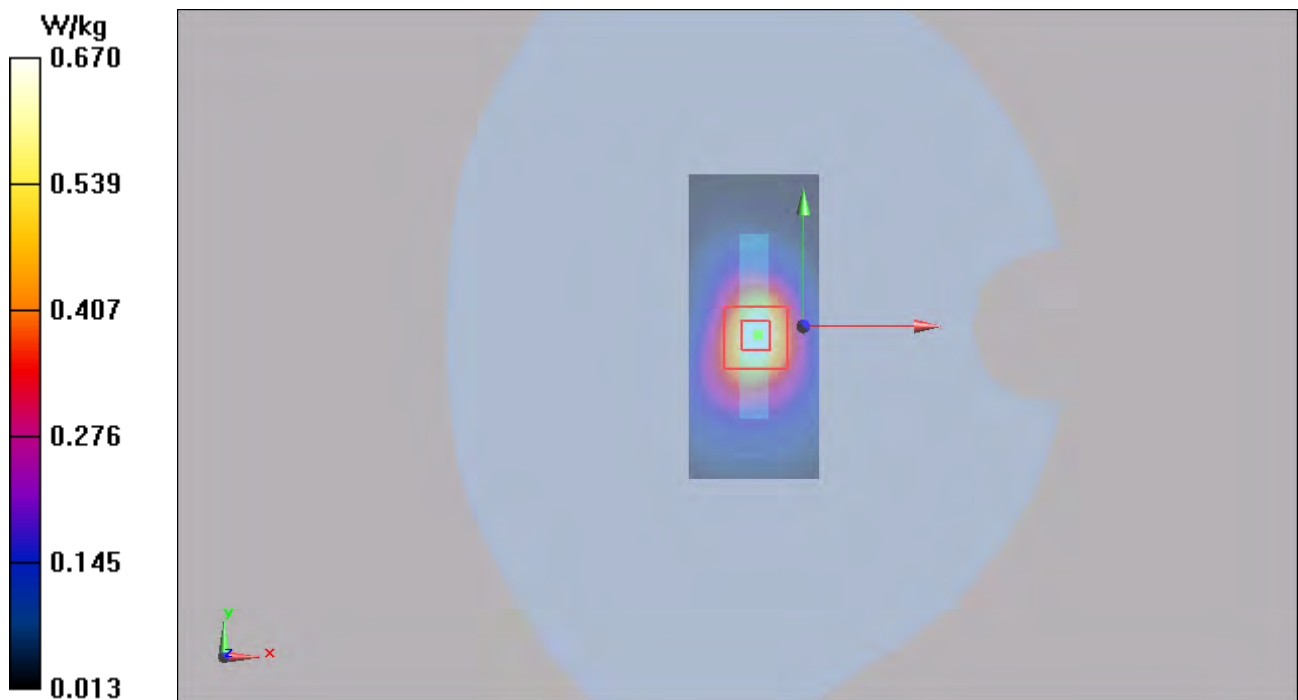
Figure 45 Body, Bottom Edge, GSM 1900 GPRS (4Txslots) Channel 661
