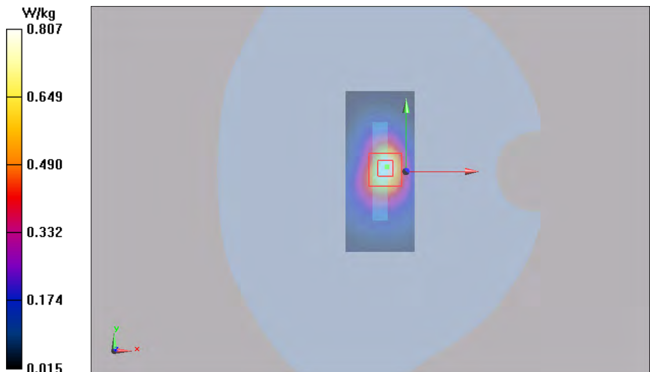
Figure 63 Body, Bottom Edge, UMTS Band II Channel 9400
