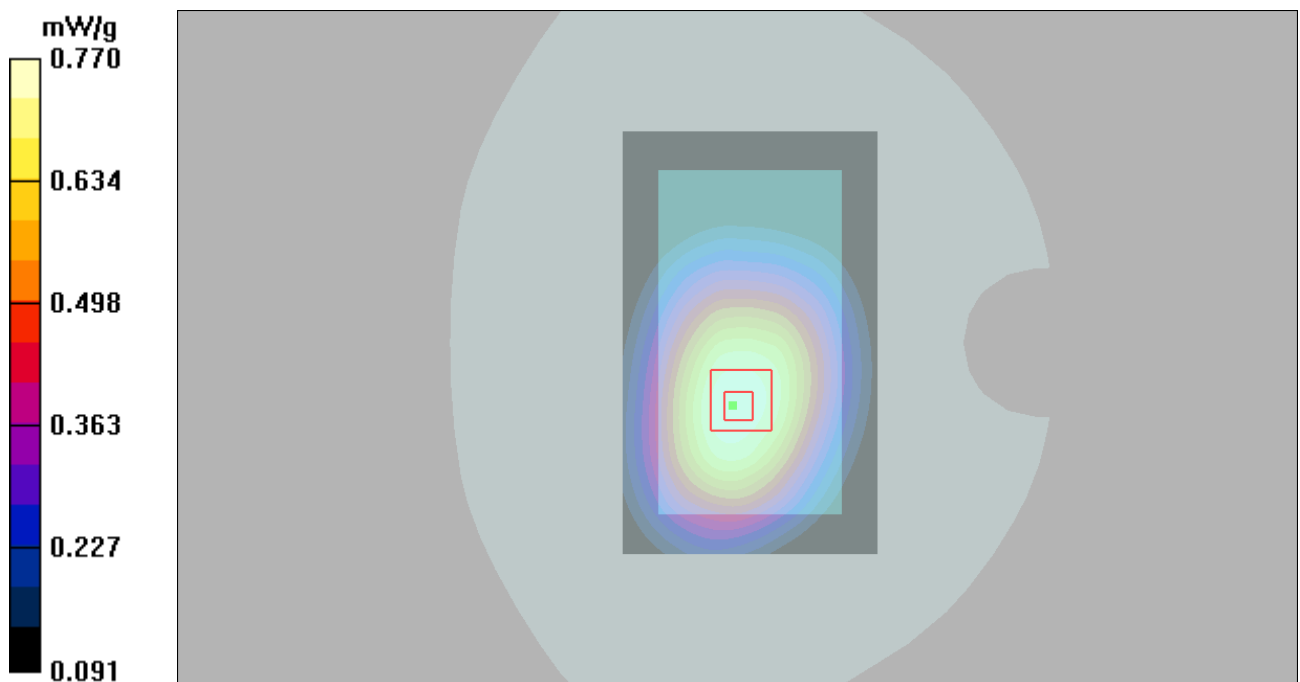
Figure 81 Body, Front Side, UMTS Band V Channel 4132
