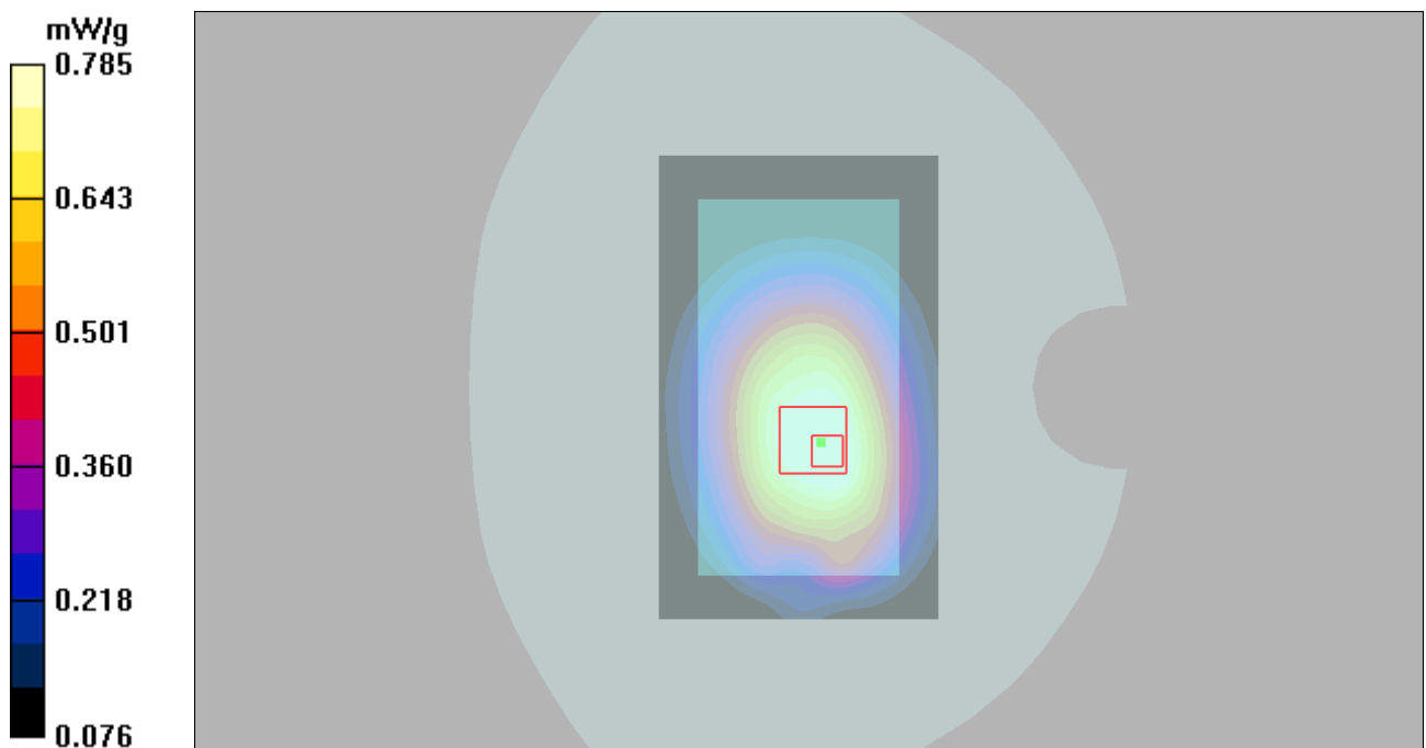
Figure 78 Body, Back Side, UMTS Band V Channel 4132
