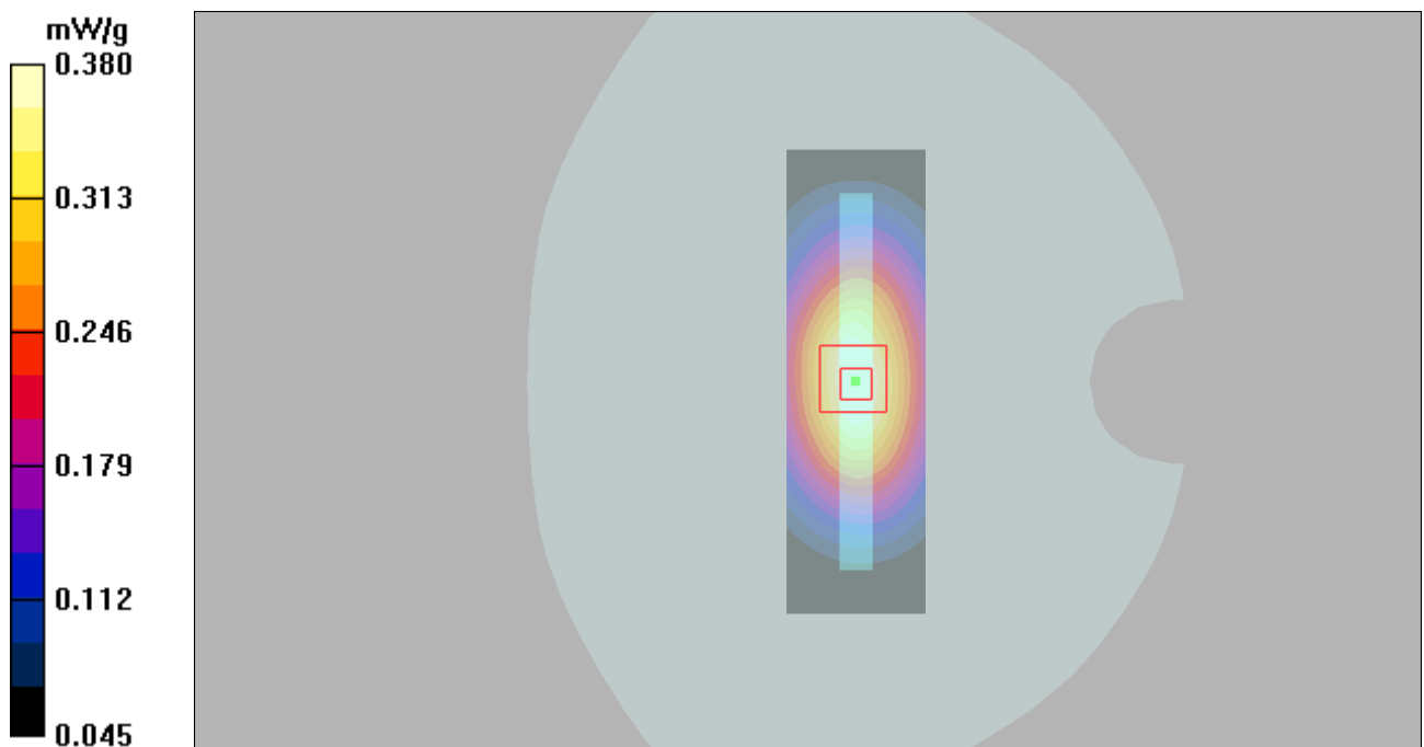
Figure 83 Body, Right Edge, UMTS Band V Channel 4183
