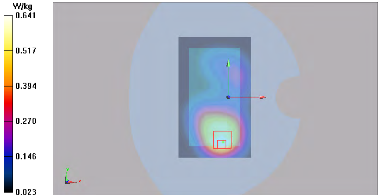
Figure 59 Body, Front Side, UMTS Band II Channel 9262
