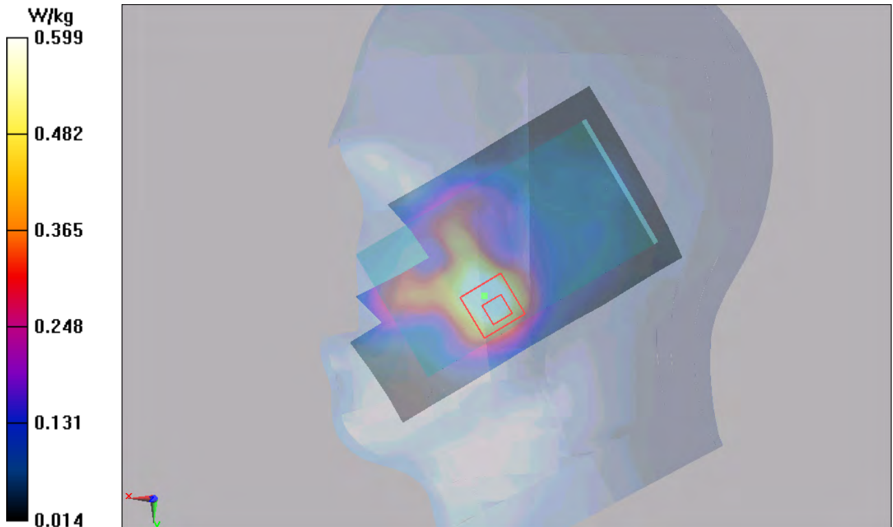
Figure 37 Right Hand Touch Cheek GSM 1900 Channel 661
