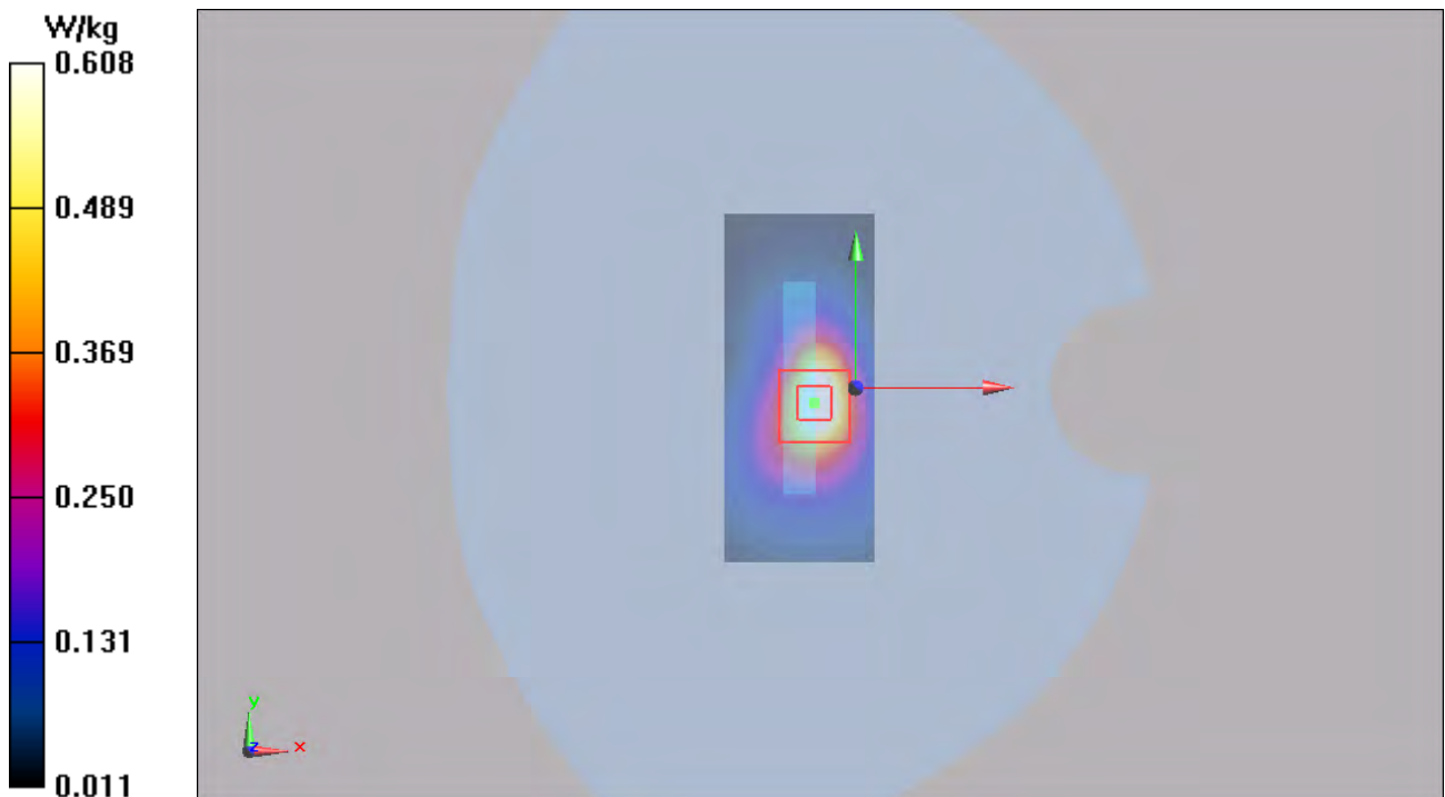
Figure 47 Body, Bottom Edge, GSM 1900 GPRS (4Txslots) Channel 810
