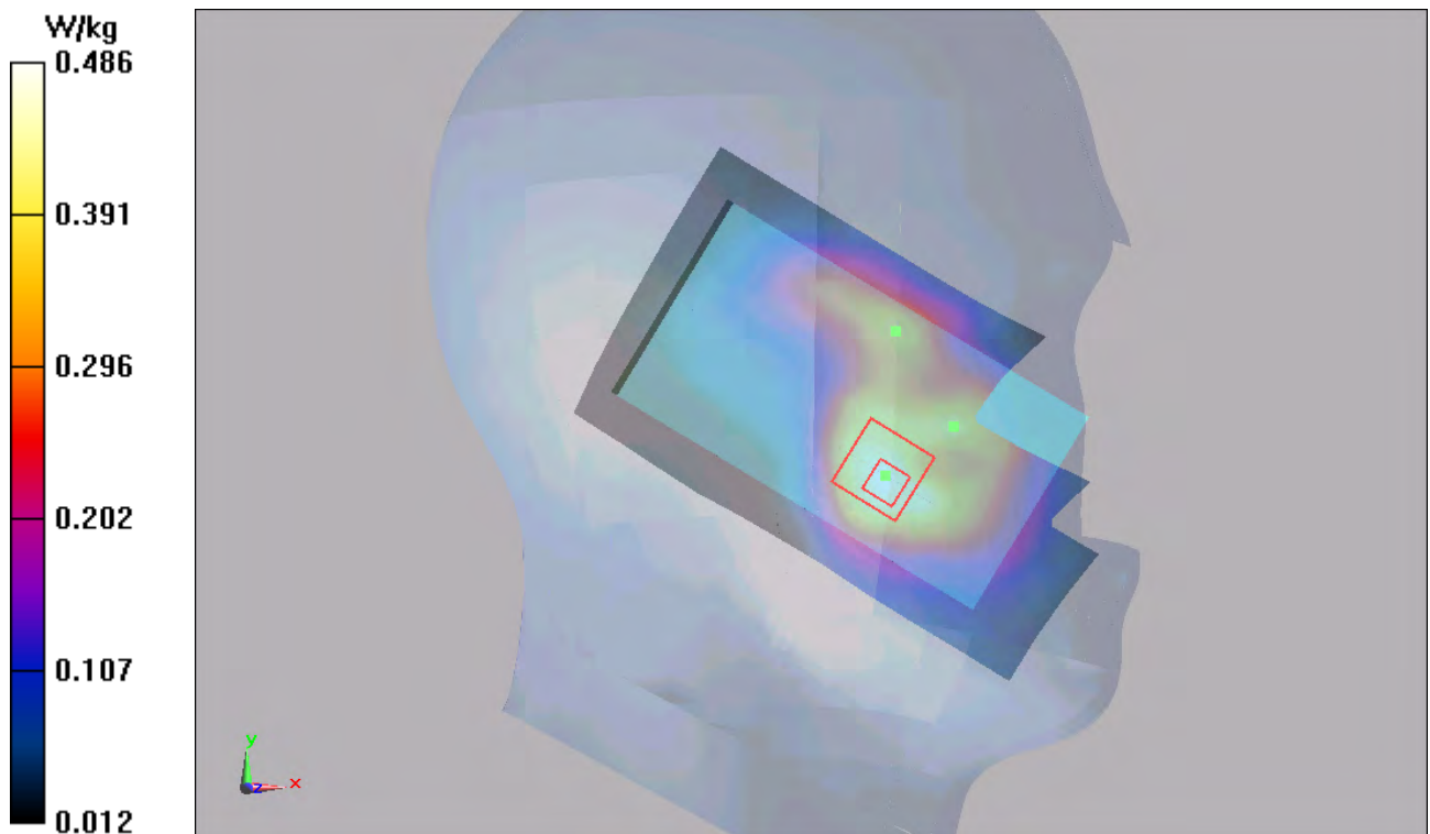
Figure 33 Left Hand Touch Cheek GSM 1900 Channel 661
