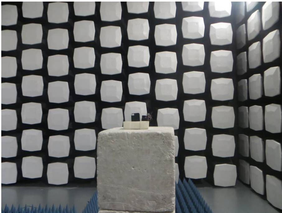
10. Radiated Emissions (Part 22/24) (Above 3GHz)
