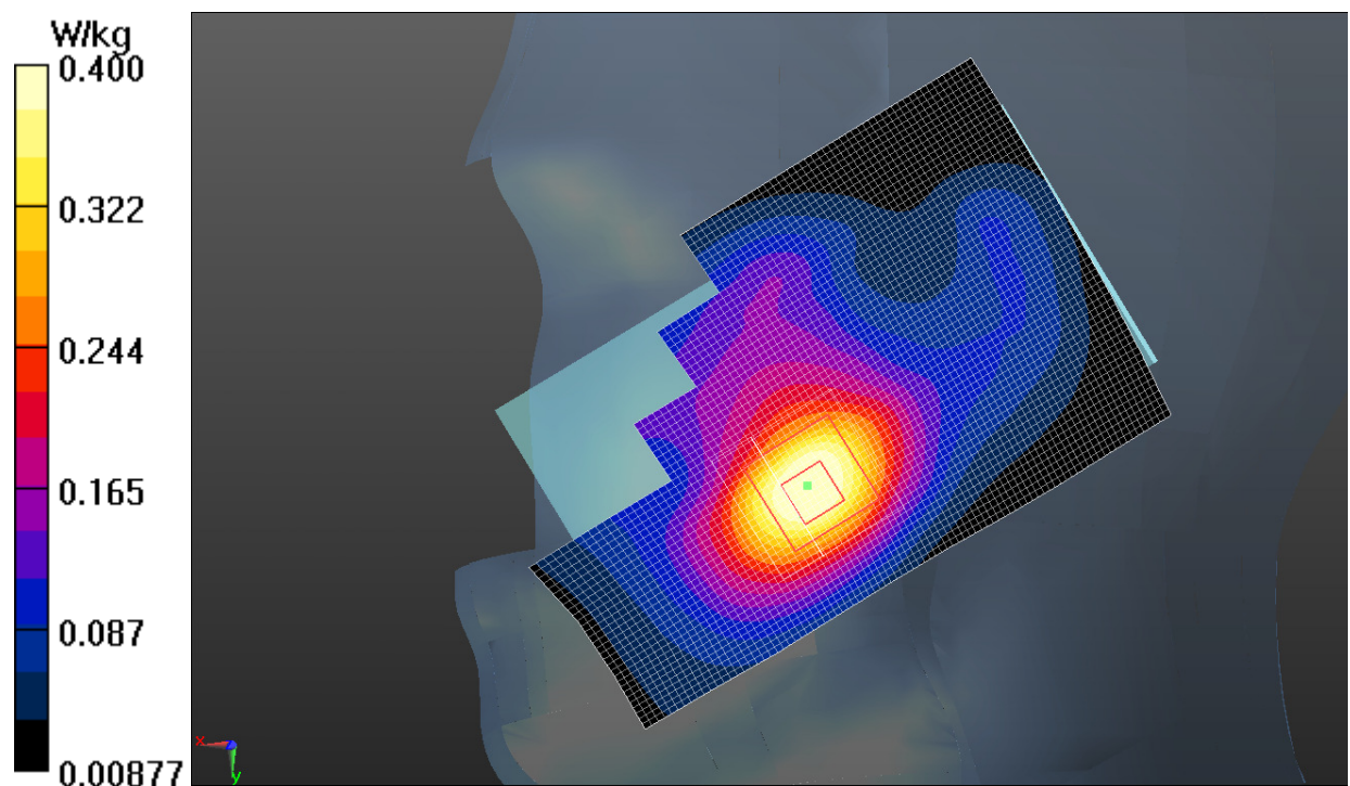
Fig.3 1900 MHz CH810
