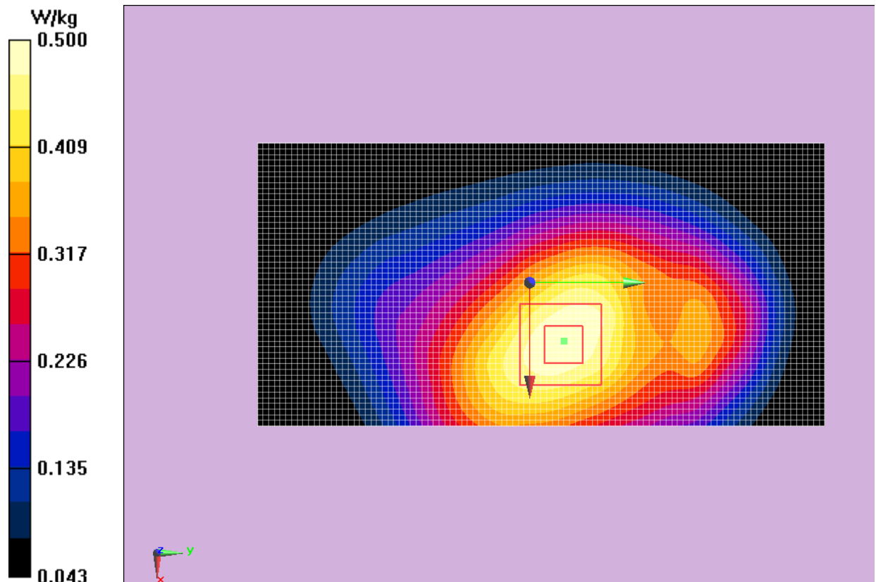
Fig.6 WCDMA 850 CH4183
