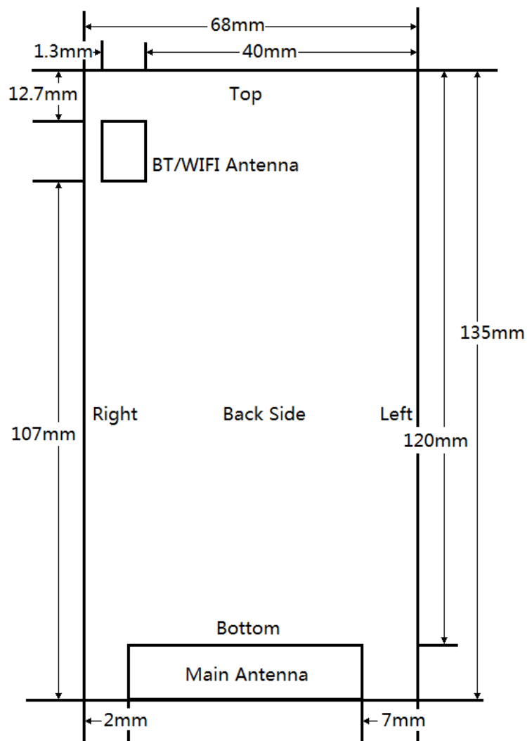
Mobile Hotspot Sides for SAR Testing
