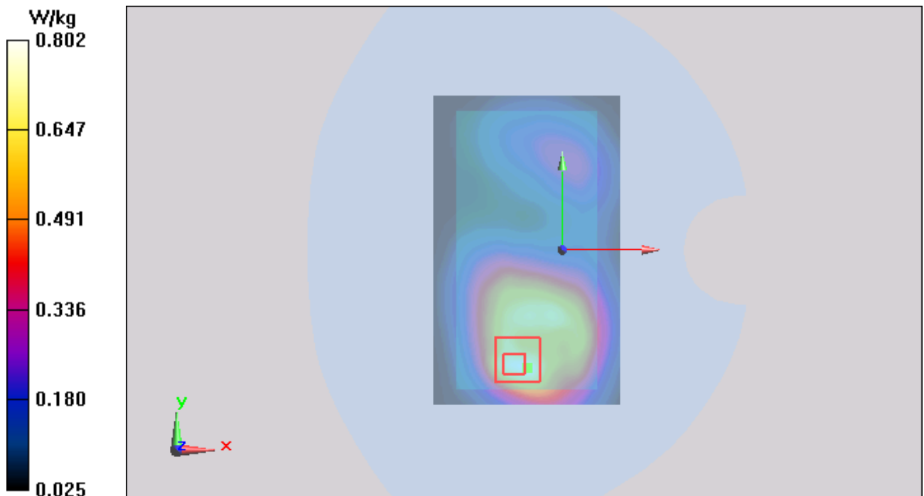
Figure 70 Body, Back Side, UMTS Band II Channel 9400
