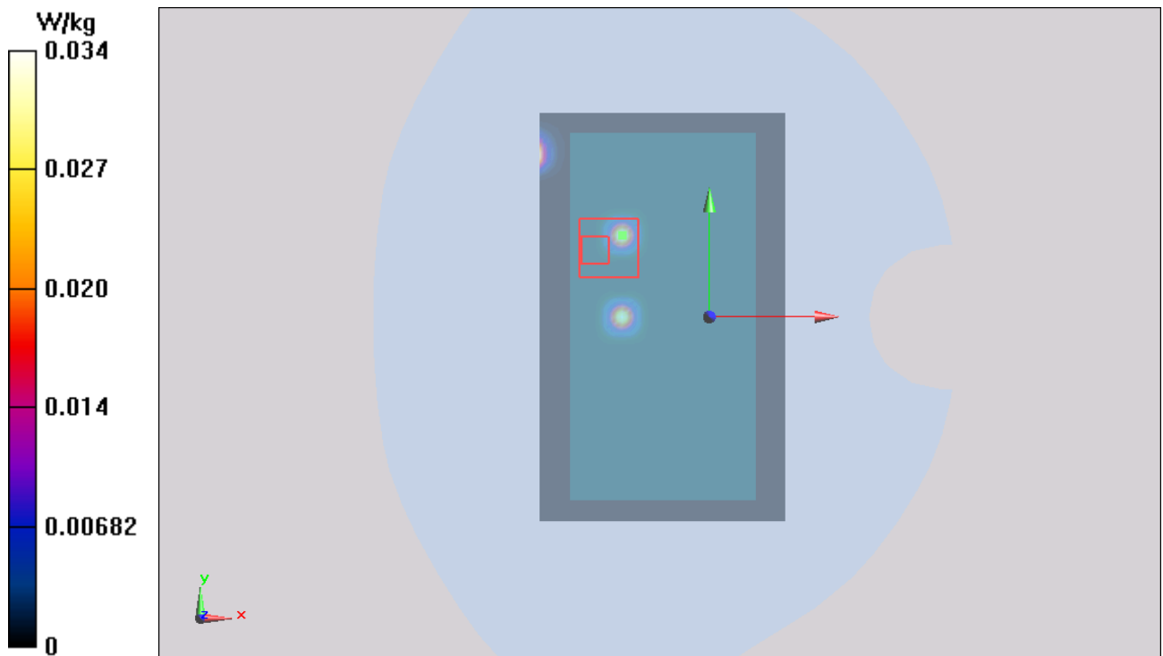
Figure 109 Body, Front Side, 802.11b Channel 11
