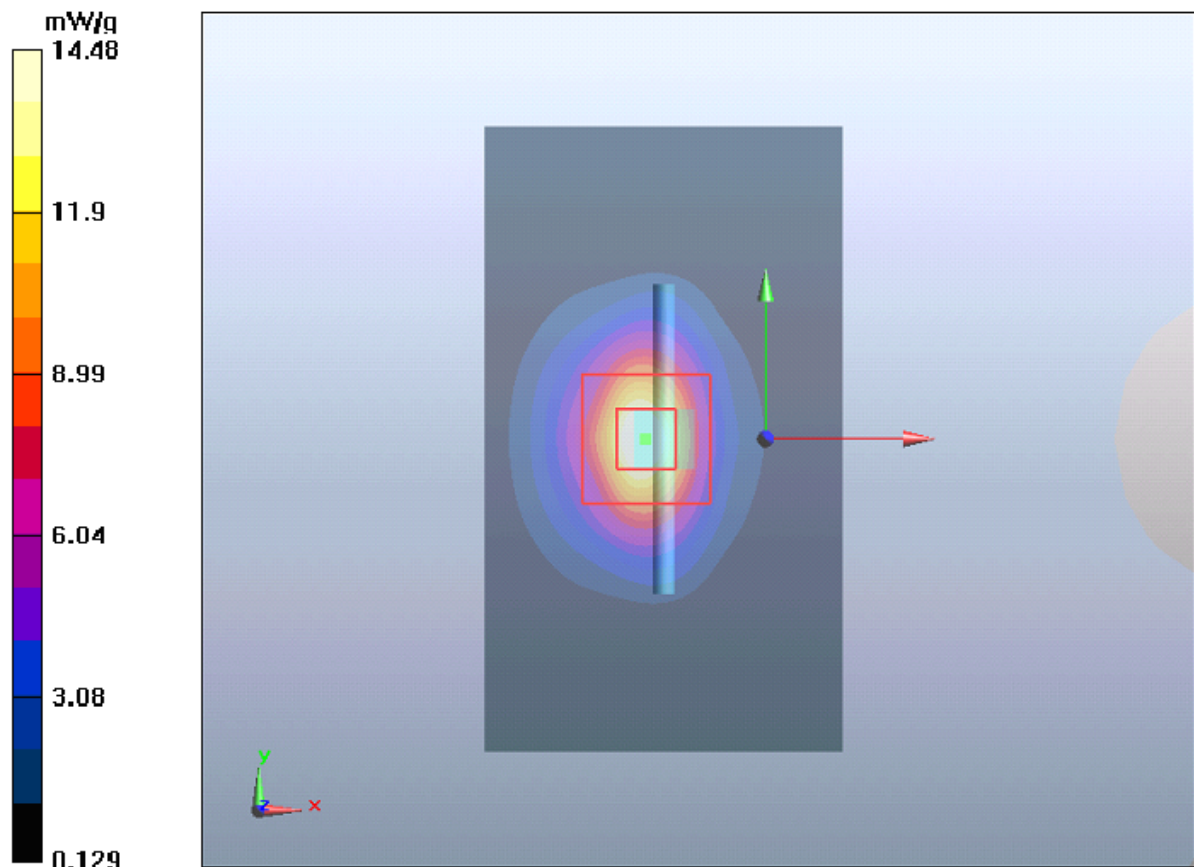
Figure 20 System Performance Check 2450MHz 250mW
