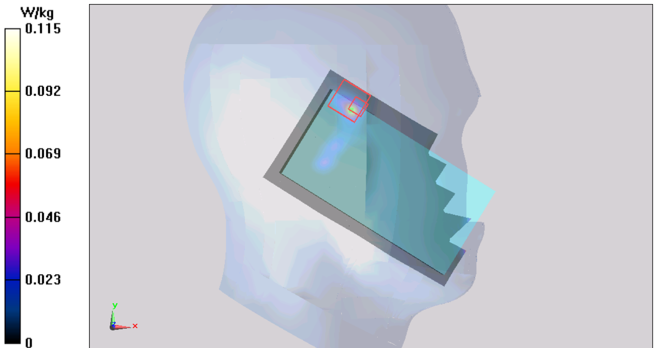
Figure 102 Left Hand Tilt 15° 802.11b Channel 11
