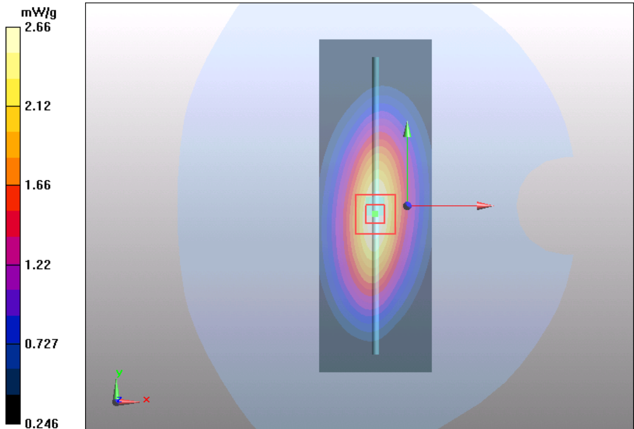
Figure 13 System Performance Check 835MHz 250mW
