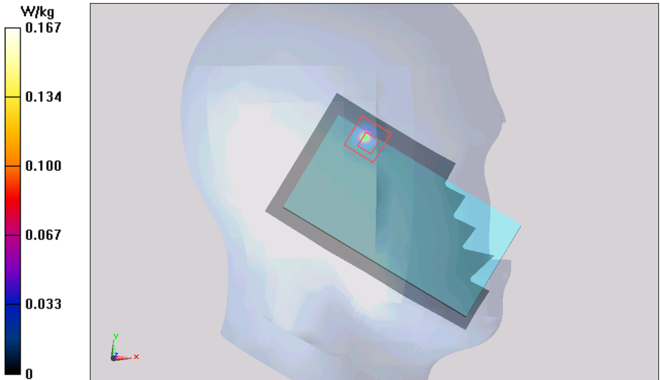
Figure 107 Left Hand Touch Cheek 802.11b Channel 11
