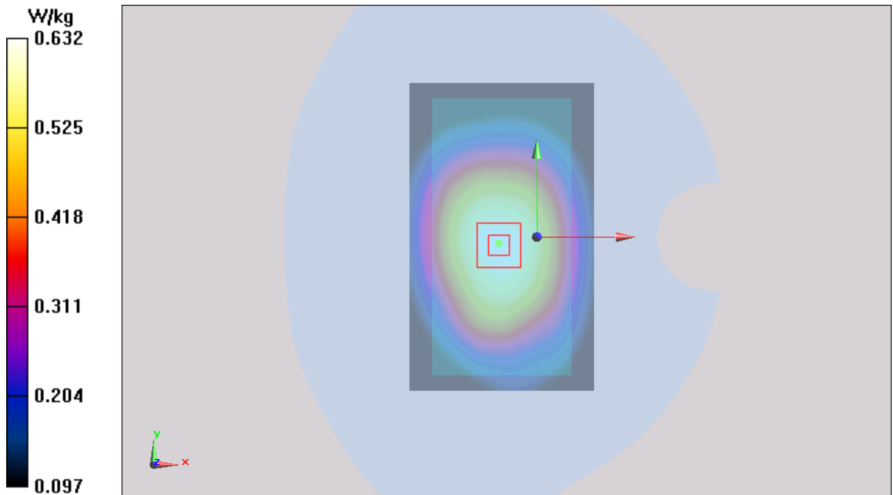
Figure 33 Body, Front Side, GSM 850 Channel 128
