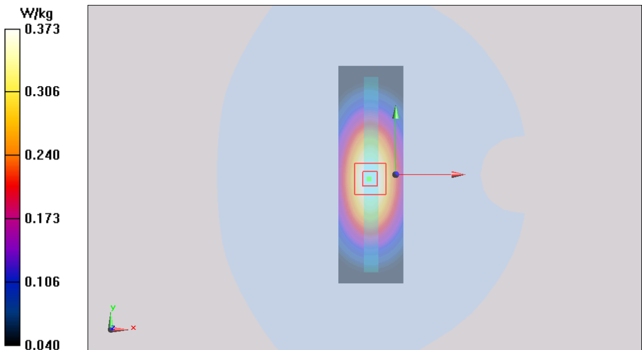
Figure 95 Body, Right Edge, UMTS Band V Channel 4183
