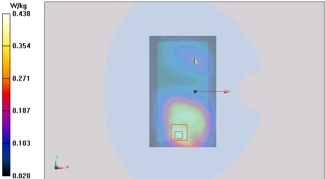
Figure 54 Body, Back Side, GSM 1900 Channel 661
