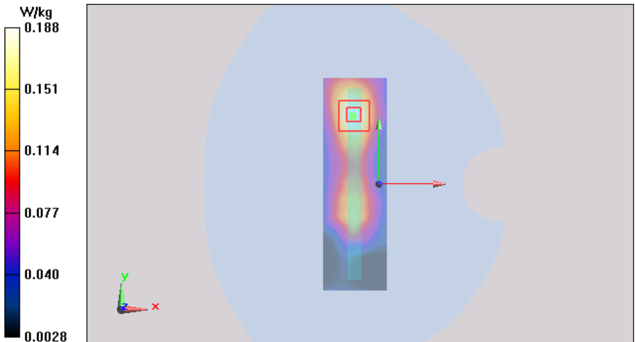
Figure 76 Body, Right Edge, UMTS Band II Channel 9400
