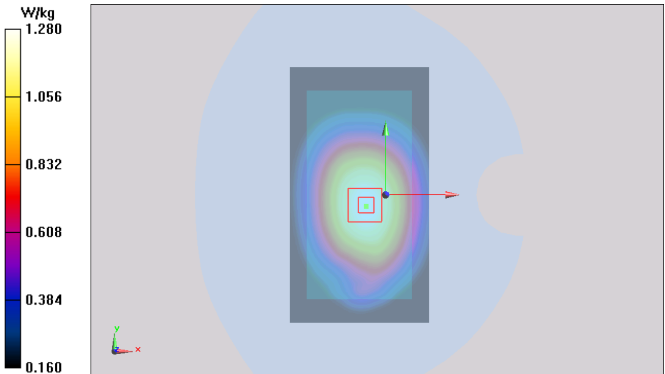
Figure 44 Body, Back Side, GSM 850 GPRS (3Txslots) Channel 251
