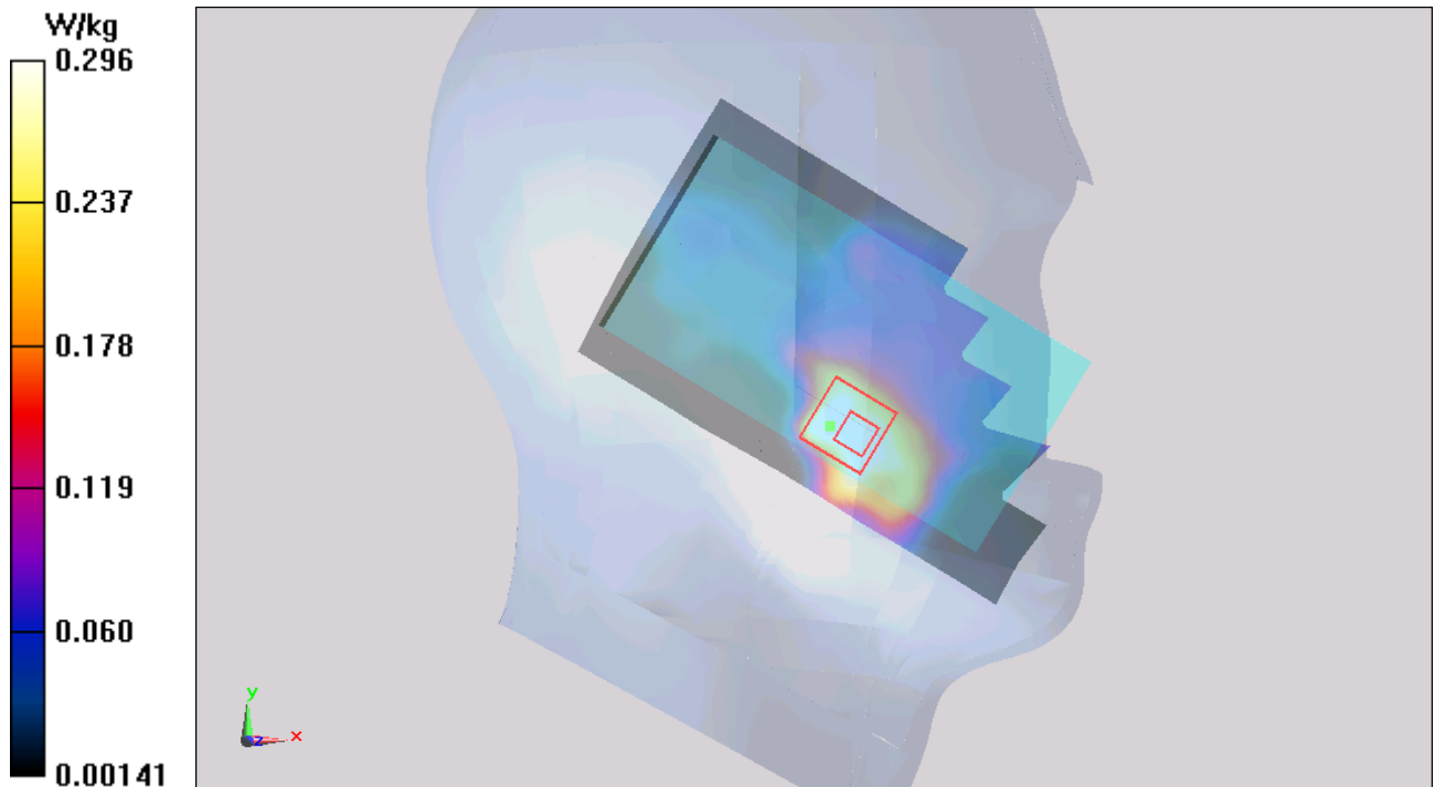
Figure 53 Left Hand Touch Cheek GSM 1900 Channel 661
