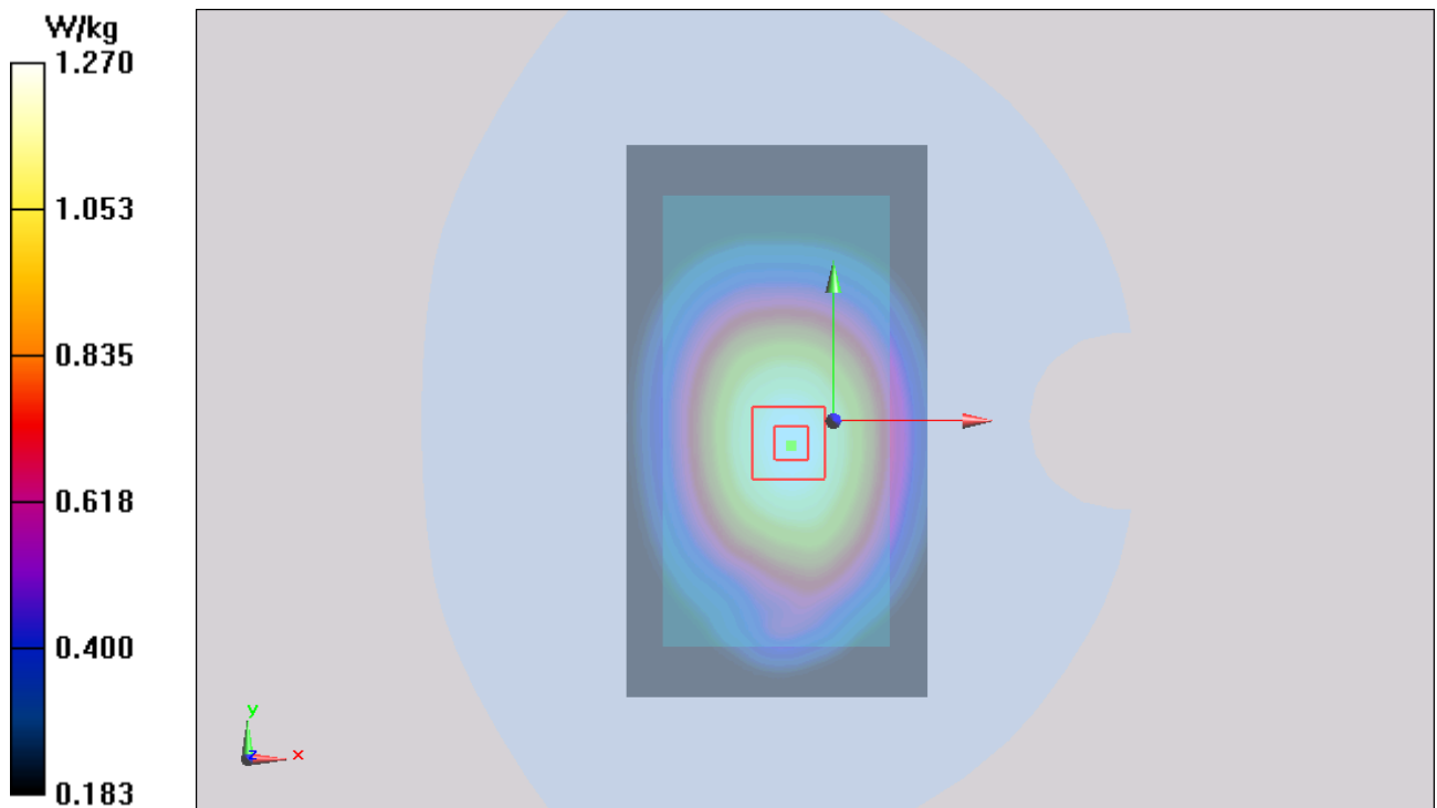
Figure 45 Body, Back Side, GSM 850 GPRS (3Txslots) Channel 251
