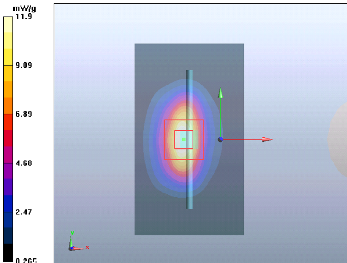
Figure 18 System Performance Check 1900MHz 250mW
