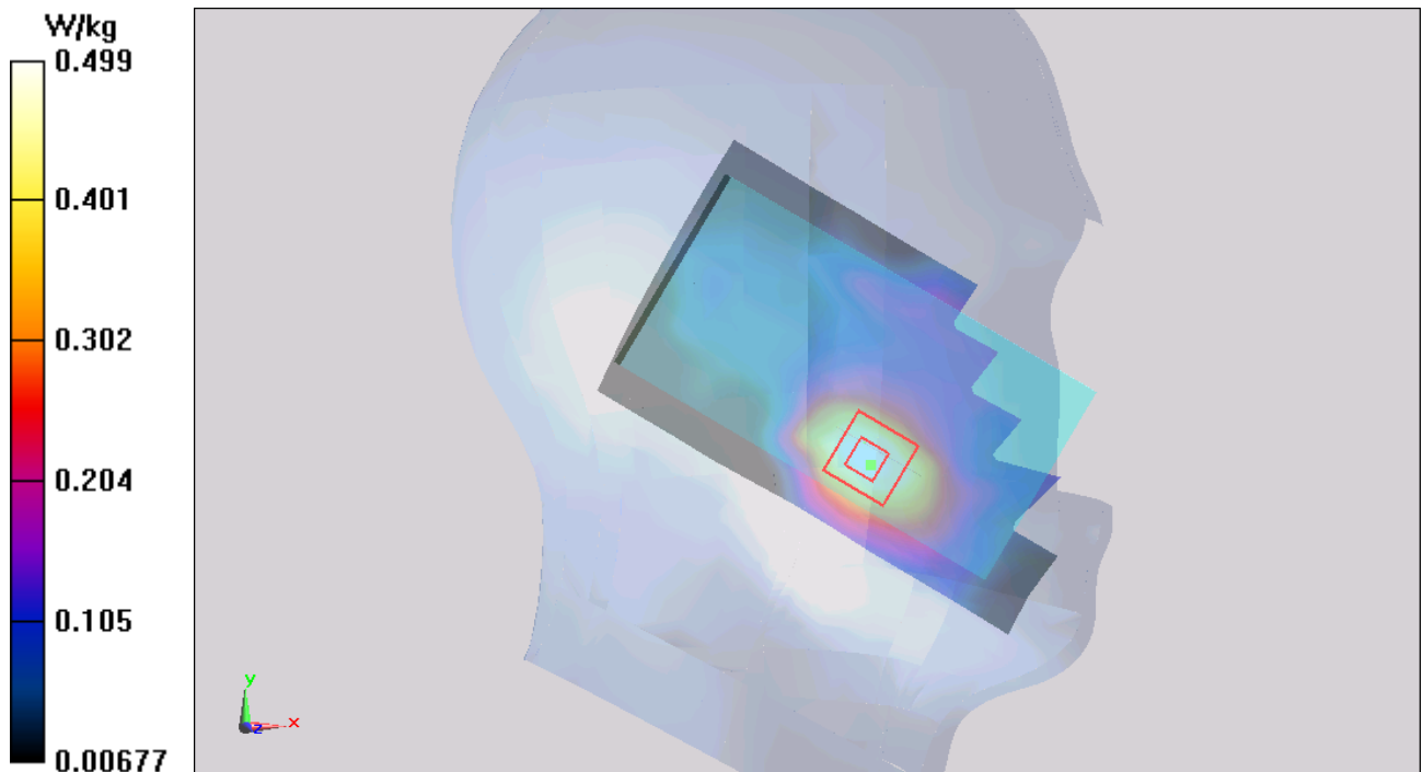
Figure 64 Left Hand Touch Cheek UMTS Band II Channel 9400
