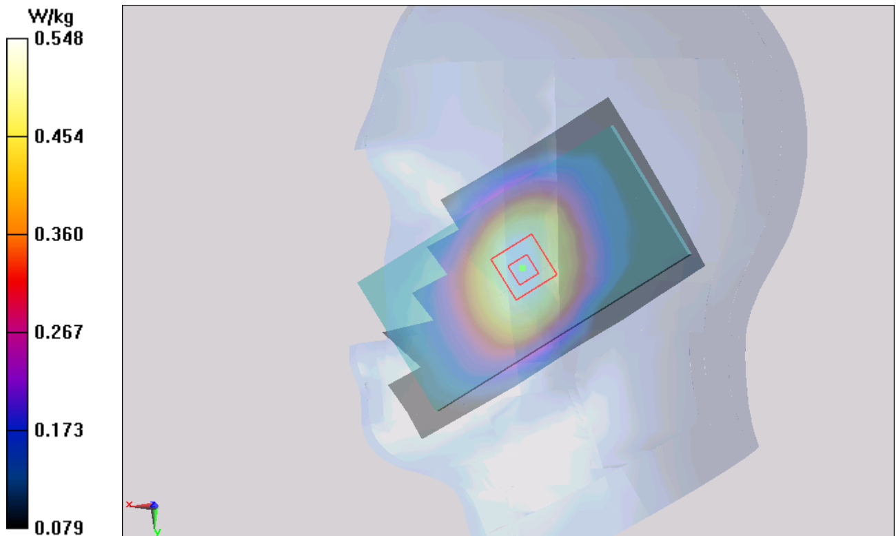
Figure 83 Right Hand Touch Cheek UMTS Band V Channel 4183
