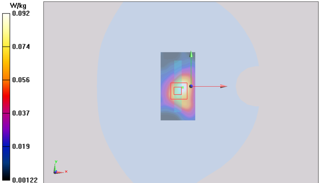
Figure 96 Body, Bottom Edge, UMTS Band V Channel 4183
