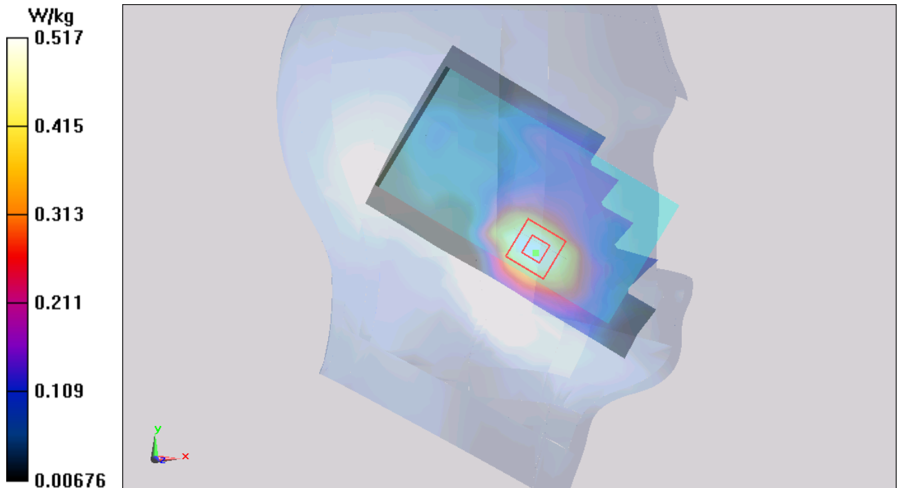
Figure 69 Left Hand Touch Cheek UMTS Band II Channel 9400
