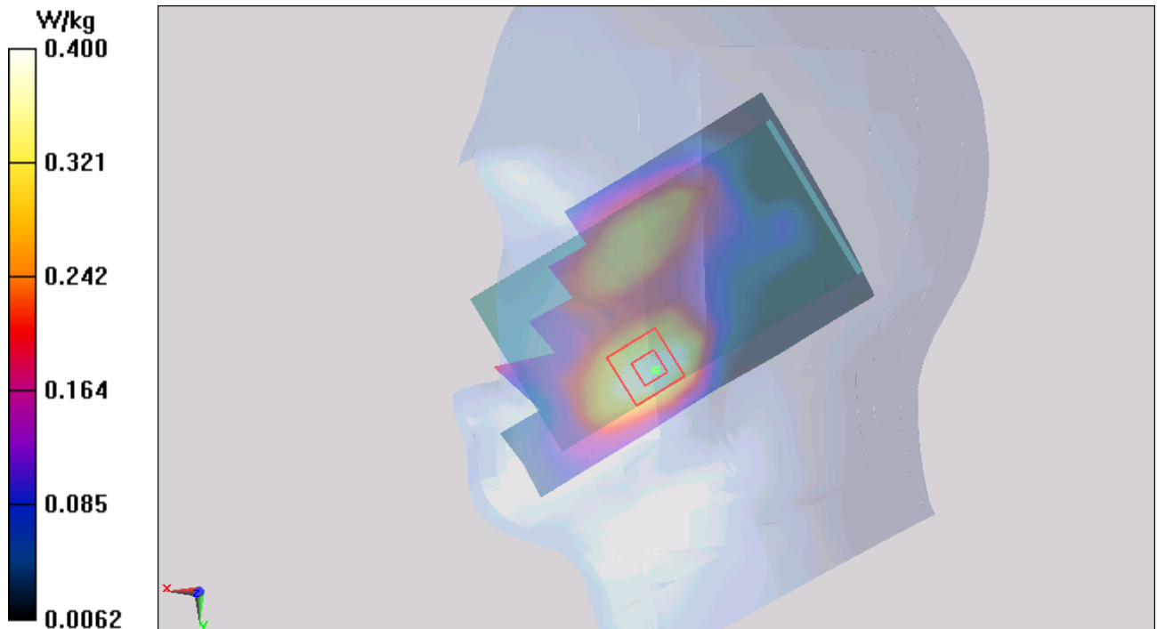
Figure 66 Right Hand Touch Cheek UMTS Band II Channel 9400
