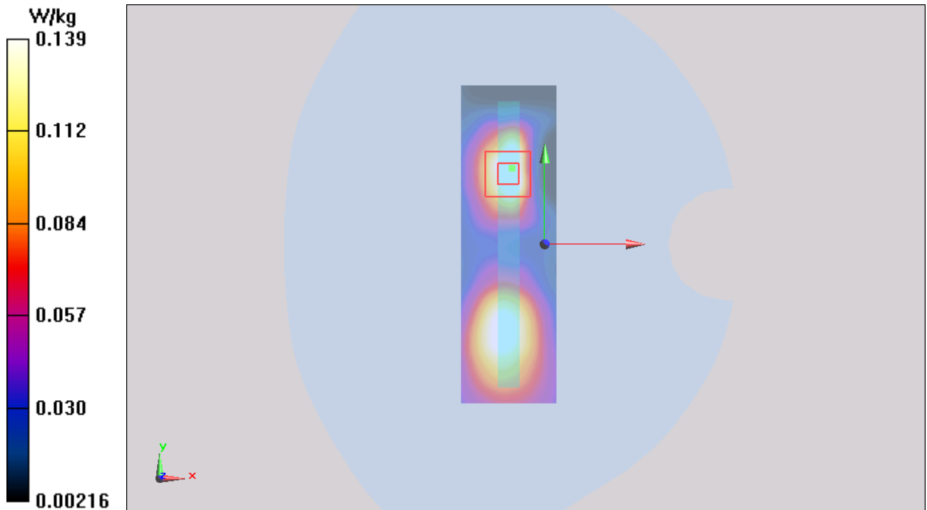
Figure 58 Body, Left Edge, GSM 1900 GPRS (2Txslots) Channel 661
