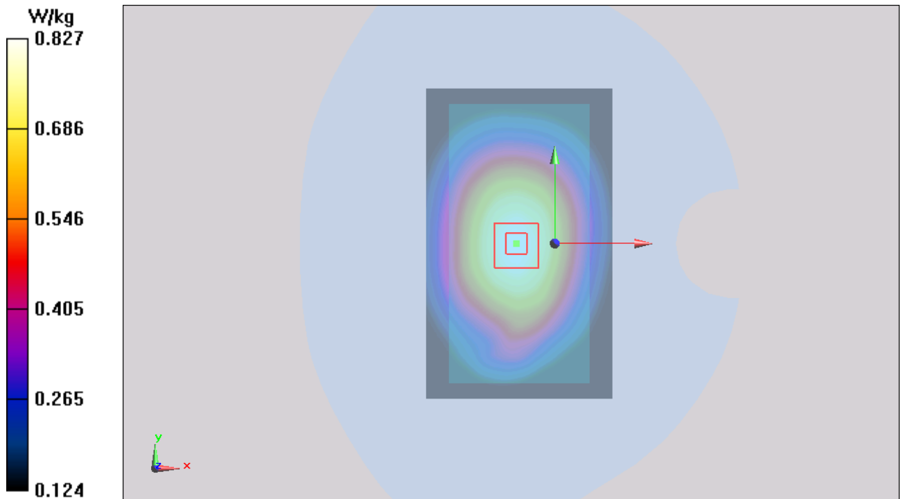
Figure 30 Body, Back Side, GSM 850 Channel 128
