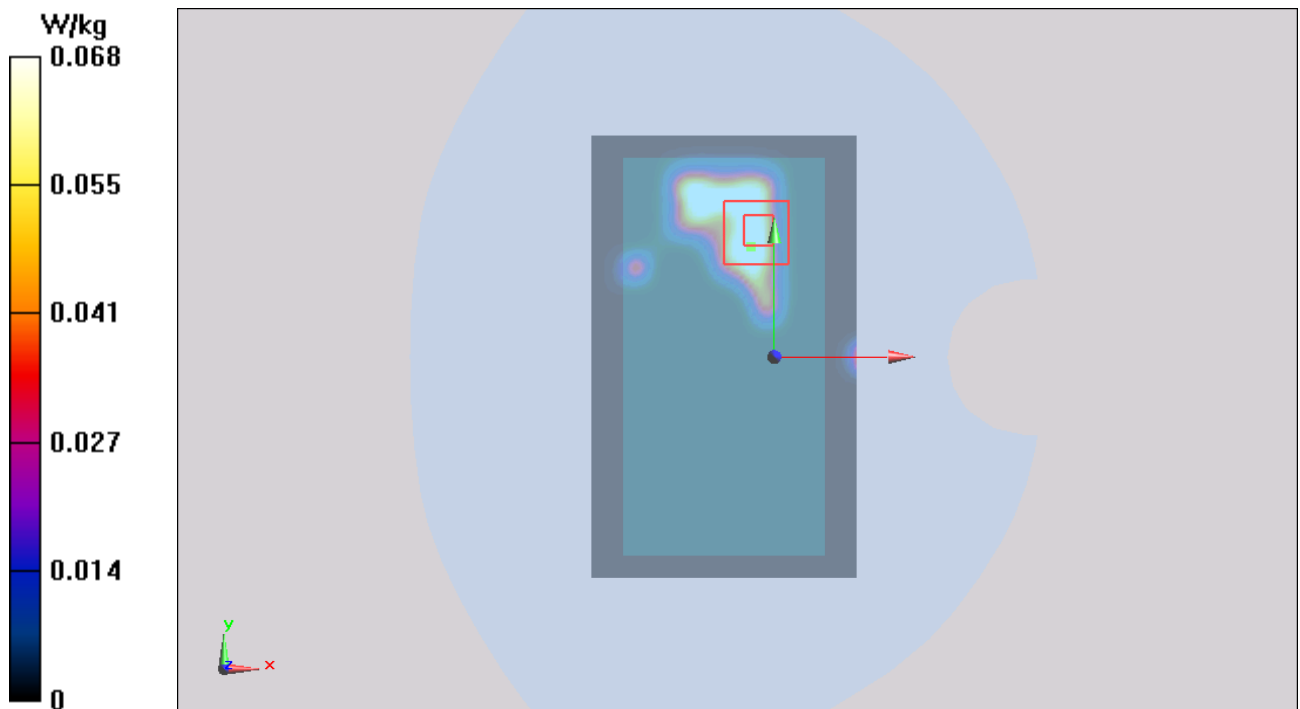
Figure 108 Body, Back Side, 802.11b Channel 11
