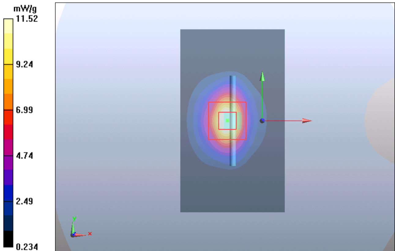
Figure 17 System Performance Check 1900MHz 250mW
