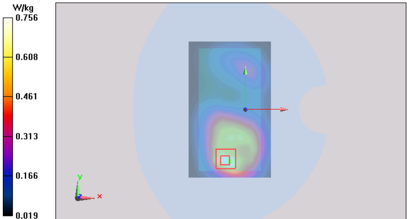
Figure 71 Body, Back Side, UMTS Band II Channel 9538
