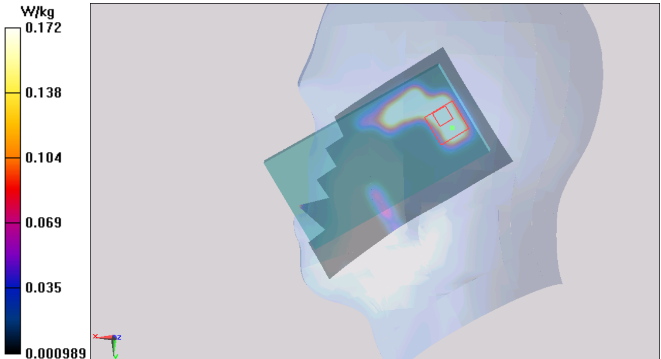
Figure 67 Right Hand Tilt 15° UMTS Band II Channel 9400
