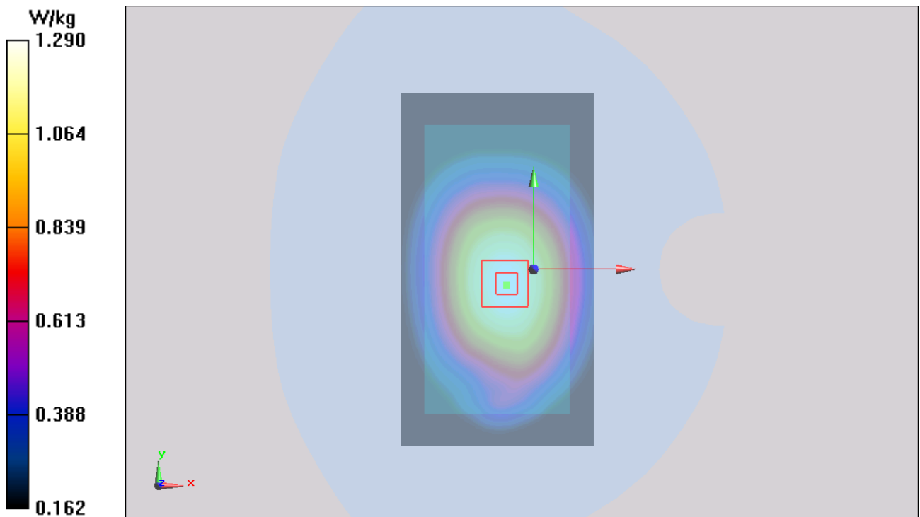
Figure 43 Body, Back Side, GSM 850 GPRS (3Txslots) Channel 251
