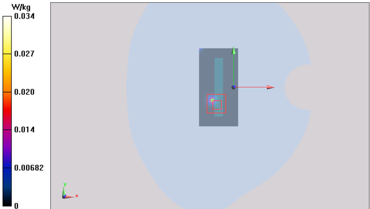
Figure 111 Body, Top Edge, 802.11b Channel 11
