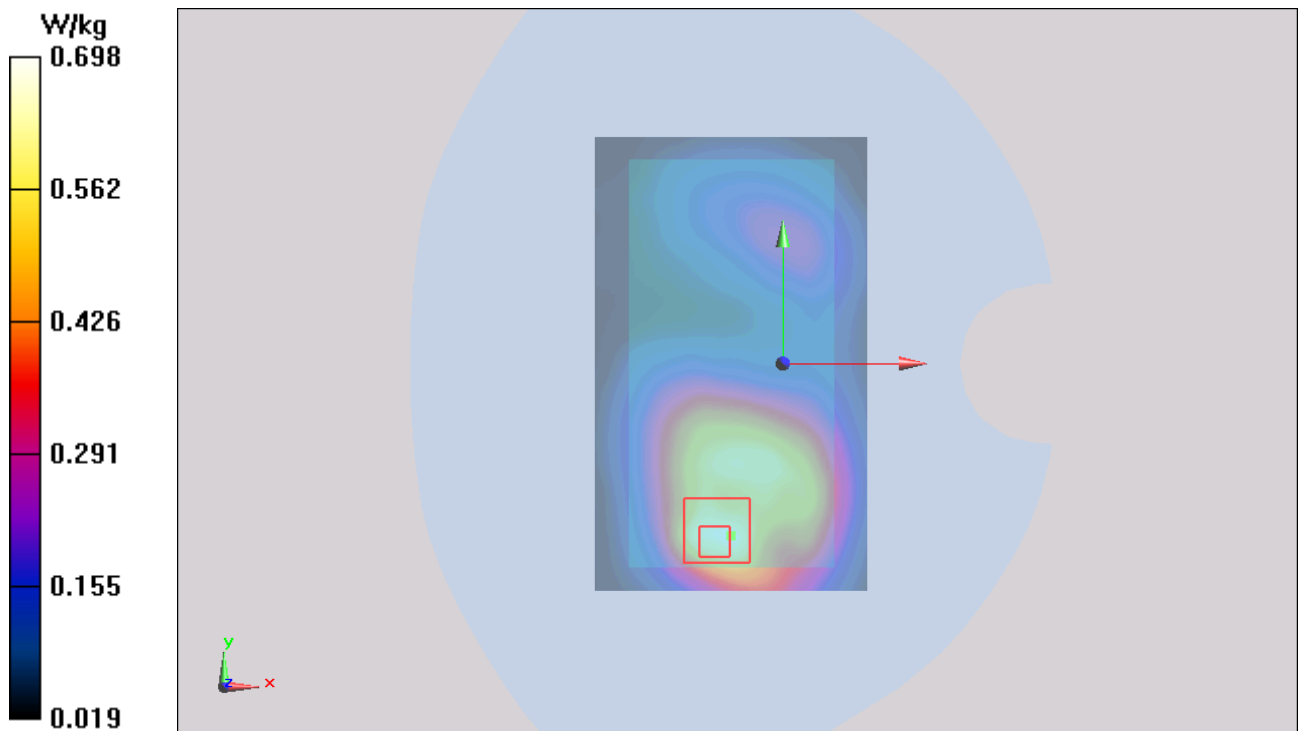
Figure 61 Body, Back Side, GSM 1900 GPRS (2Txslots) Channel 661
