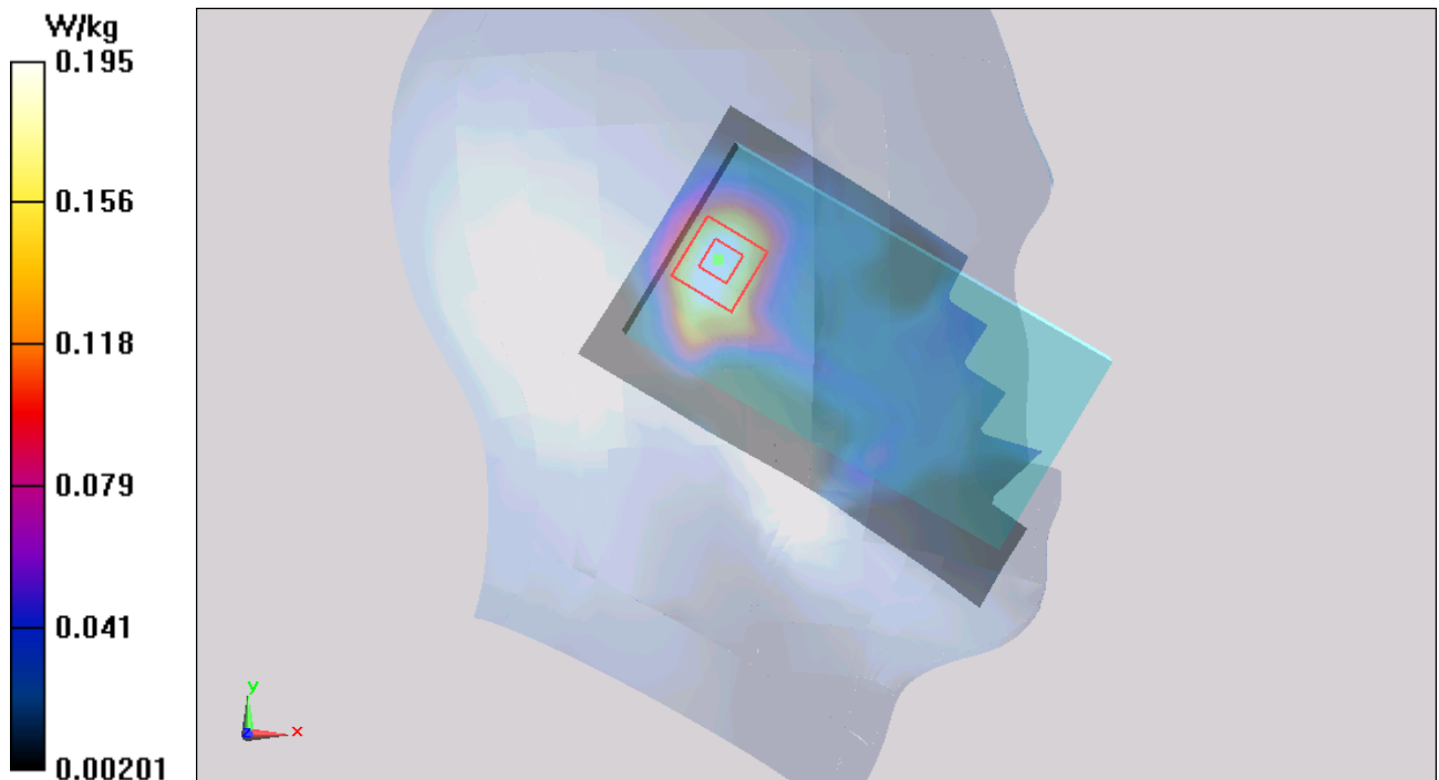
Figure 65 Left Hand Tilt 15° UMTS Band II Channel 9400
