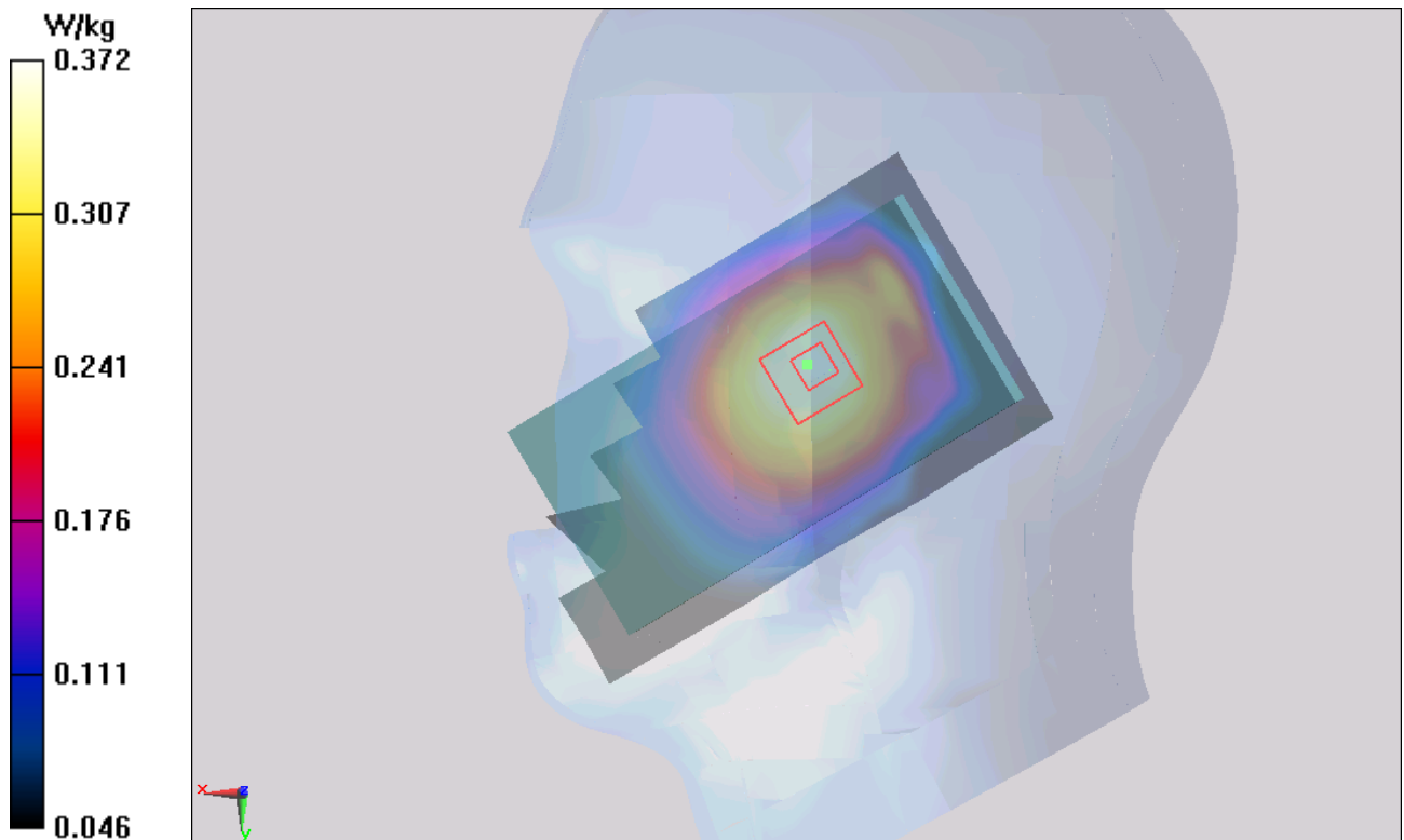
Figure 84 Right Hand Tilt 15° UMTS Band V Channel 4183
