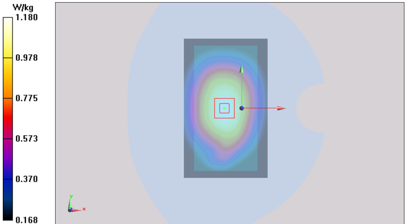
Figure 35 Body, Back Side, GSM 850 GPRS (3Txslots) Channel 190
