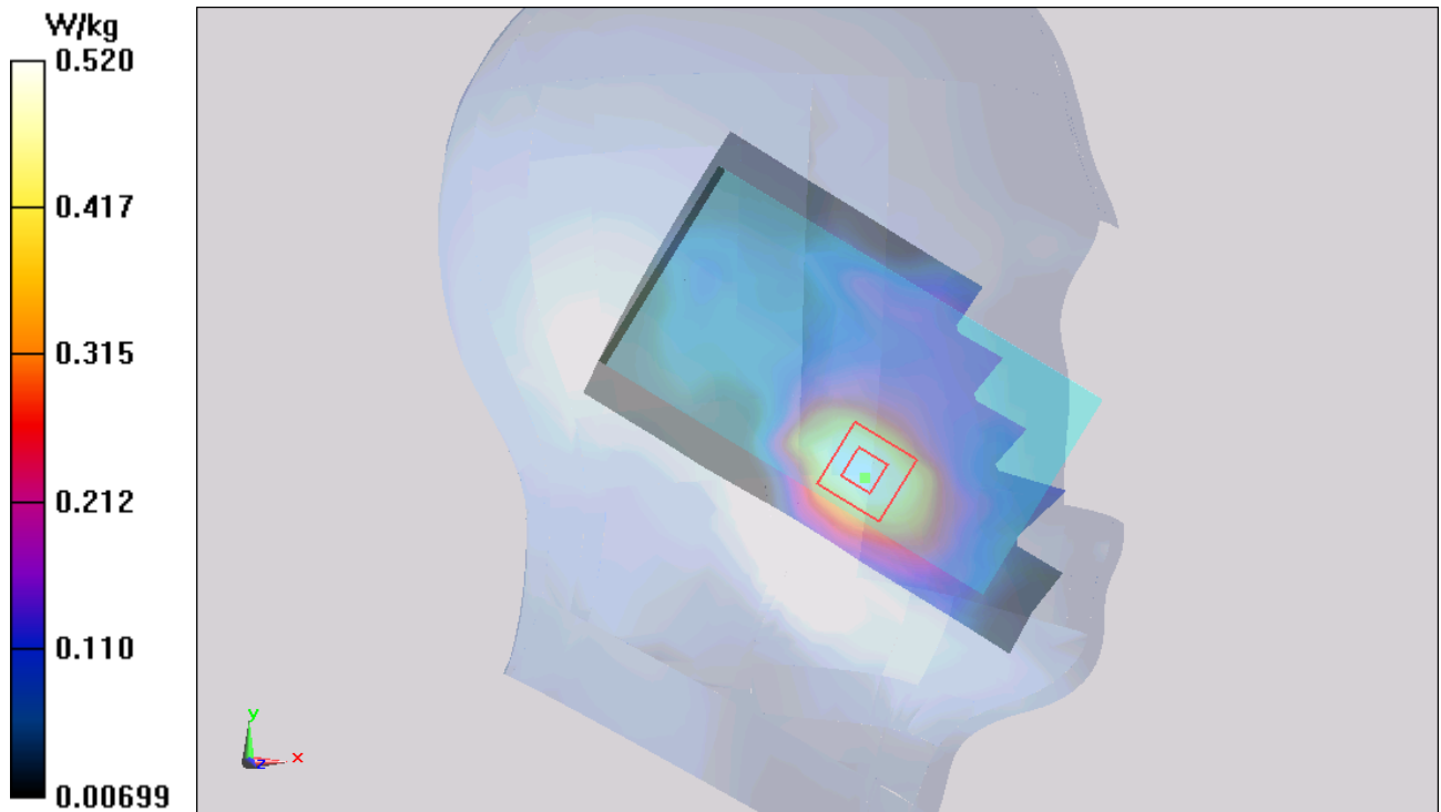
Figure 70 Left Hand Touch Cheek UMTS Band II Channel 9400
