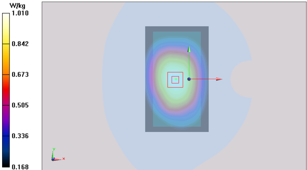
Figure 38 Body, Front Side, GSM 850 GPRS (3Txslots)Channel 190
