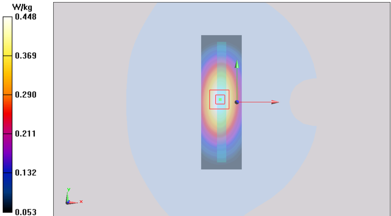
Figure 40 Body, Left Edge, GSM 850 GPRS (3Txslots)Channel 190
