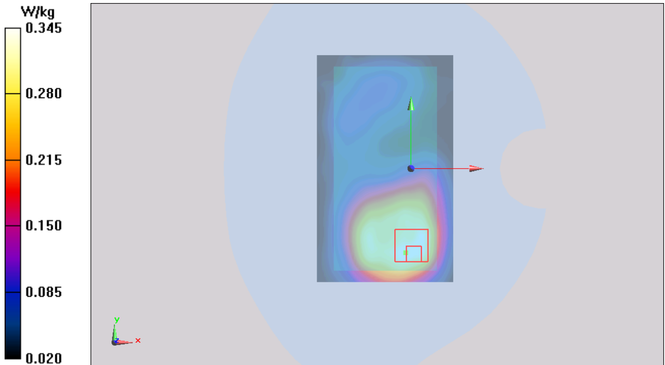
Figure 55 Body, Front Side, GSM 1900 Channel 661
