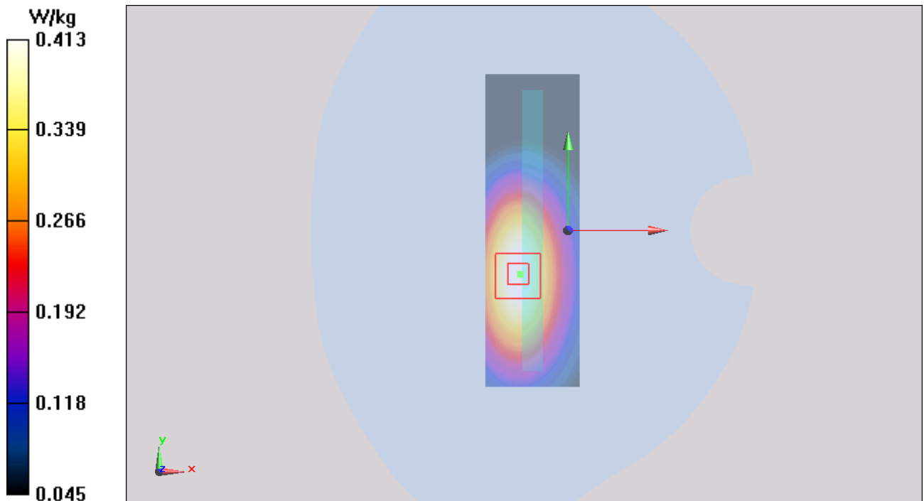
Figure 94 Body, Left Edge, UMTS Band V Channel 4183
