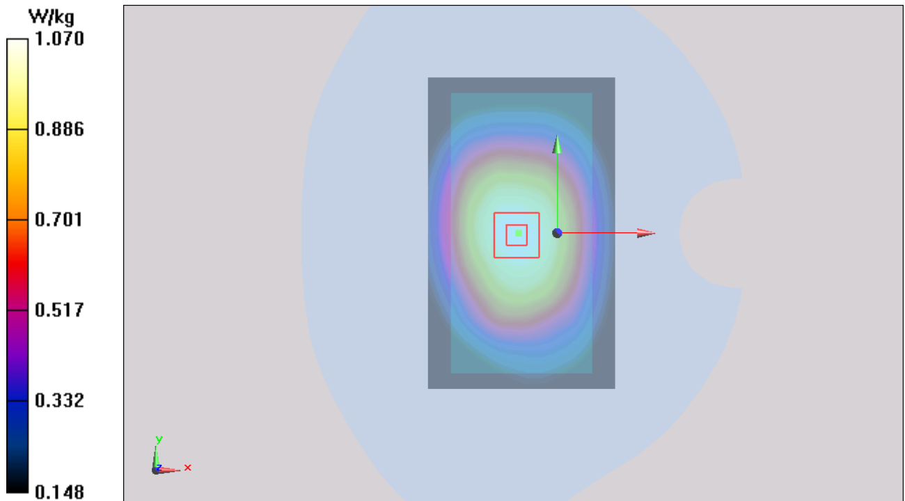
Figure 37 Body, Front Side, GSM 850 GPRS (3Txslots)Channel 251
