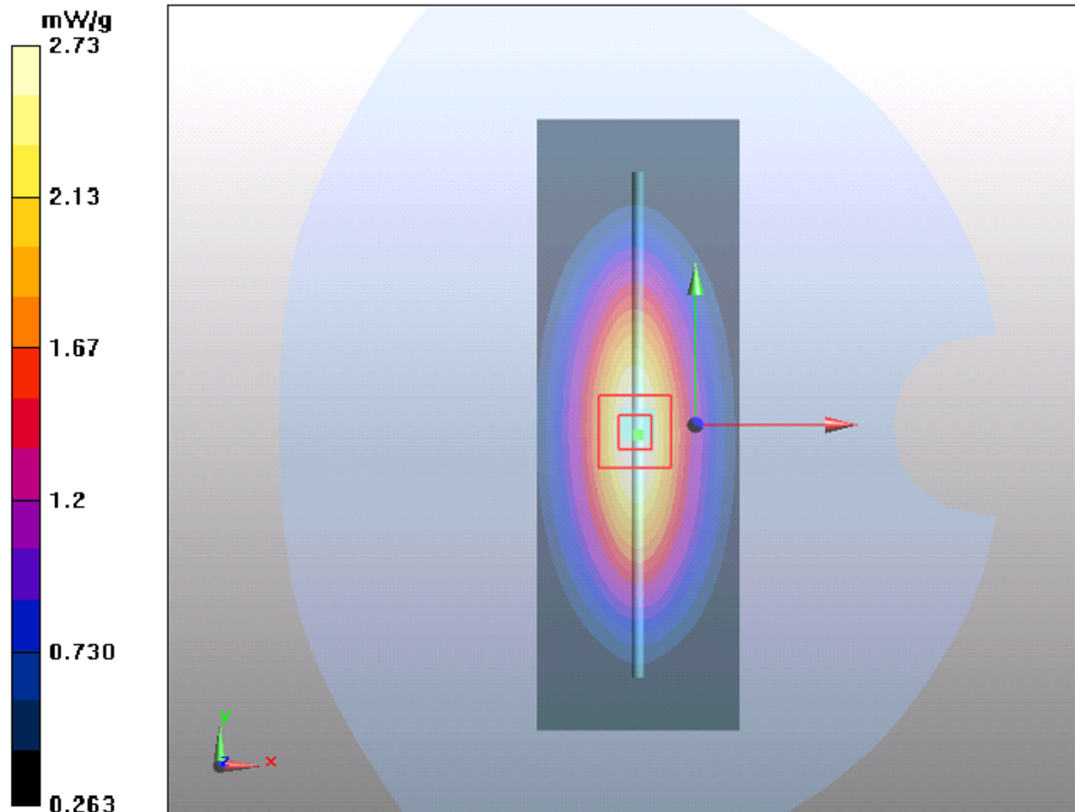
Figure 14 System Performance Check 835MHz 250Mw
