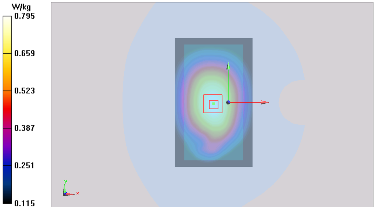
Figure 29 Body, Back Side, GSM 850 Channel 190
