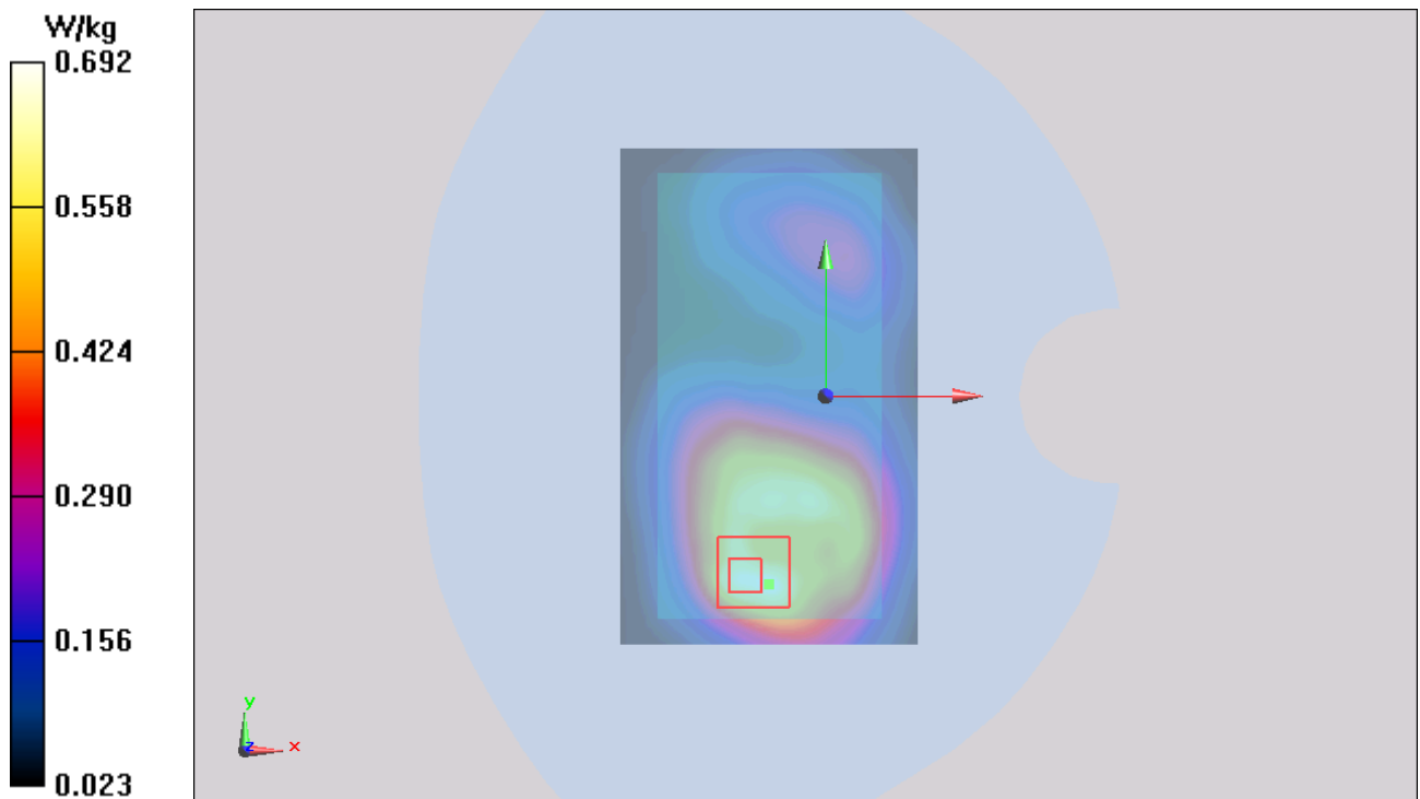
Figure 63Body, Back Side, GSM 1900 GPRS (2Txslots) Channel 661
