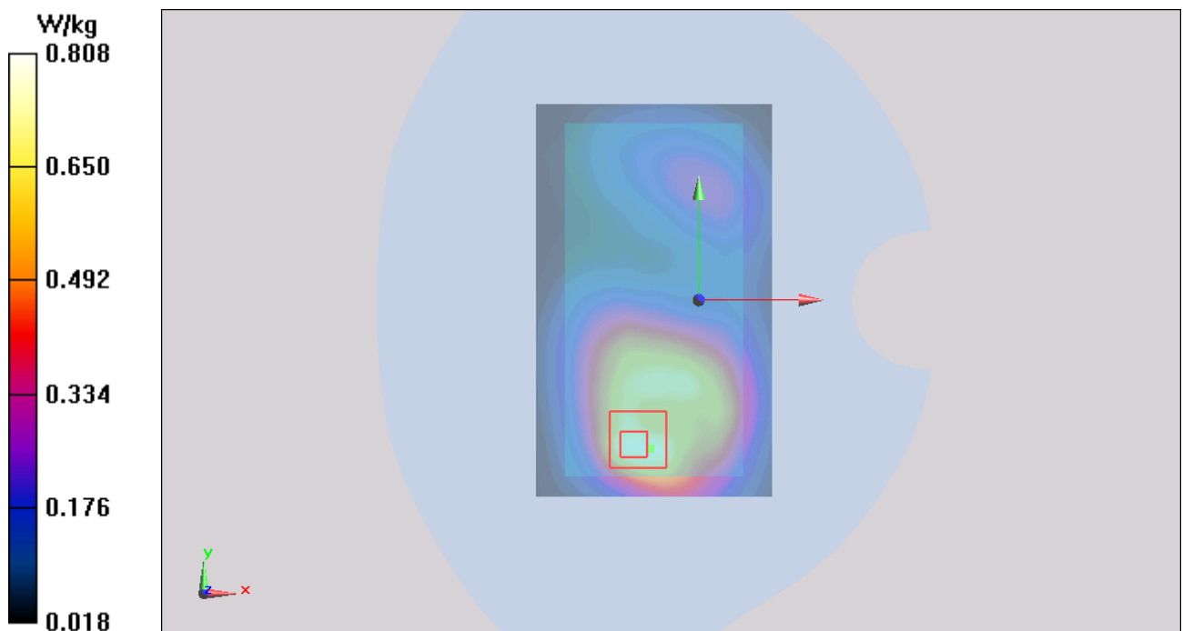
Figure 80 Body, Back Side, UMTS Band II Channel 9400
