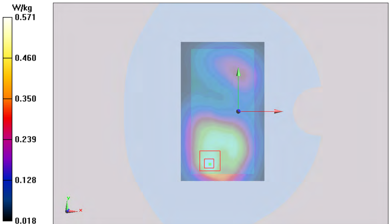
Figure 118 Body, Back Side, GSM 1900 GPRS (2Txslots) Channel 661
