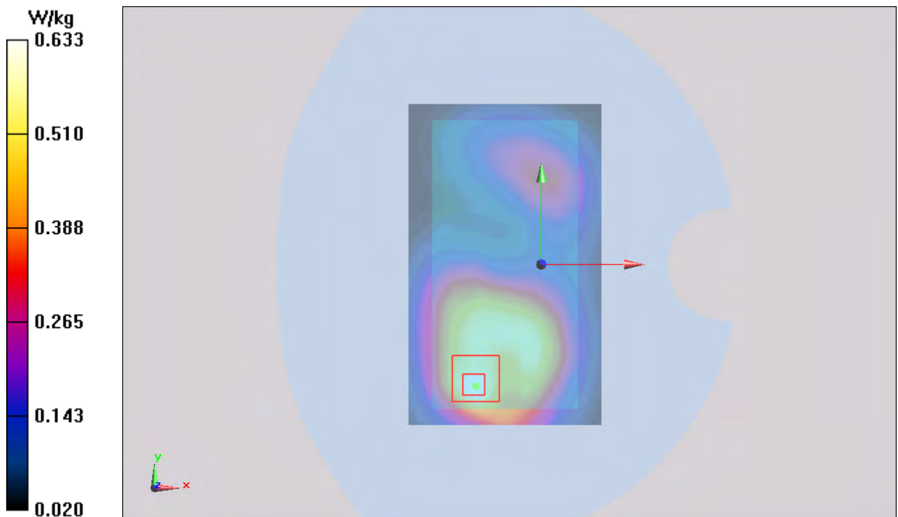
Figure 121 Body, Back Side, UMTS Band II Channel 9400
