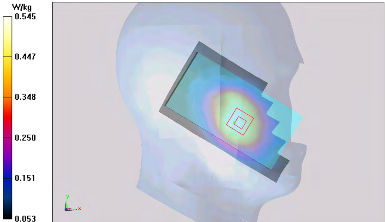
Figure 122 Left Touch Cheek UMTS Band V Channel 4183
