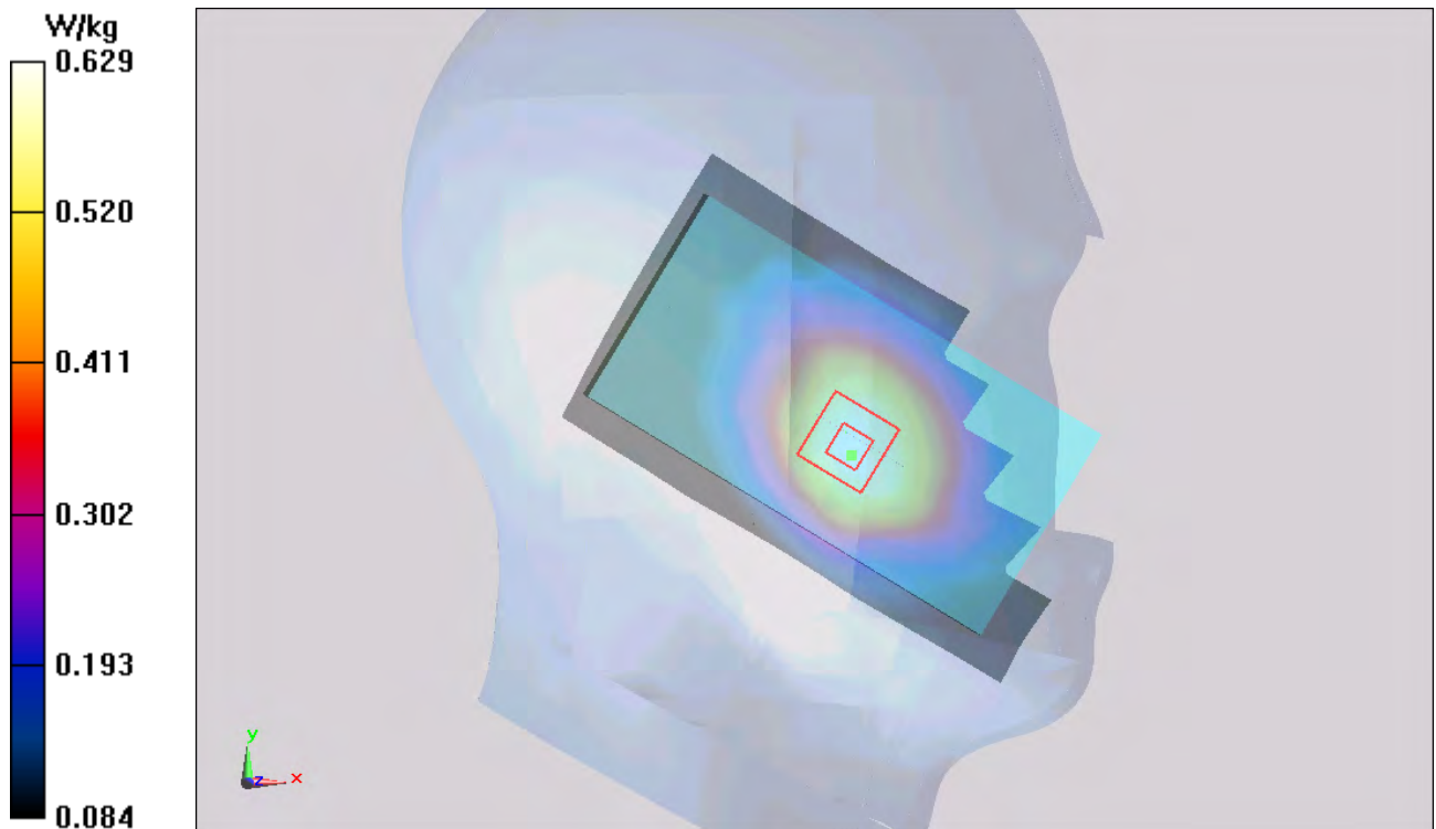
Figure 112 Left Hand Touch Cheek GSM 850 Channel 190
