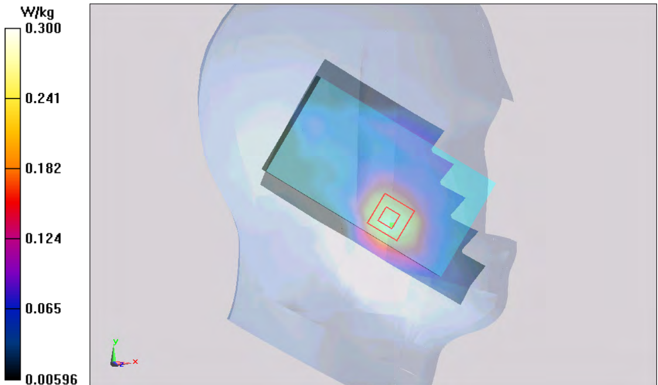
Figure 116 Left Hand Touch Cheek GSM 1900 Channel 661
