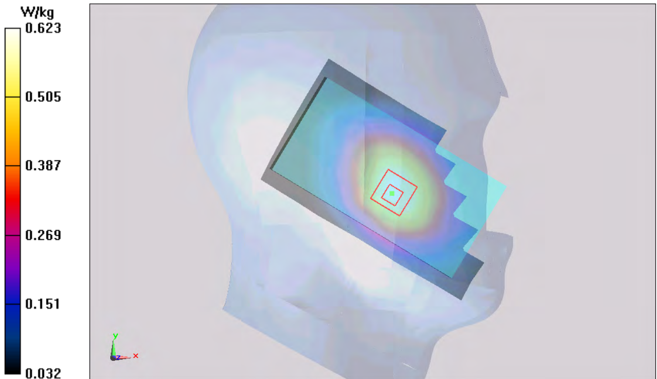
Figure 111 Left Hand Touch Cheek GSM 850 Channel 190
