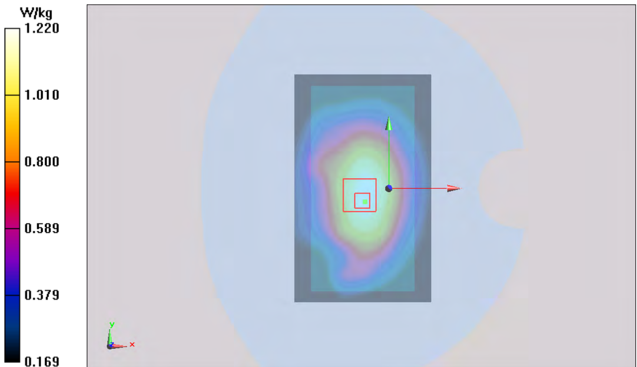
Figure 114 Body, Back Side, GSM 850 GPRS (3Txslots) Channel 251
