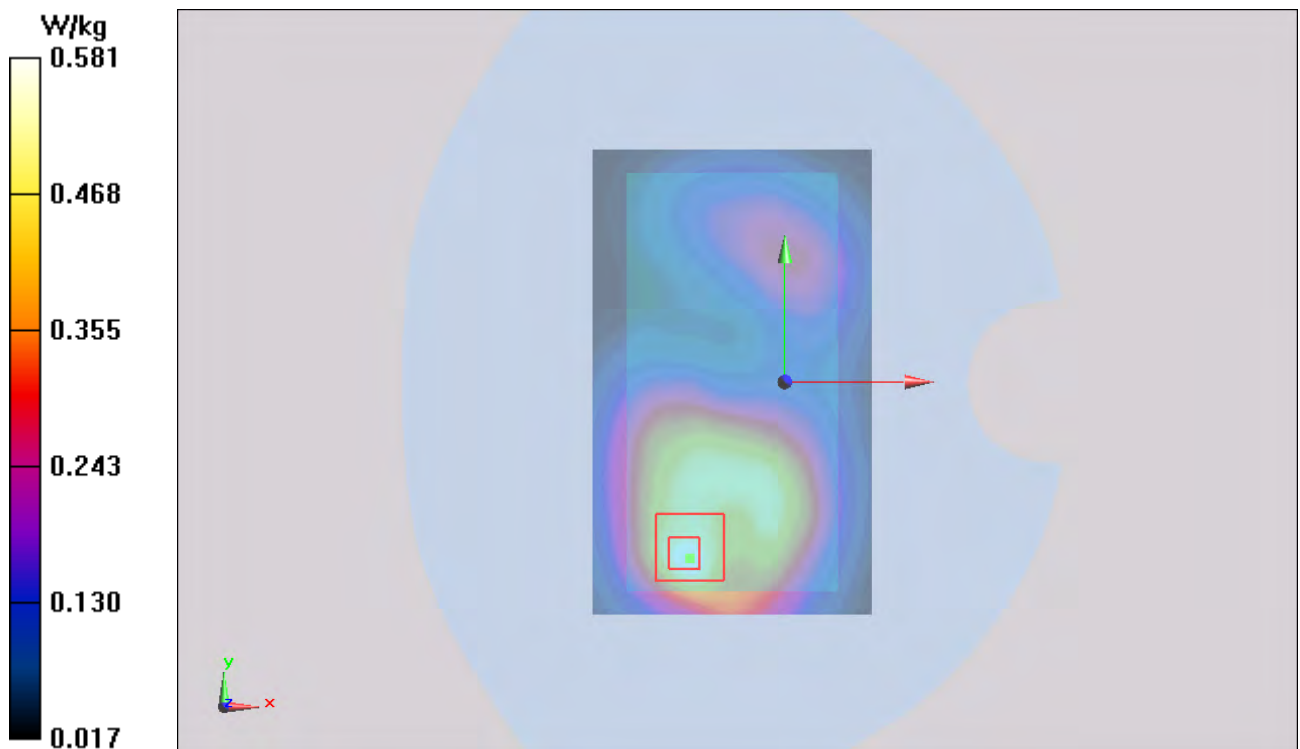
Figure 119 Body, Back Side, GSM 1900 GPRS (2Txslots) Channel 661
