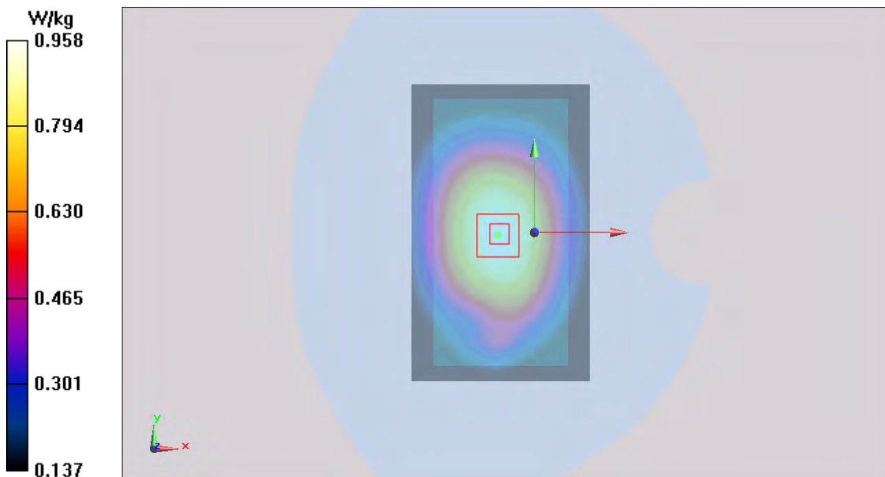
Figure 89 Body, Back Side, UMTS Band V Channel 4233
