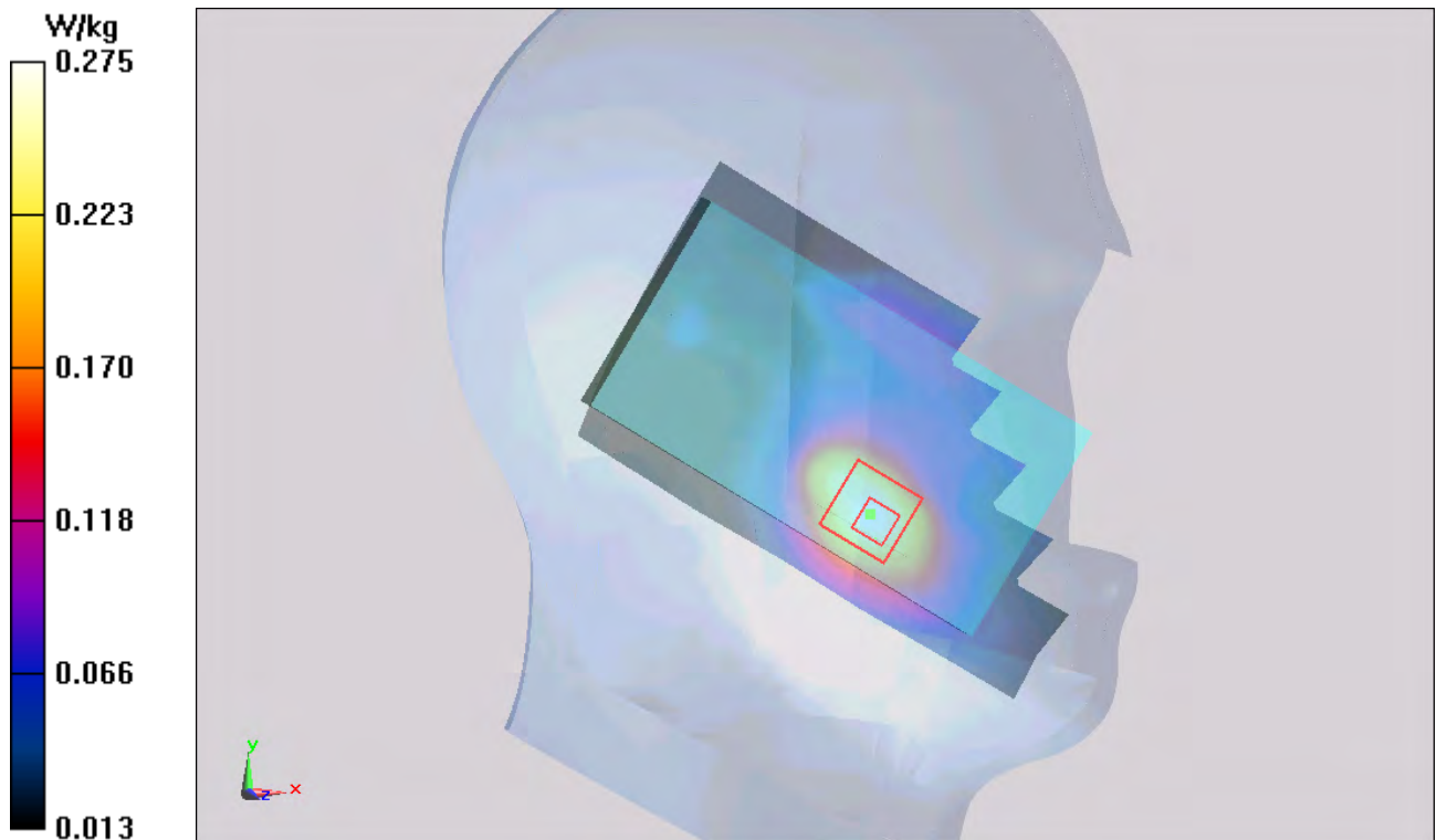
Figure 117 Left Hand Touch Cheek GSM 1900 Channel 661
