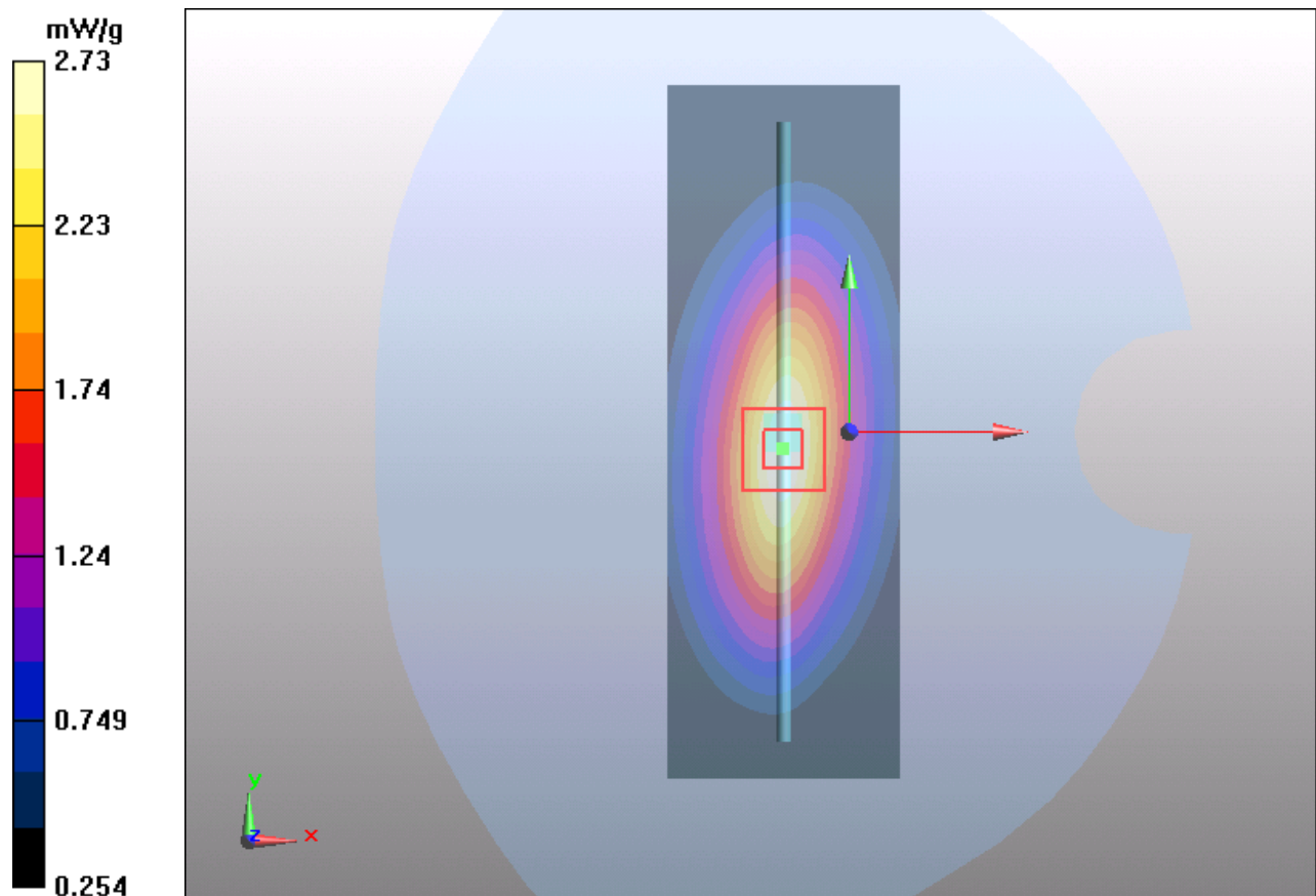
Figure 107 System Performance Check 835MHz 250mW
