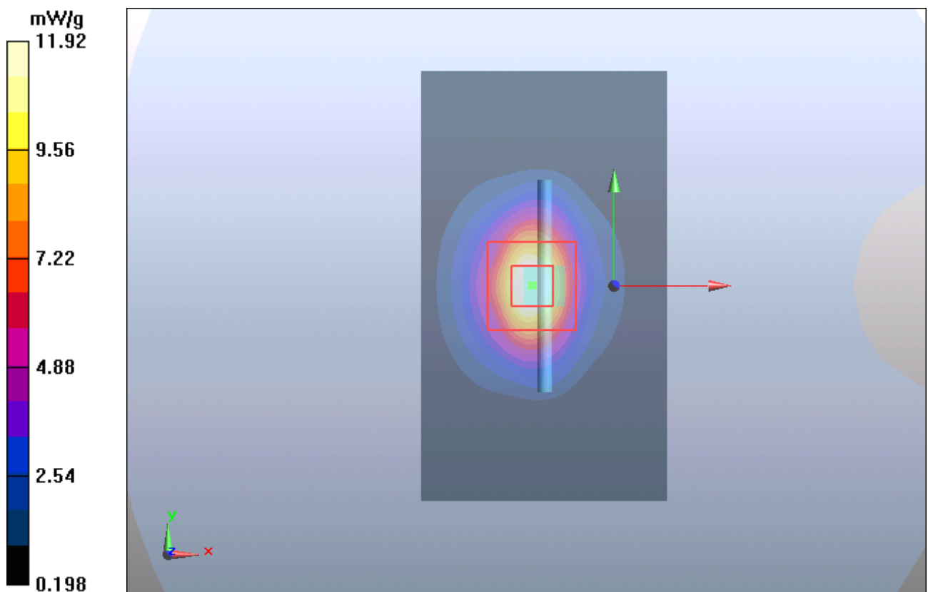
Figure 109 System Performance Check 1900MHz 250mW
