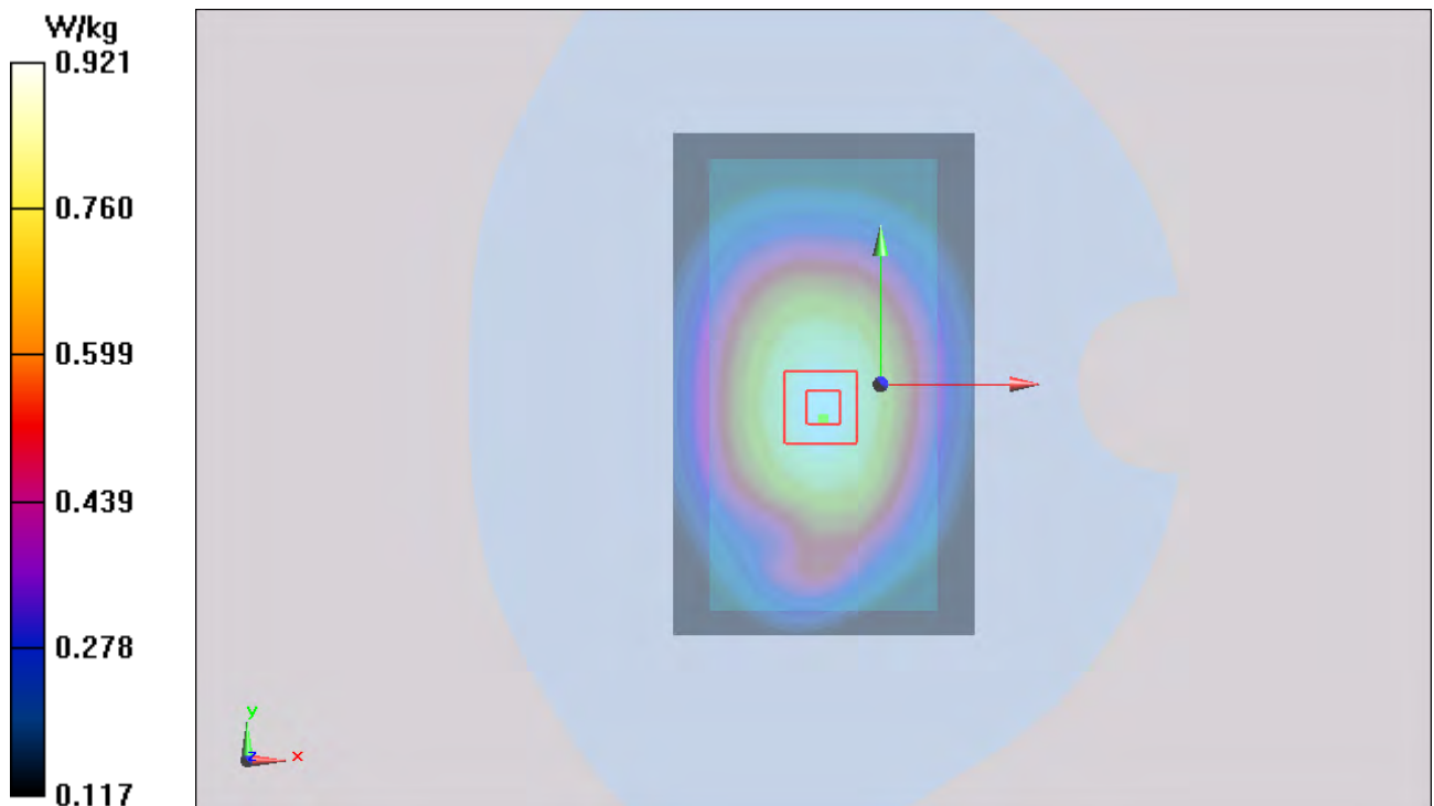
Figure 124 Body, Back Side, UMTS Band V Channel 4183
