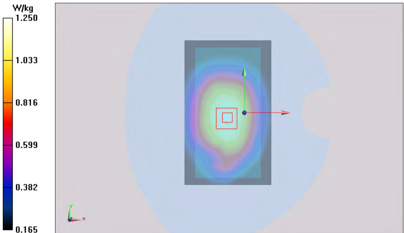
Figure 113 Body, Back Side, GSM 850 GPRS (3Txslots) Channel 251
