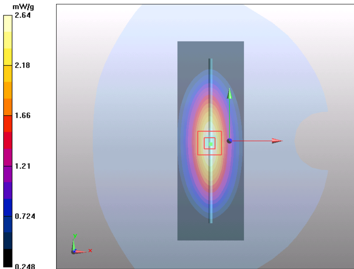
Figure 108 System Performance Check 835MHz 250Mw
