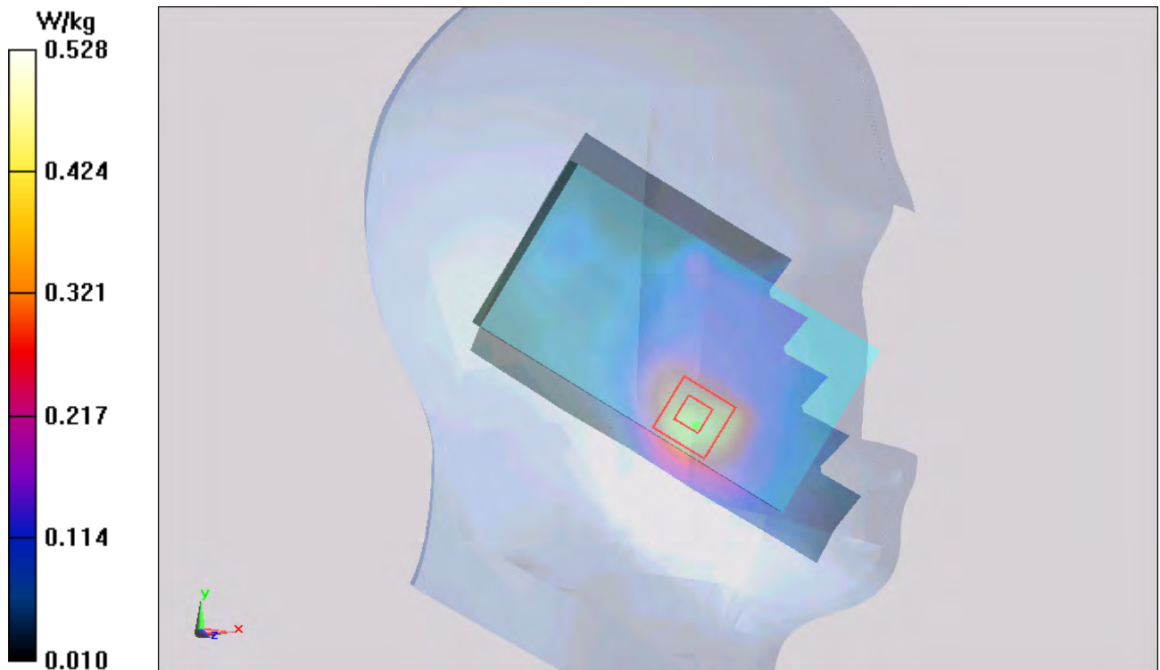
Figure 120 Left Hand Touch Cheek UMTS Band II Channel 9400
