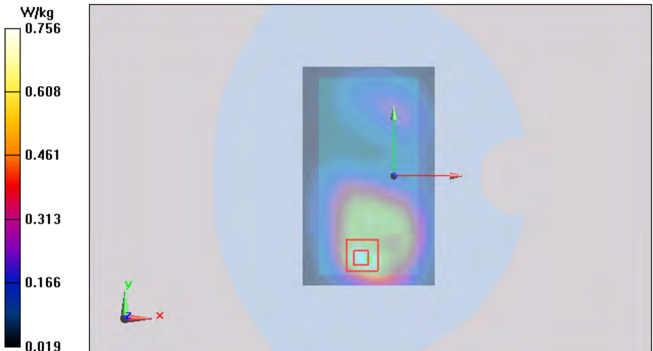
Figure 63 Body, Back Side, UMTS Band II Channel 9538
