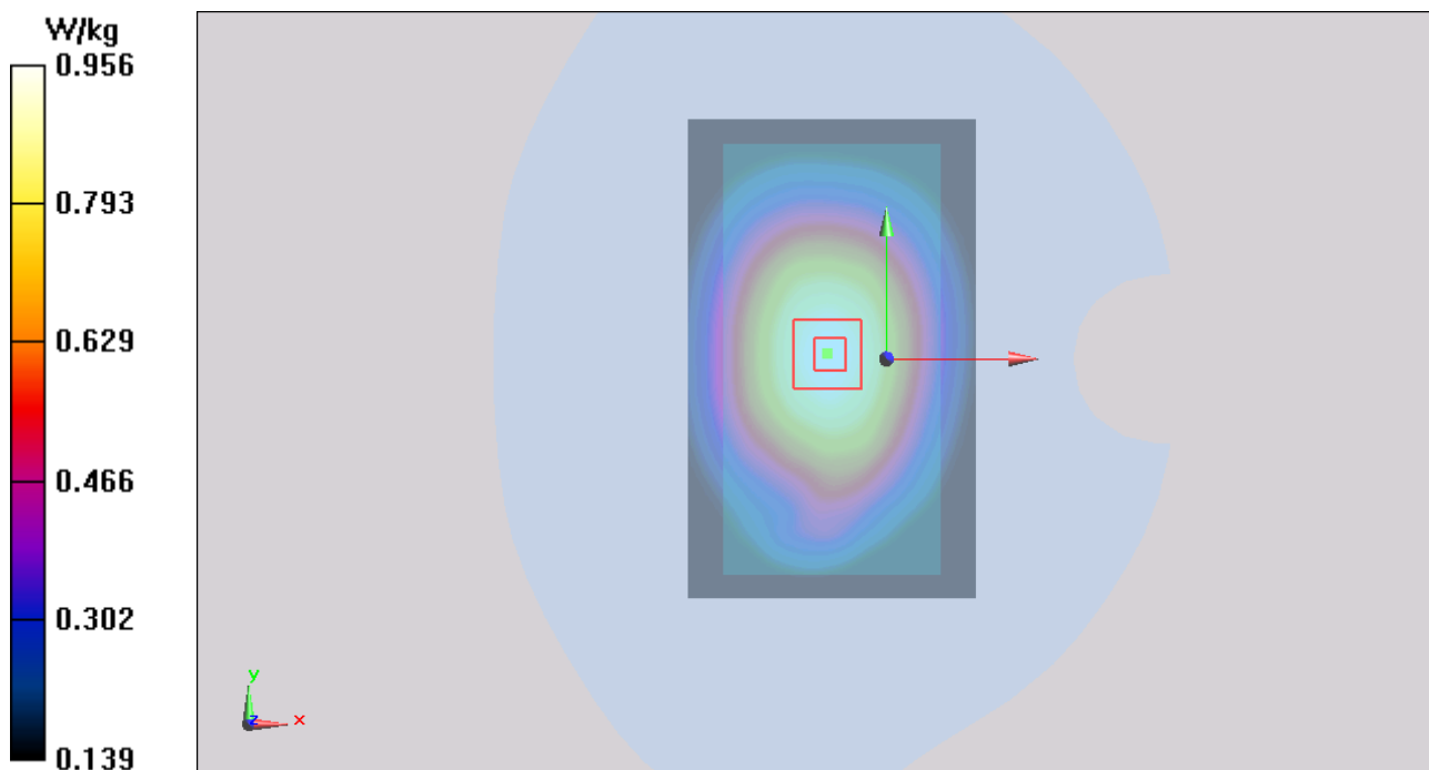
Figure 91 Body, Back Side, UMTS Band V Channel 4233
