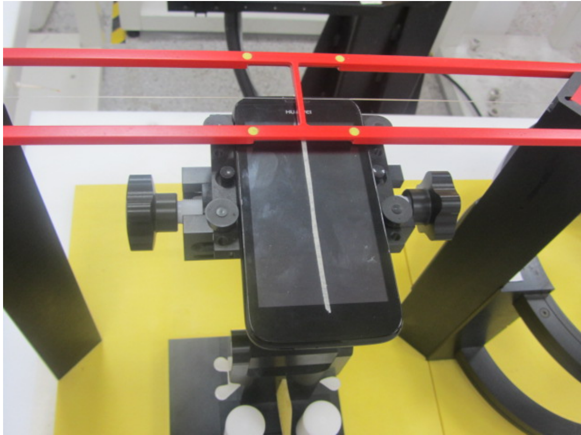
HAC RF test photo
