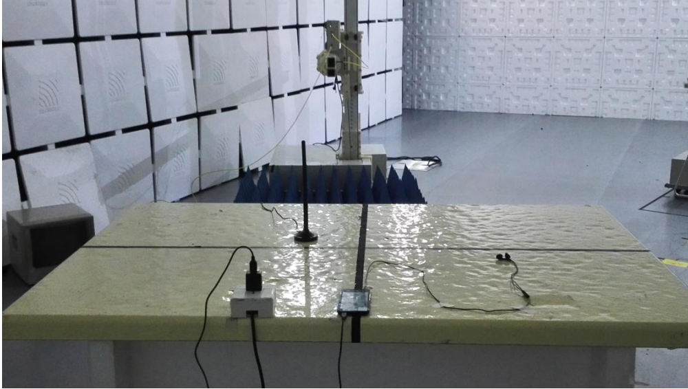
Radiated Spurious Emission (above 18GHz)
