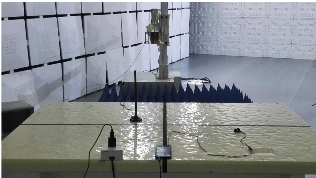
Radiated Spurious Emission (3GHz to18GHz)
