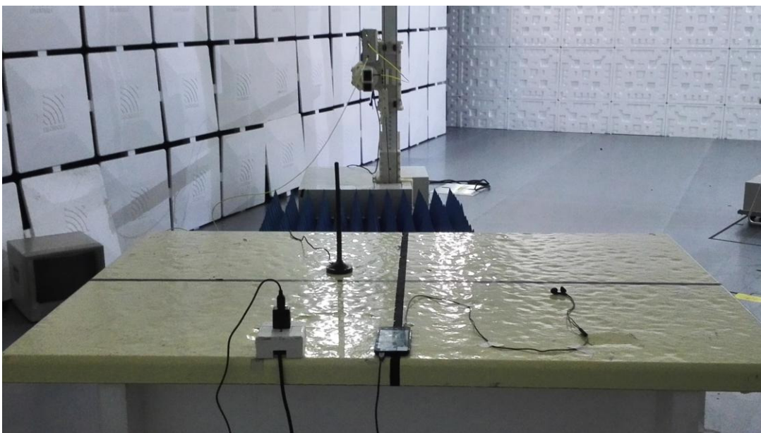
Radiated Spurious Emission (18GHz to26.5GHz)
