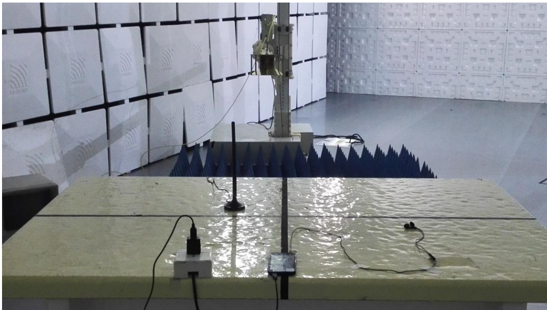
Radiated Spurious Emission (1GHz to18GHz)
