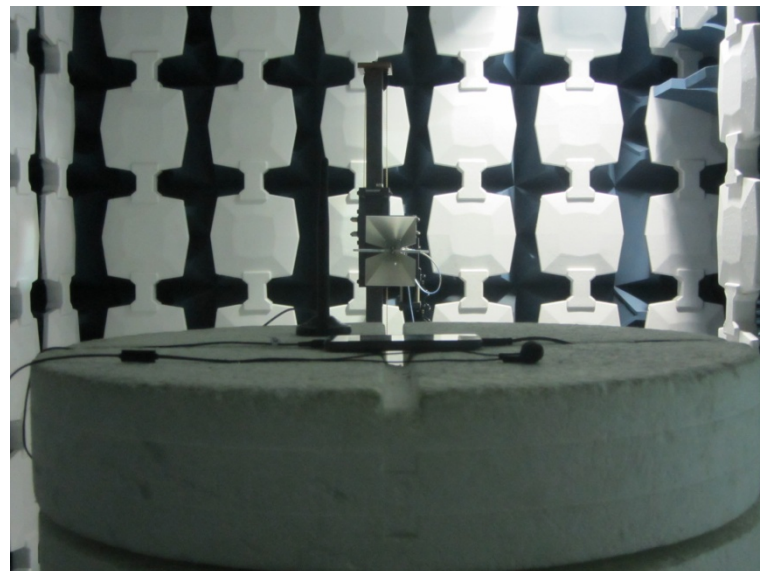
Radiated Spurious Emission (3GHz to18GHz)
