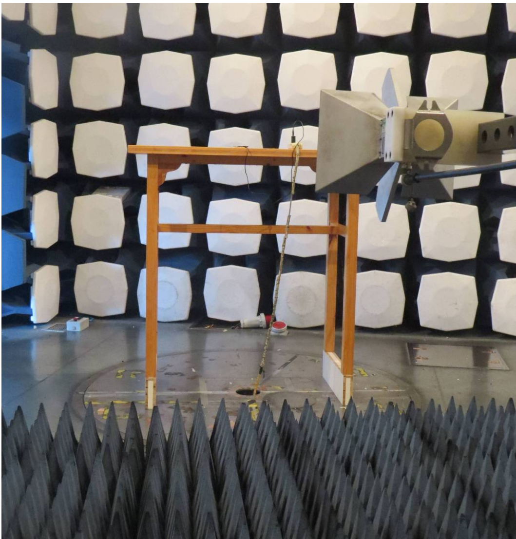
Picture 2 Radiated Emission Test Setup
