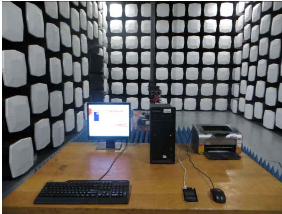
2. Radiated Emissions (Part 15B PC mode)-2
