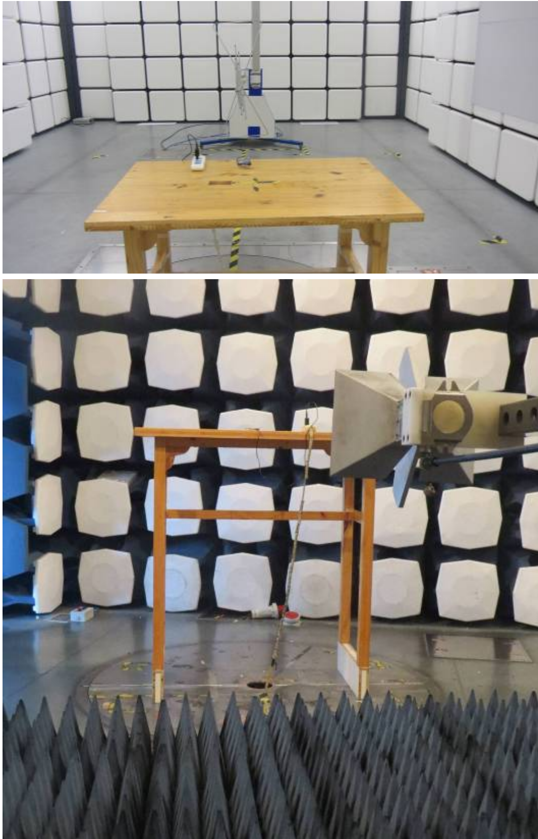
Picture 2 Radiated Emission Test Setup
