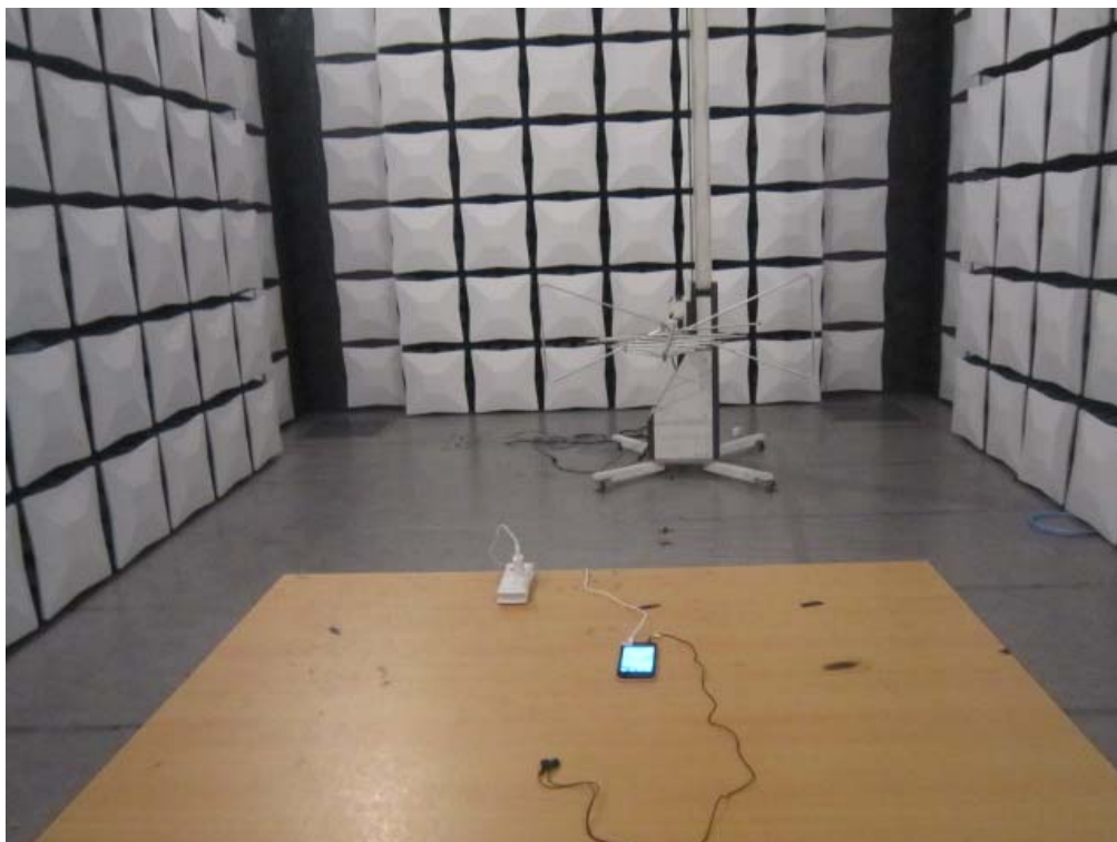
Photo 2 FCC Part 22H/24E Radiated Emission below 1GHz
