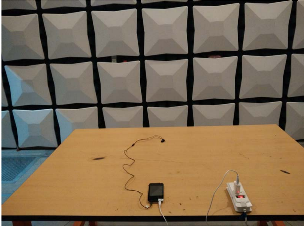
Photo 3 FCC Part 22H/24E Radiated Emission below 1GHz
