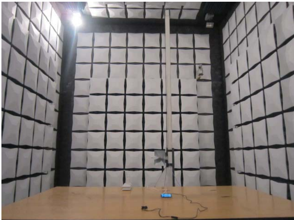
Photo 4 FCC Part 22H/24E Radiated Emission above 1GHz
