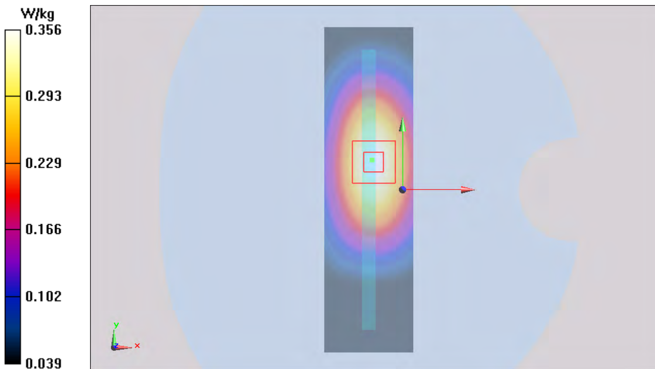
Figure 62 Body, Left Edge, UMTS Band V Channel 4183
