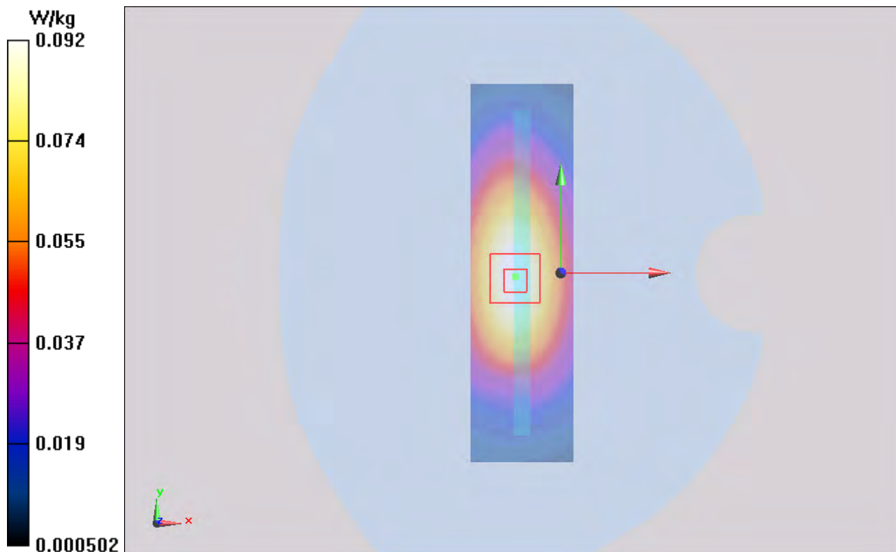
Figure 23 Body, Right Edge, GSM 850 GPRS (3Txslots) Channel 190
