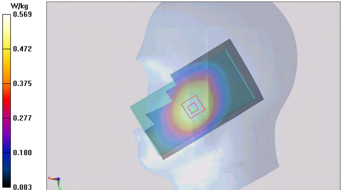
Figure 57 Right Touch Cheek UMTS Band V Channel 4183
