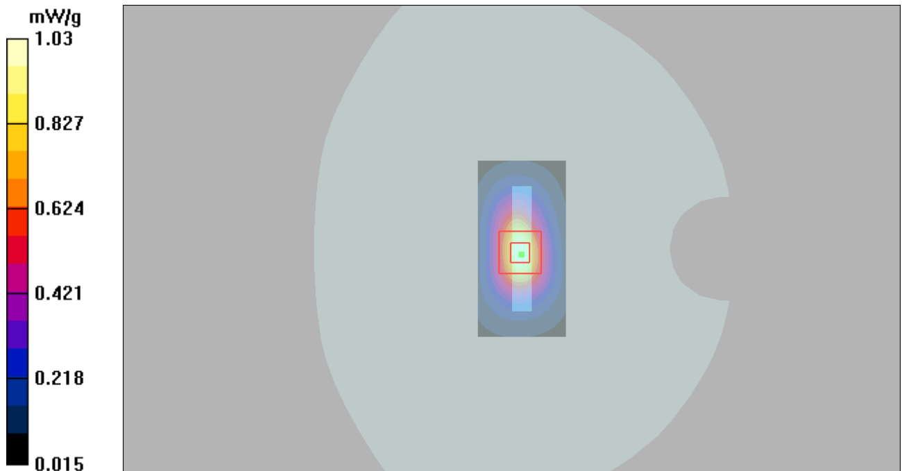
Figure 92 Body, Bottom Edge, UMTS Band II Channel 9538
