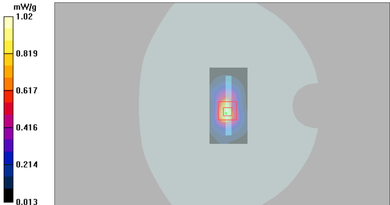
Figure 91 Body, Bottom Edge, UMTS Band II Channel 9538
