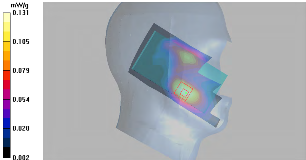
Figure 86 Left Hand Touch Cheek GSM 1900 Channel 661
