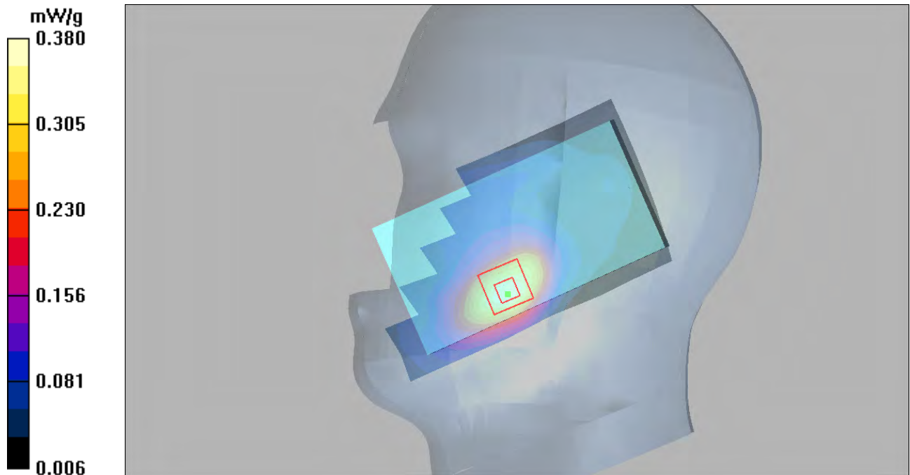
Figure 90 Right Hand Touch Cheek UMTS Band II Channel 9400
