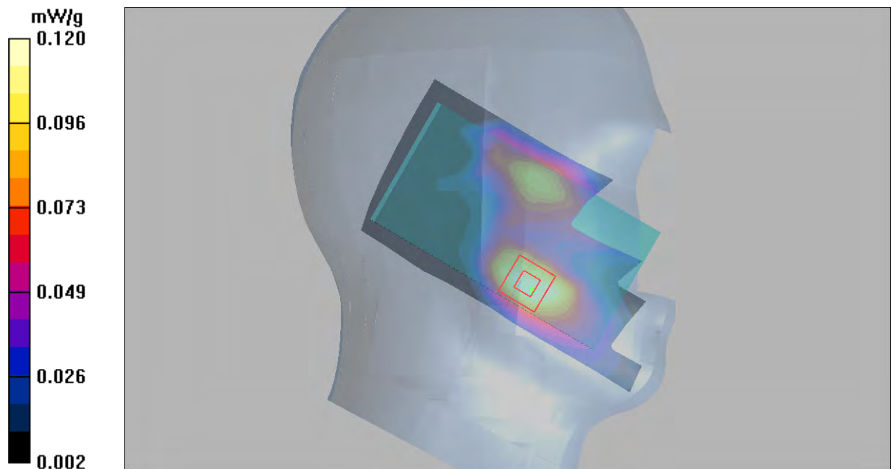
Figure 87 Left Hand Touch Cheek GSM 1900 Channel 661
