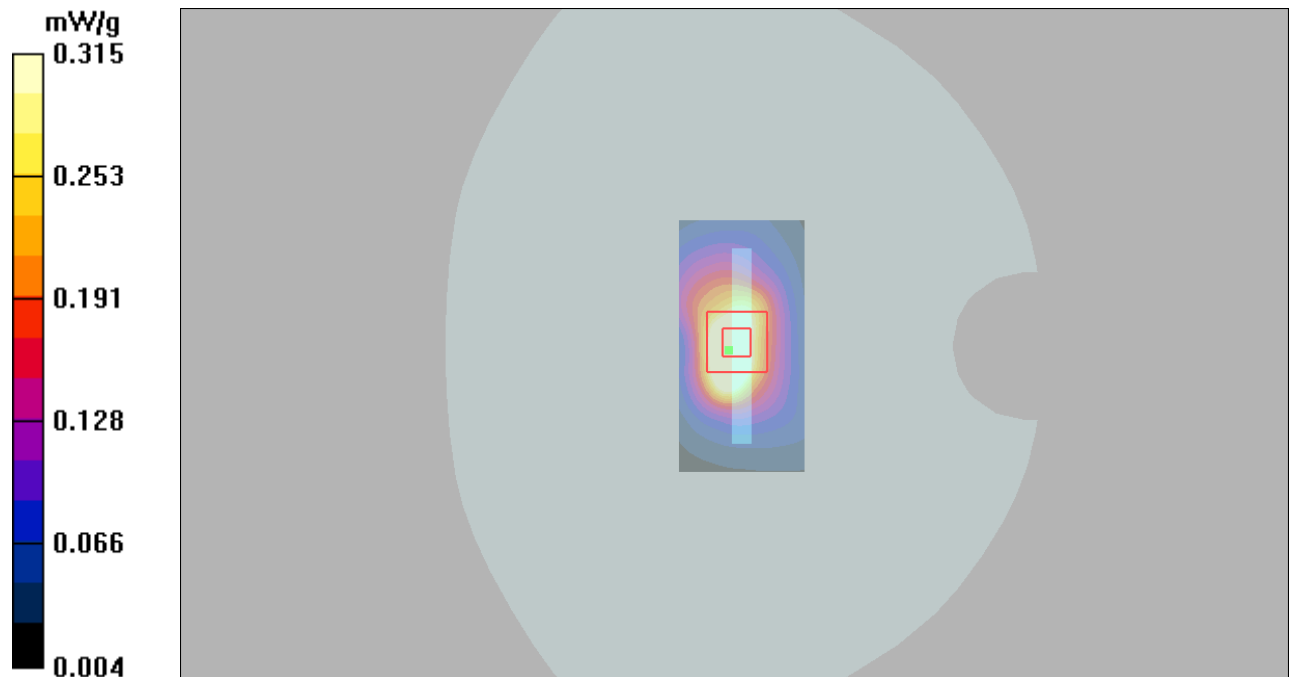
Figure 88 Body, Bottom Edge, GSM 1900 GPRS (4Txslots) Channel 661
