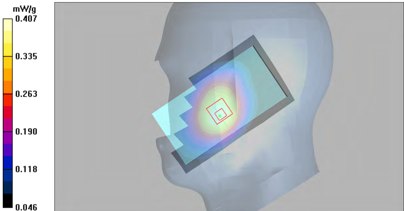
Figure 93 Right Hand Touch Cheek UMTS Band V Channel 4183
