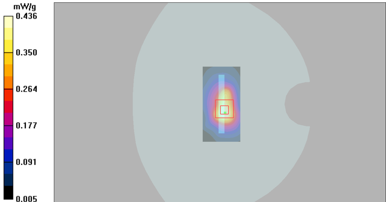
Figure 89 Body, Bottom Edge, GSM 1900 GPRS (4Txslots) Channel 661
