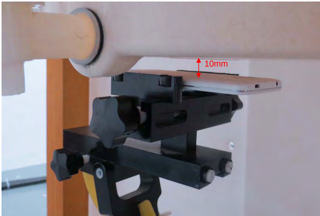
Picture 21: Back Side, the distance from handset to the bottom of the Phantom is 10mm (Variant Model)
