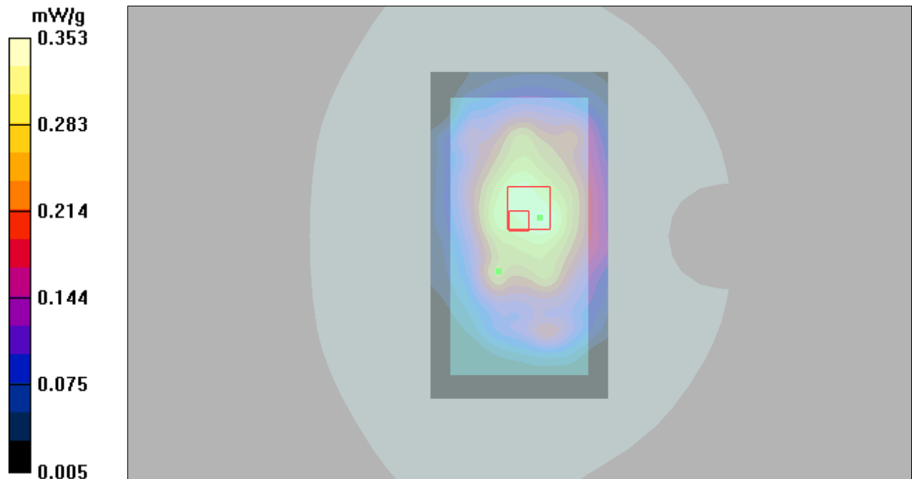
Figure 85 Body, Back Side, GSM 850 GPRS (3Txslots) Channel 190
