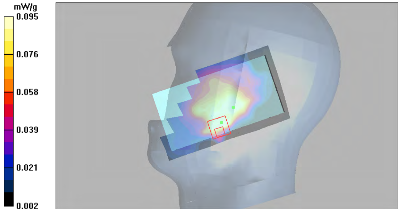
Figure 83 Right Hand Touch Cheek GSM 850 Channel 190
