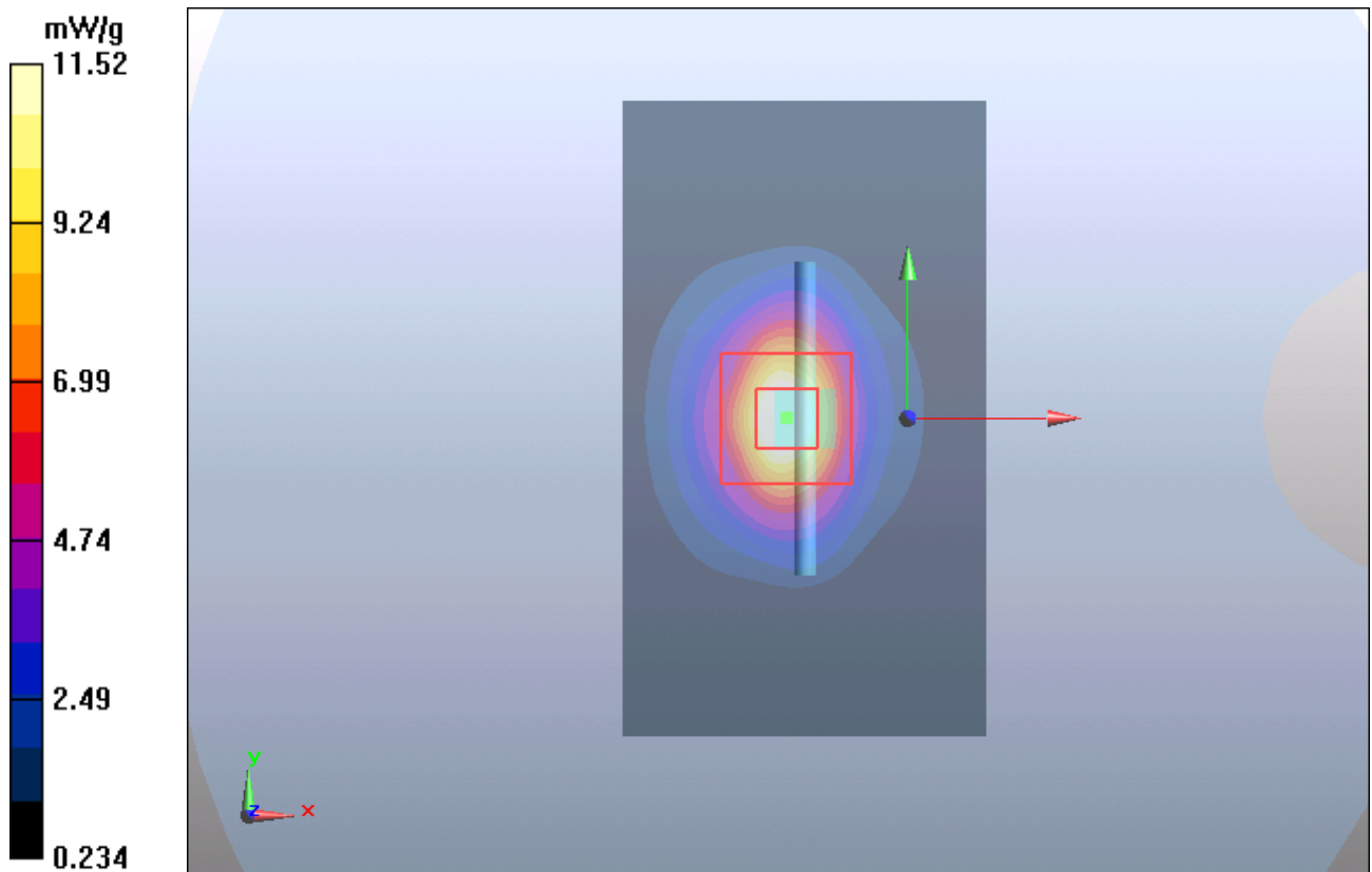
Figure 81 System Performance Check 1900MHz 250mW
