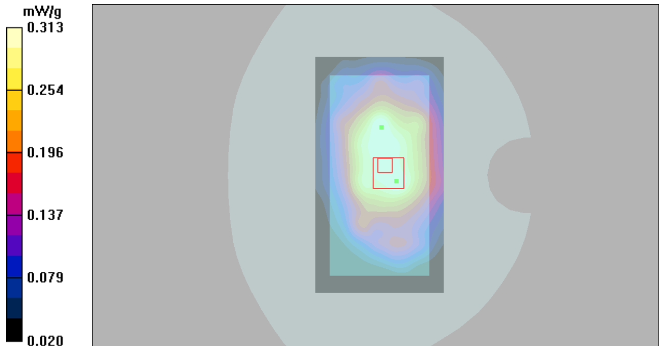
Figure 84 Body, Back Side, GSM 850 GPRS (3Txslots) Channel 190
