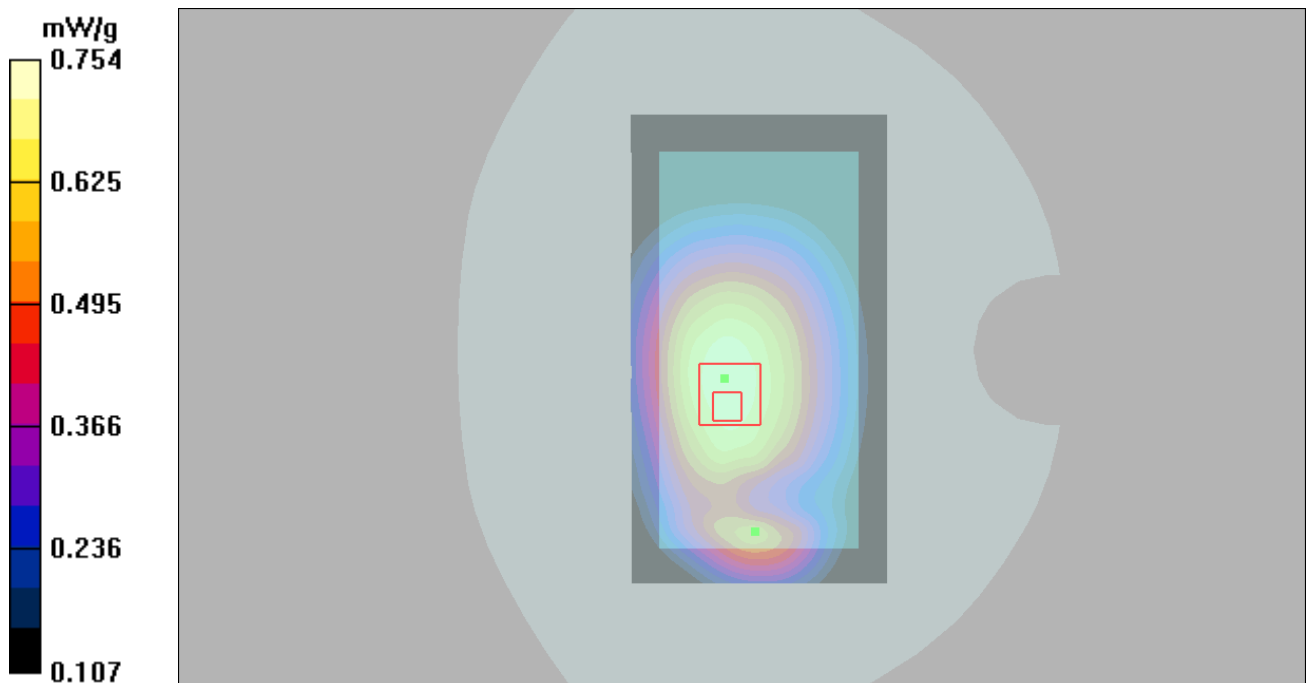
Figure 94 Body, Back Side, UMTS Band V Channel 4233
