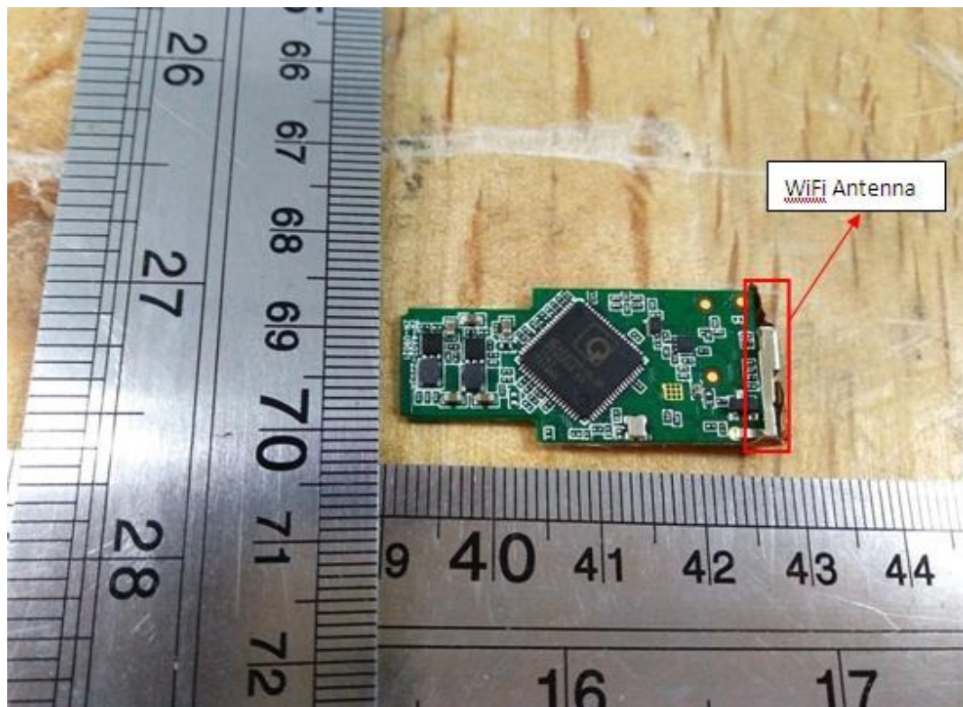
Fig. 3 Position of the antennas
