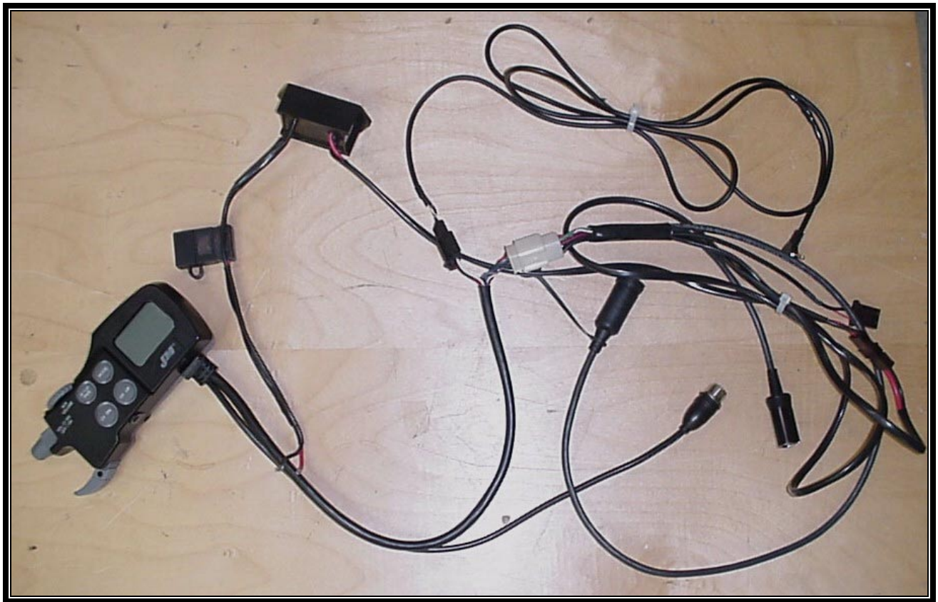
PHOTOGRAPH 10: EUT WITH ASSOCIATED CABLING
