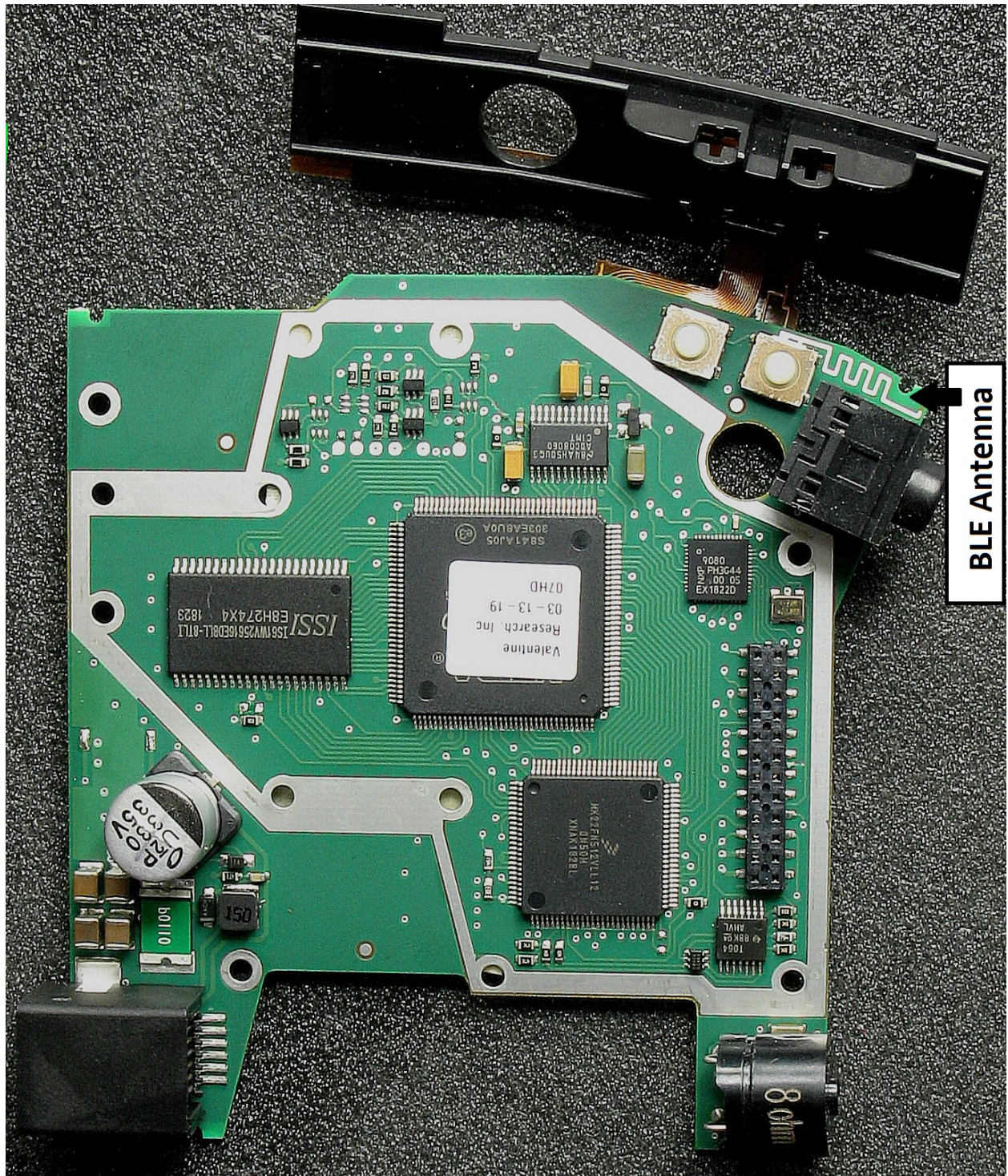
PHOTO SHOWING BT ANTENNA LOCATION
