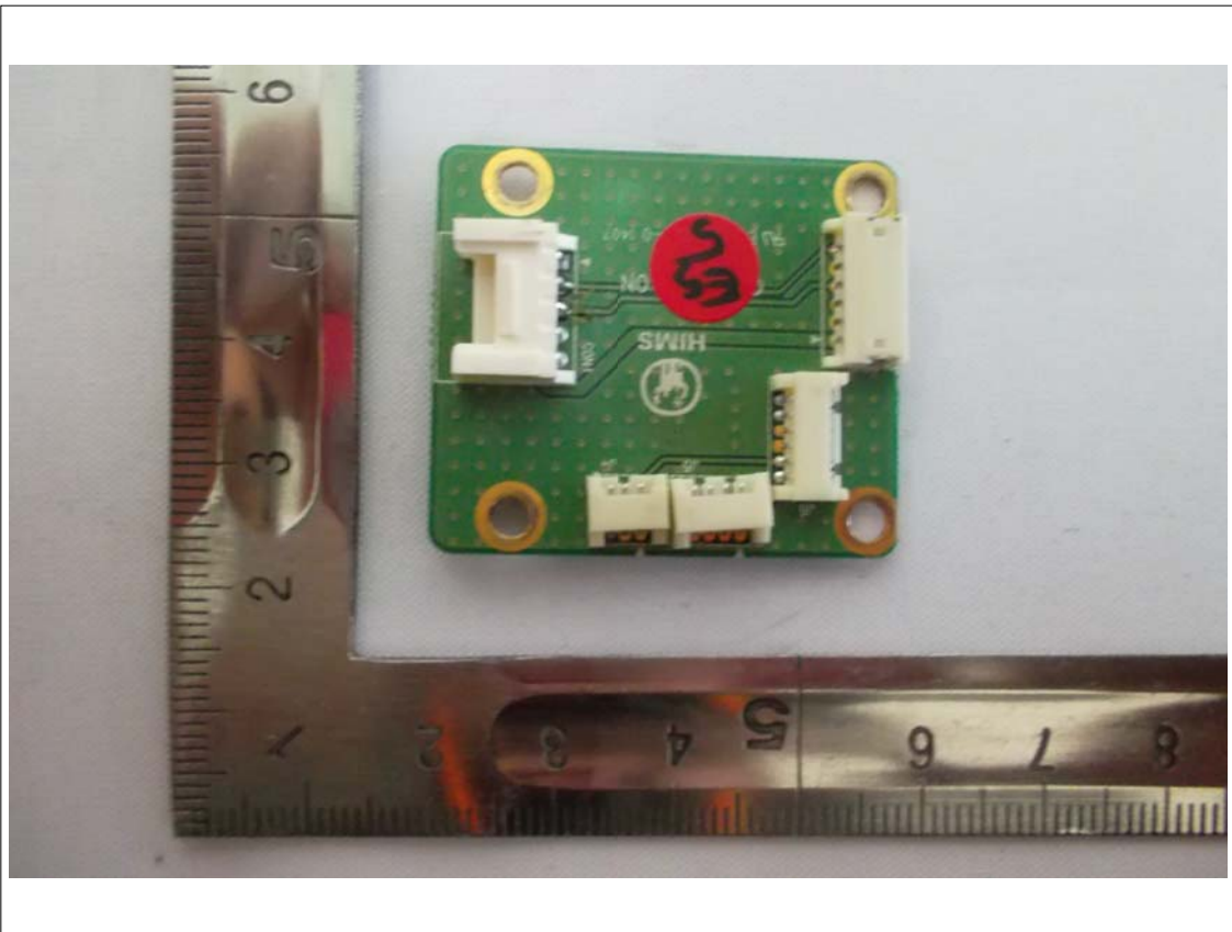
View of Sub PCB 8(Top)
