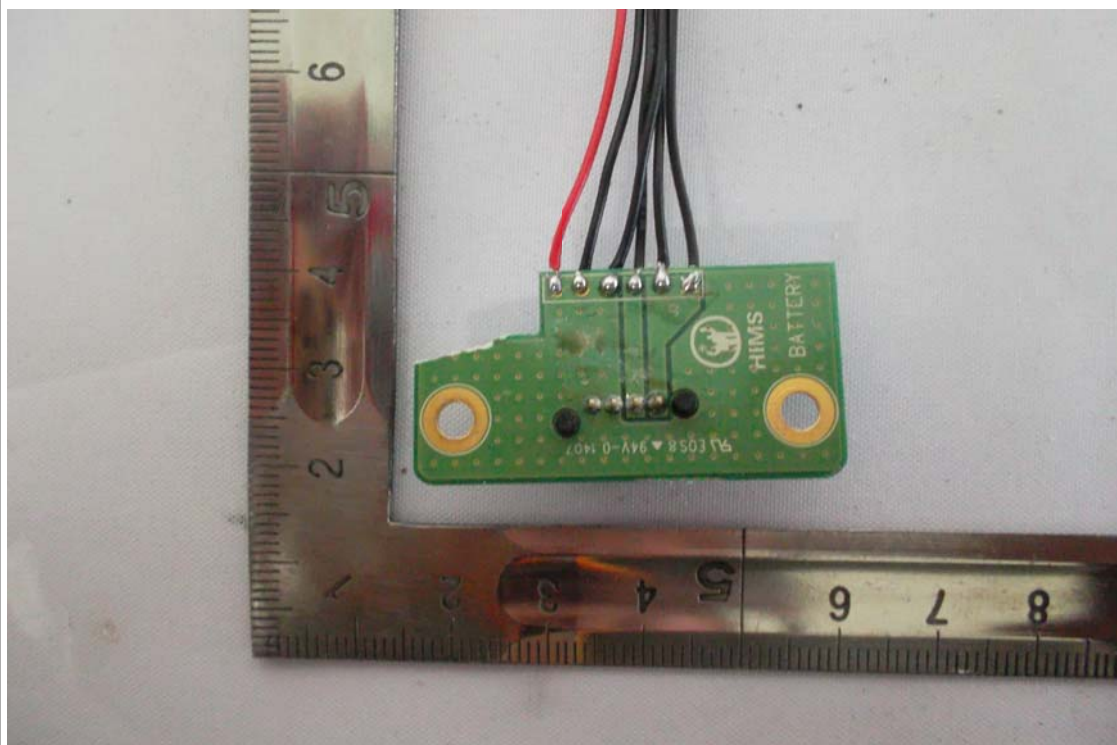
View of Sub PCB 3(Bottom)-BATTERY CONNECTOR
