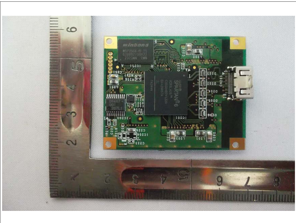
View of Sub PCB 5(Bottom)-CAMERA
