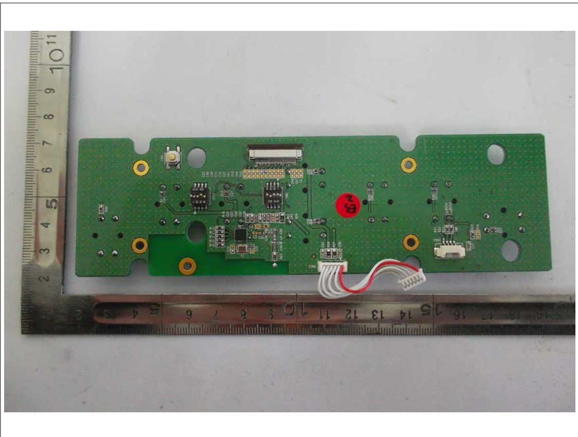
View of Sub PCB 1(Bottom)
