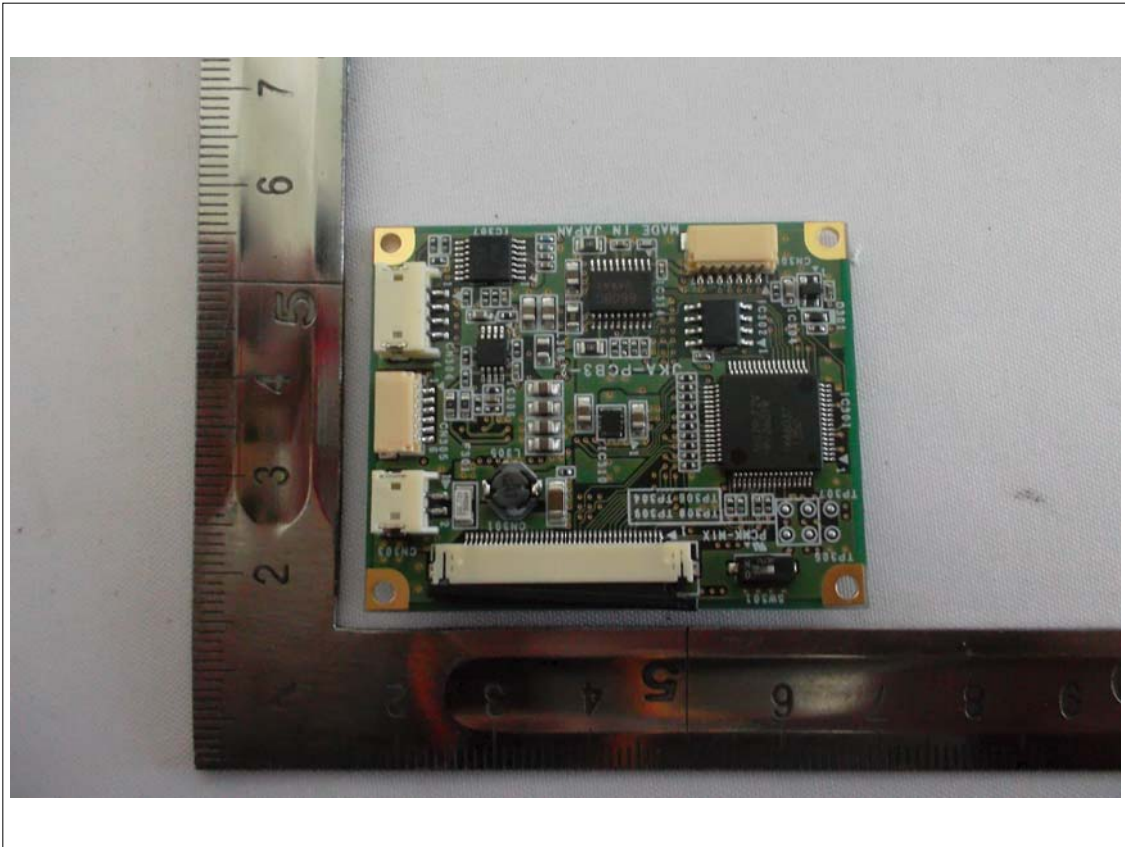
View of Sub PCB 6(Top)_CAMERA
