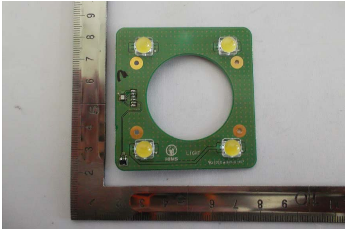
View of Sub PCB 4(Top)_CAMERA LED
