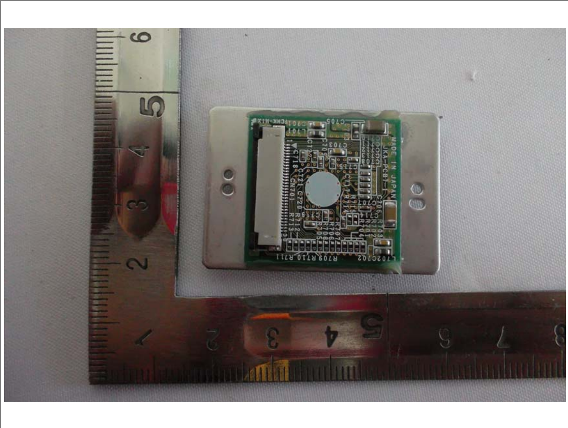
View of Sub PCB 7(Top)_CAMERA
