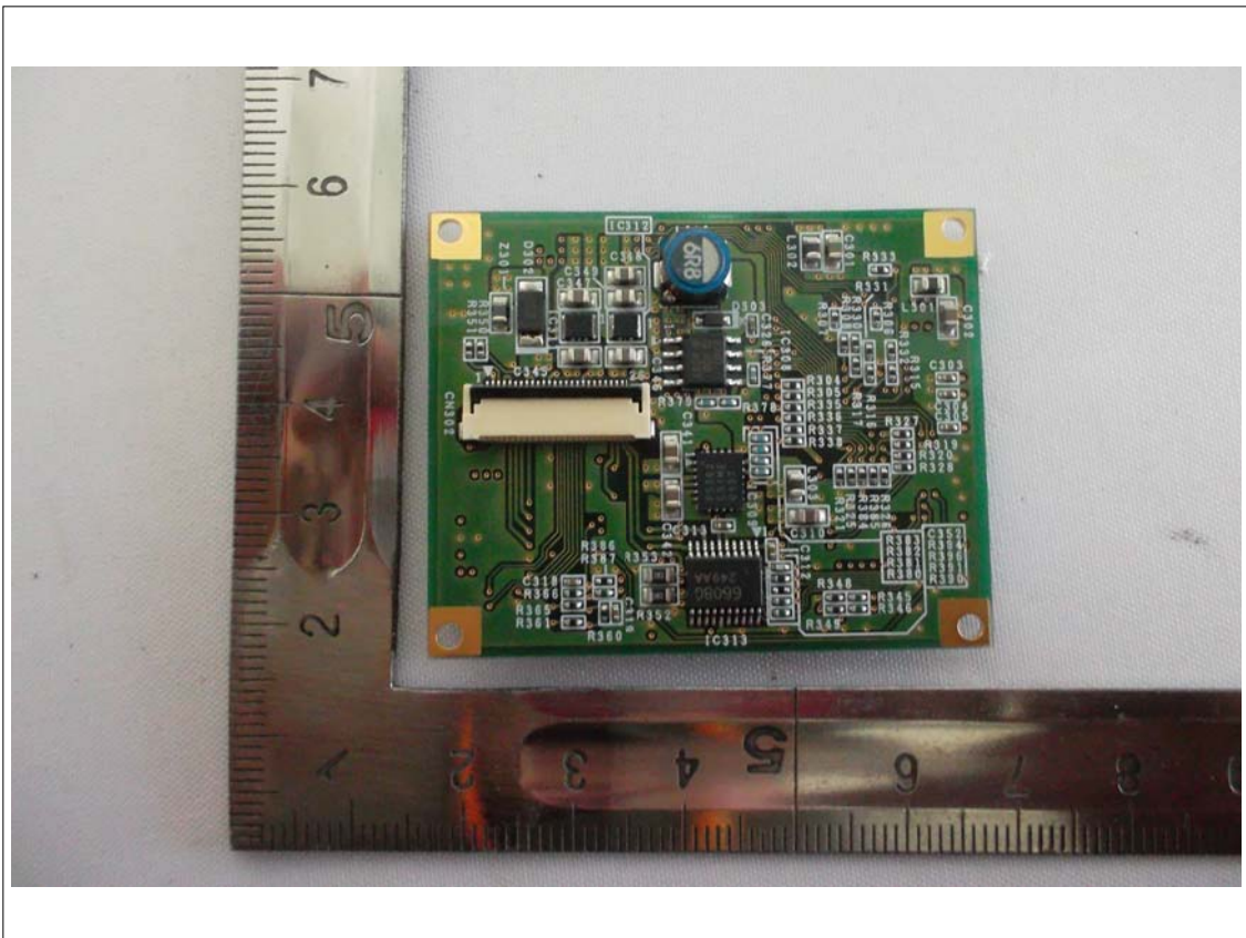
View of Sub PCB 6(Bottom)_CAMERA
