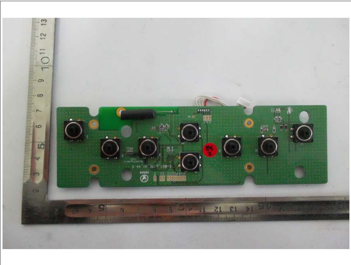
View of Sub PCB 1(Top)
