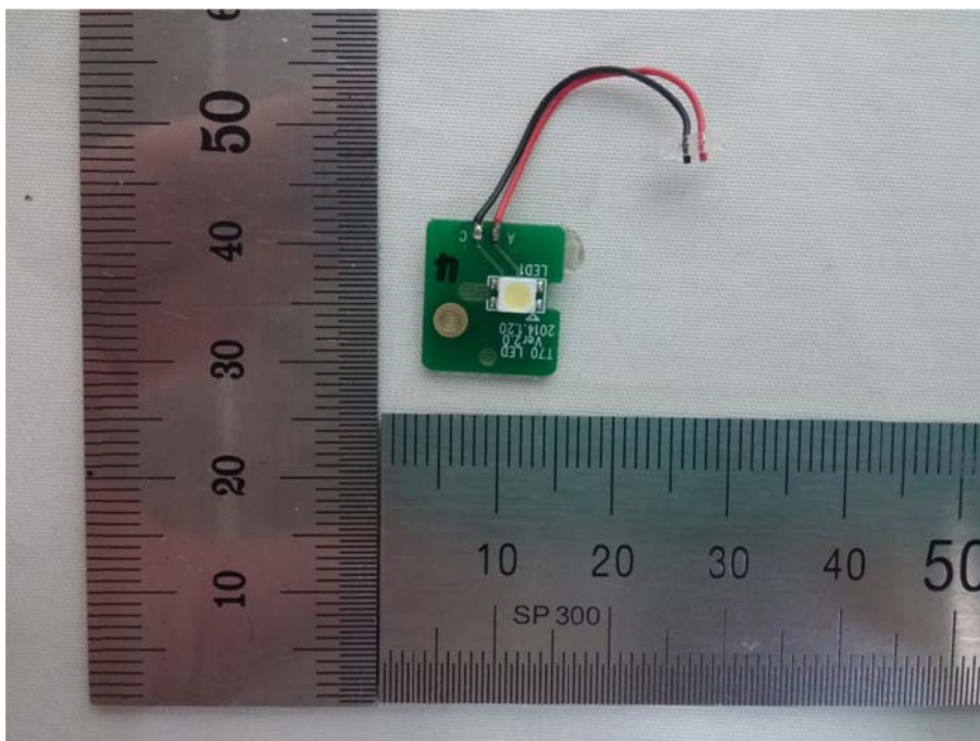
View of LED Board (TOP)
