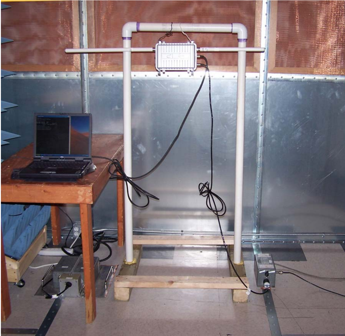
Photograph 2: Conducted Emissions Voltage Test Setup
