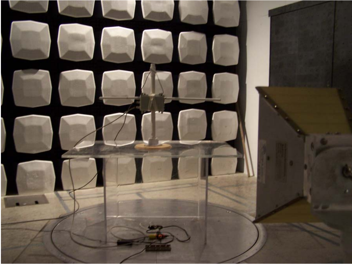
Photograph 3: Band Edge Restricted Test Setup
