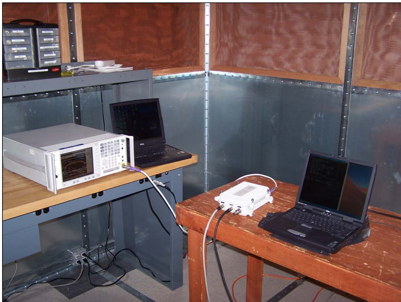
Photograph 4. Peak Power Output and RF Exposure, Test Setup
