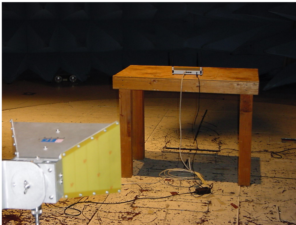
Photograph 5. Test Equipment and setup for various Radiated Measurements
