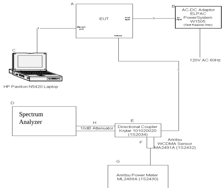
Figure 2. Block Diagram of Test Configuration (Conducted Measurement)
