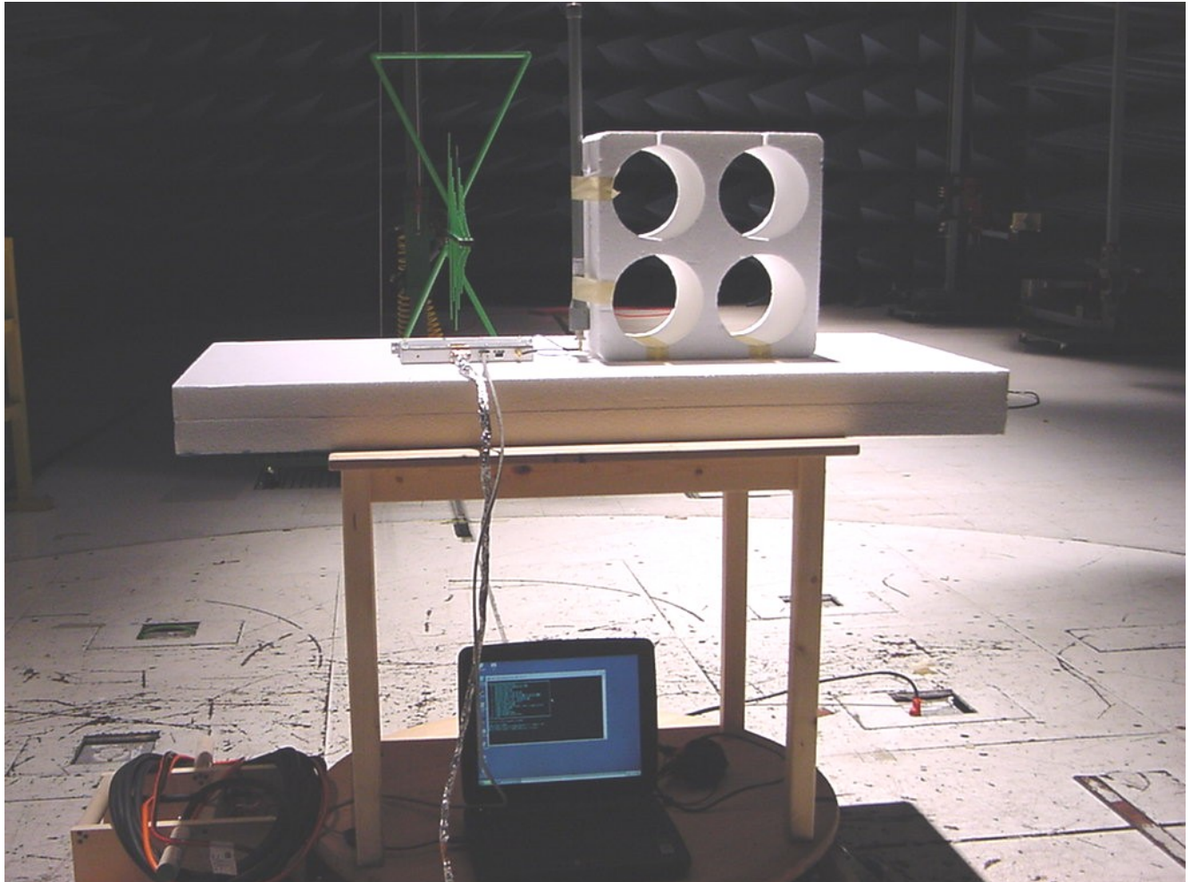
Photograph 2. Radiated Emission Limits (Below 1 GHz), Test Setup
