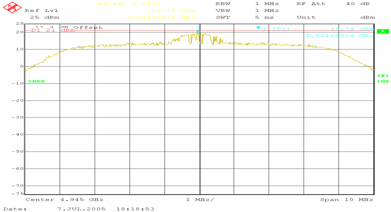
Plot 1. PPSP at Low Channel
