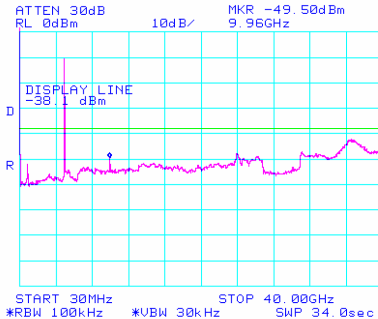
Plot 9. Conducted Spurious Emission at High Channel
