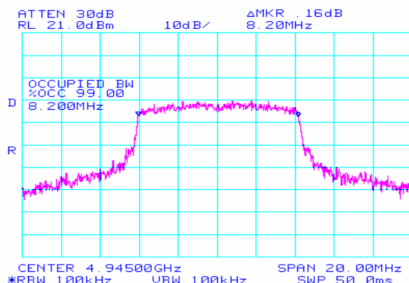
Plot 10. Measured Occupied Bandwidth
