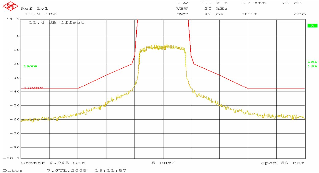
Plot 4. Emission Mask at Low Channel
