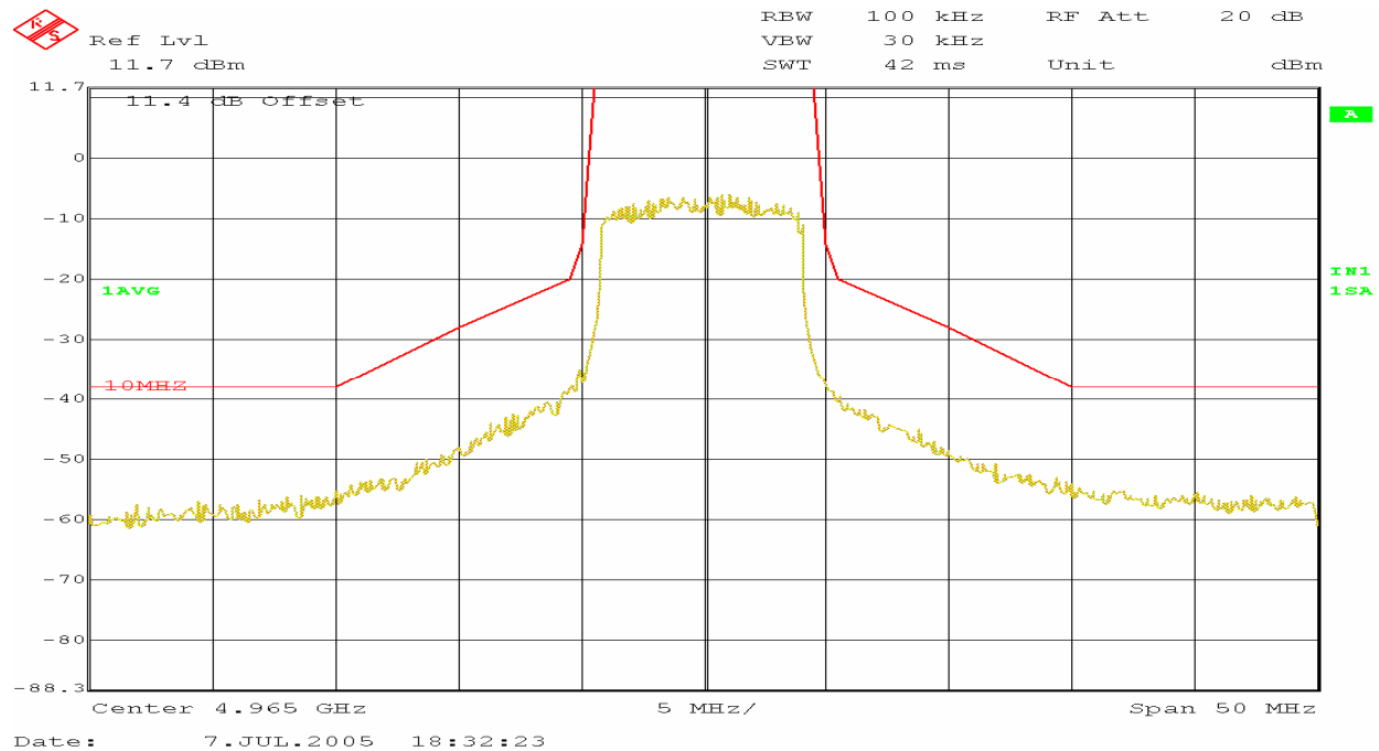
Plot 5. Emission Mask at Mid Channel
