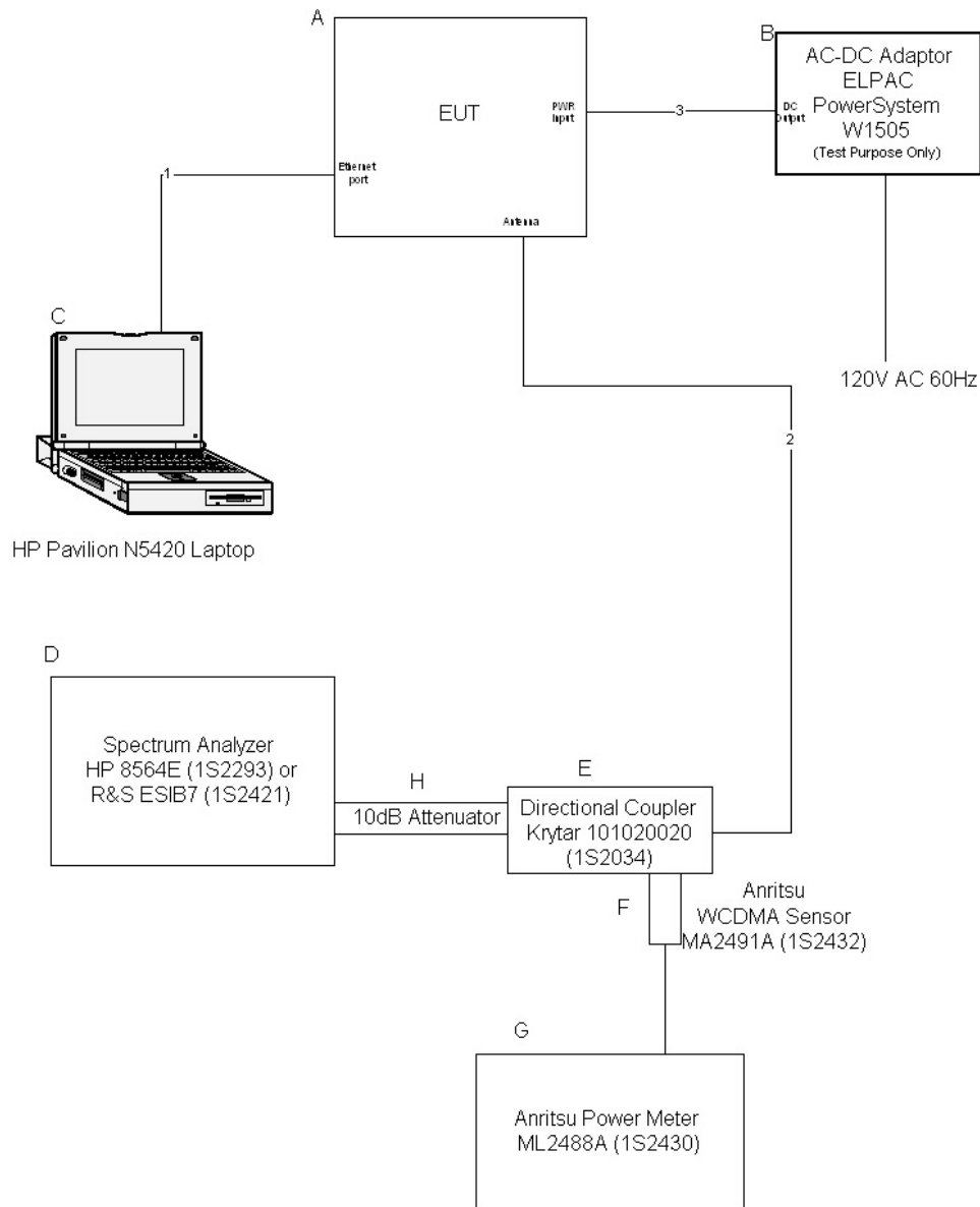
Figure 1. Block Diagram of Test Configuration (Conducted Measurements)
