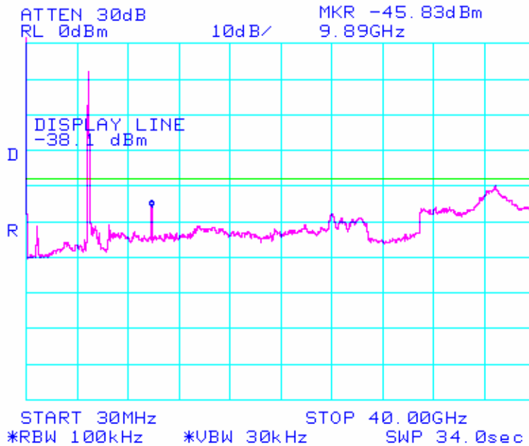
Plot 7. Conducted Spurious Emission at Low Channel
