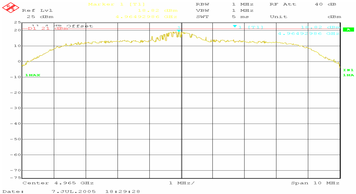
Plot 2. PPSP at Mid Channel
