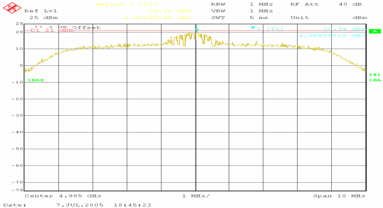
Plot 3. PPSD at High Channel
