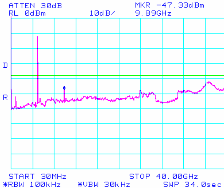
Plot 8. Conducted Spurious Emission at Mid Channel
