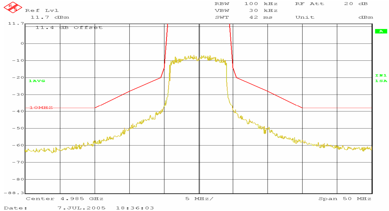
Plot 6. Emission Mask at High Channel
