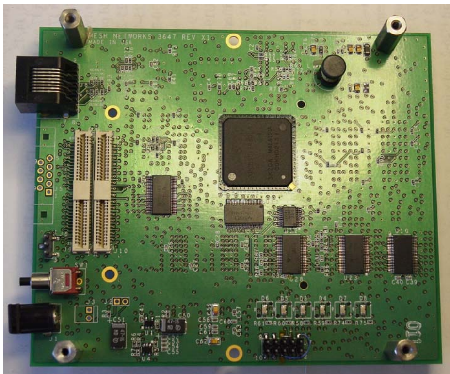
IAP6300 Single Board Computer Top Side
