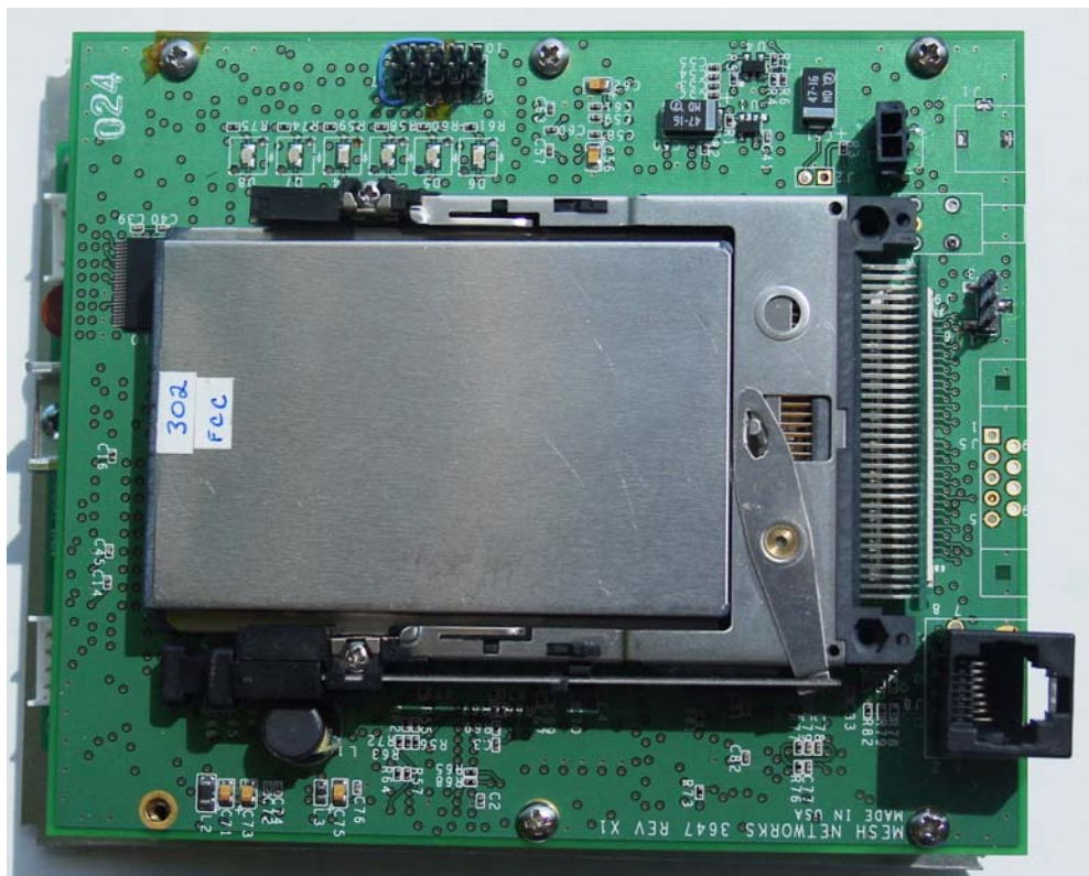
IAP6300 Single Board Computer Top Side with PCMCIA card
