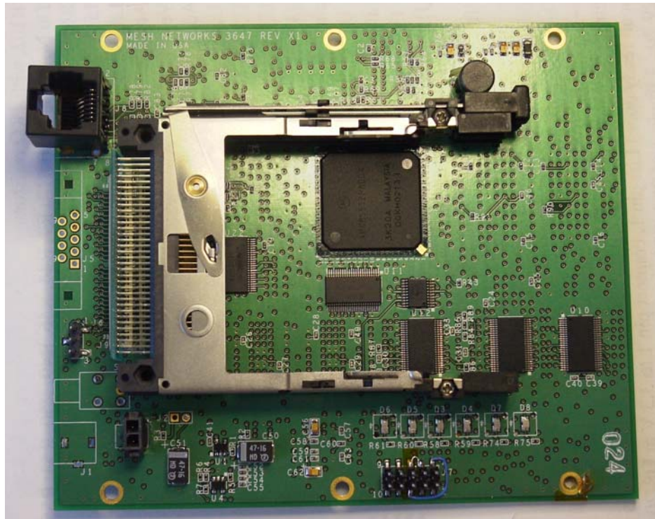
IAP6300 Single Board Computer Top Side with PCMCIA sled
