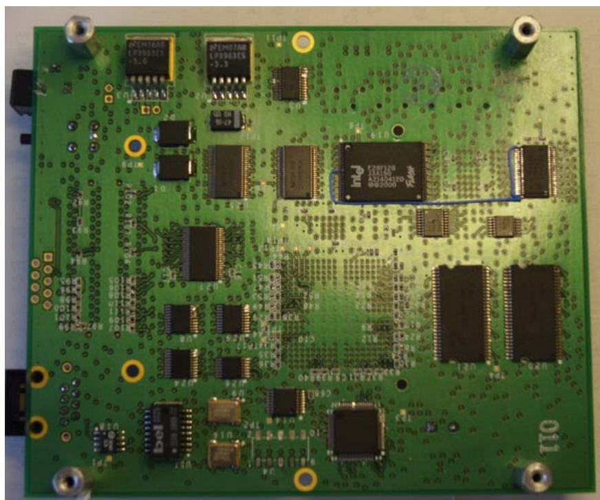
IAP6300 Single Board Computer Bottom Side
