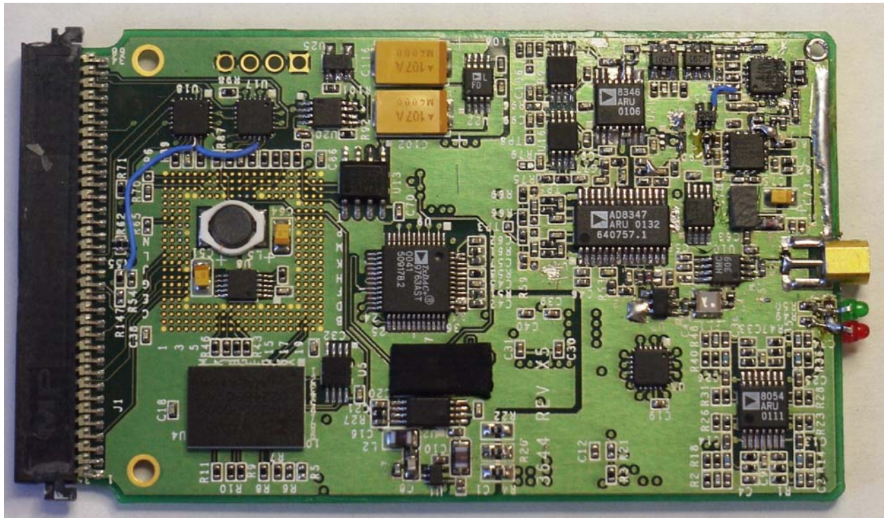
IAP6300 PCMCIA Bottom Side
